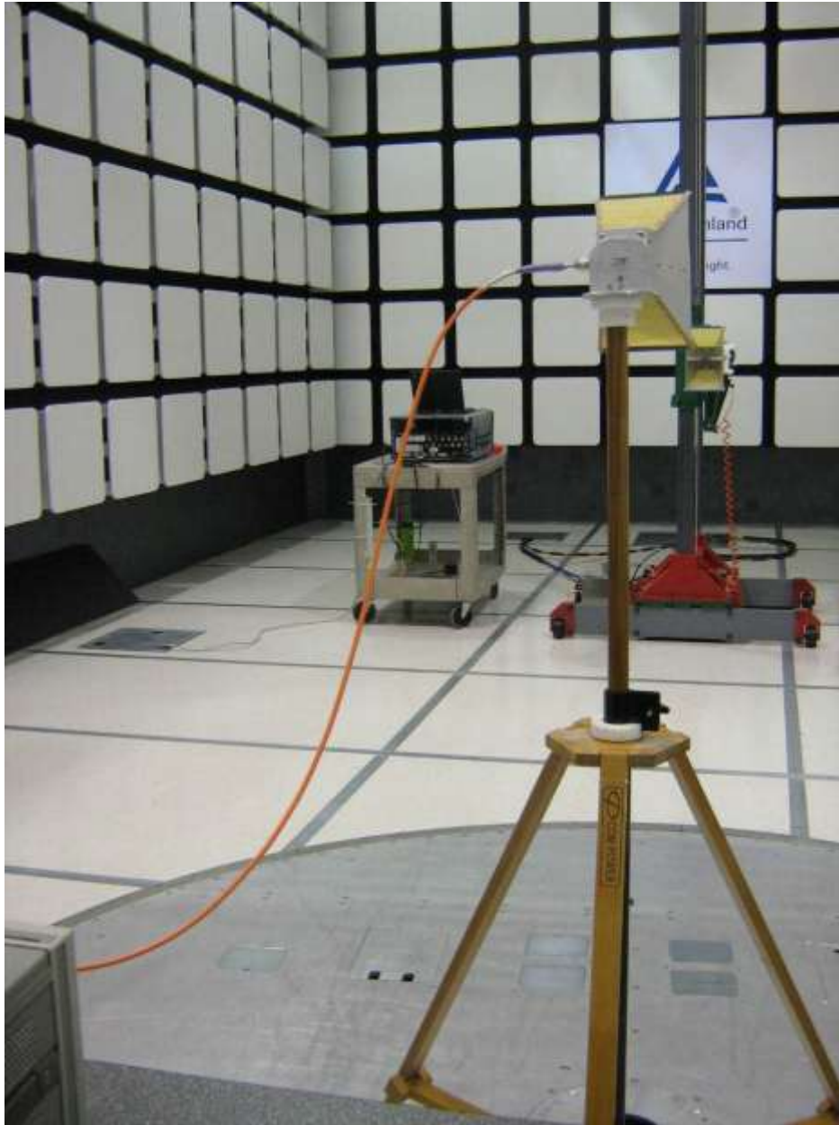
Photo of Test Setup for 1 GHz to 2.5 GHz Substitution
