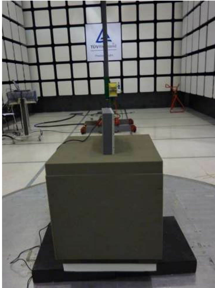
Test Setup – Radiated Emissions
