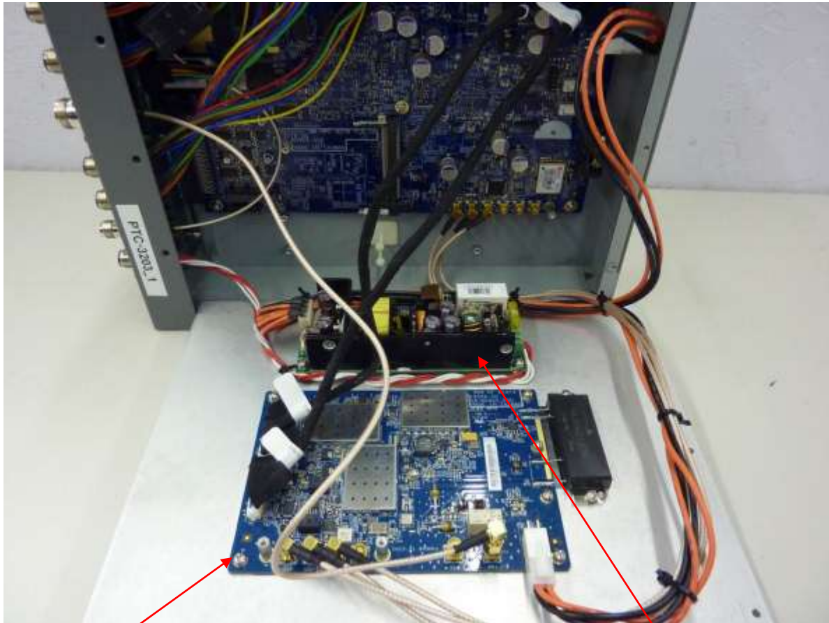
PTC Board
