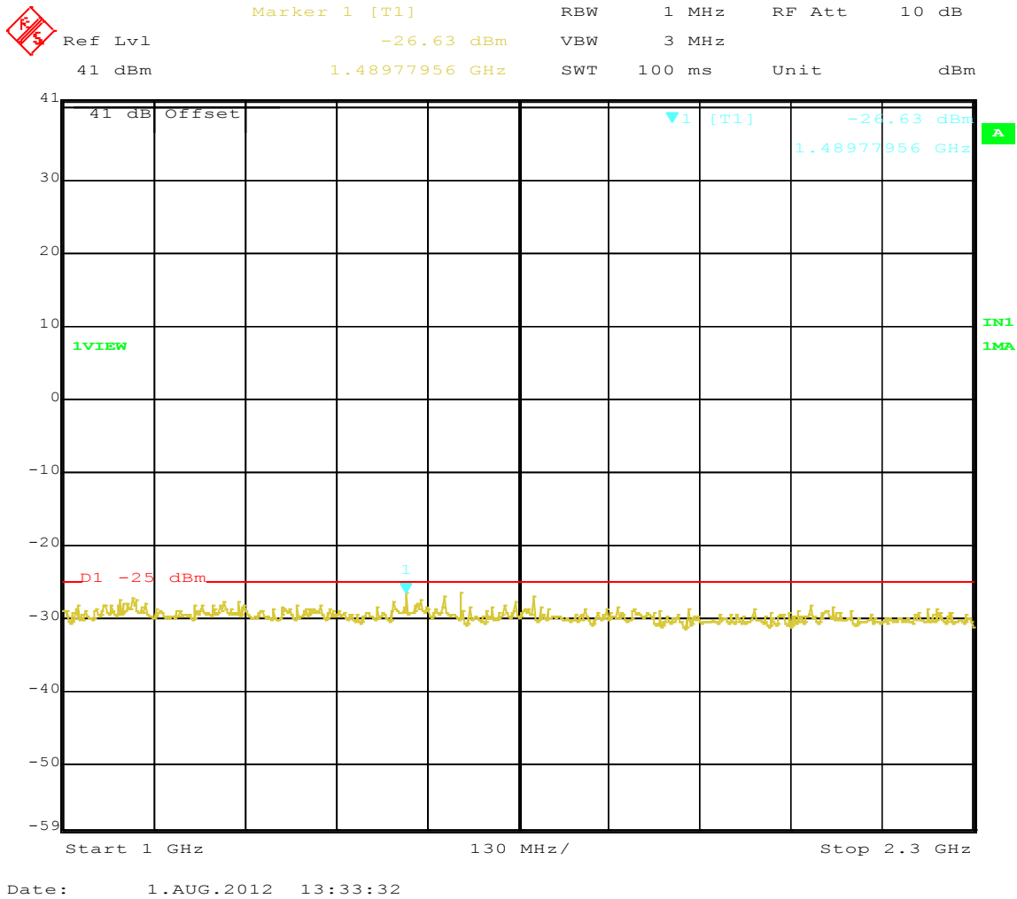
Figure 94: Out of Band Emissions Operating 219.5 MHz 16 QPSK Plot 2
