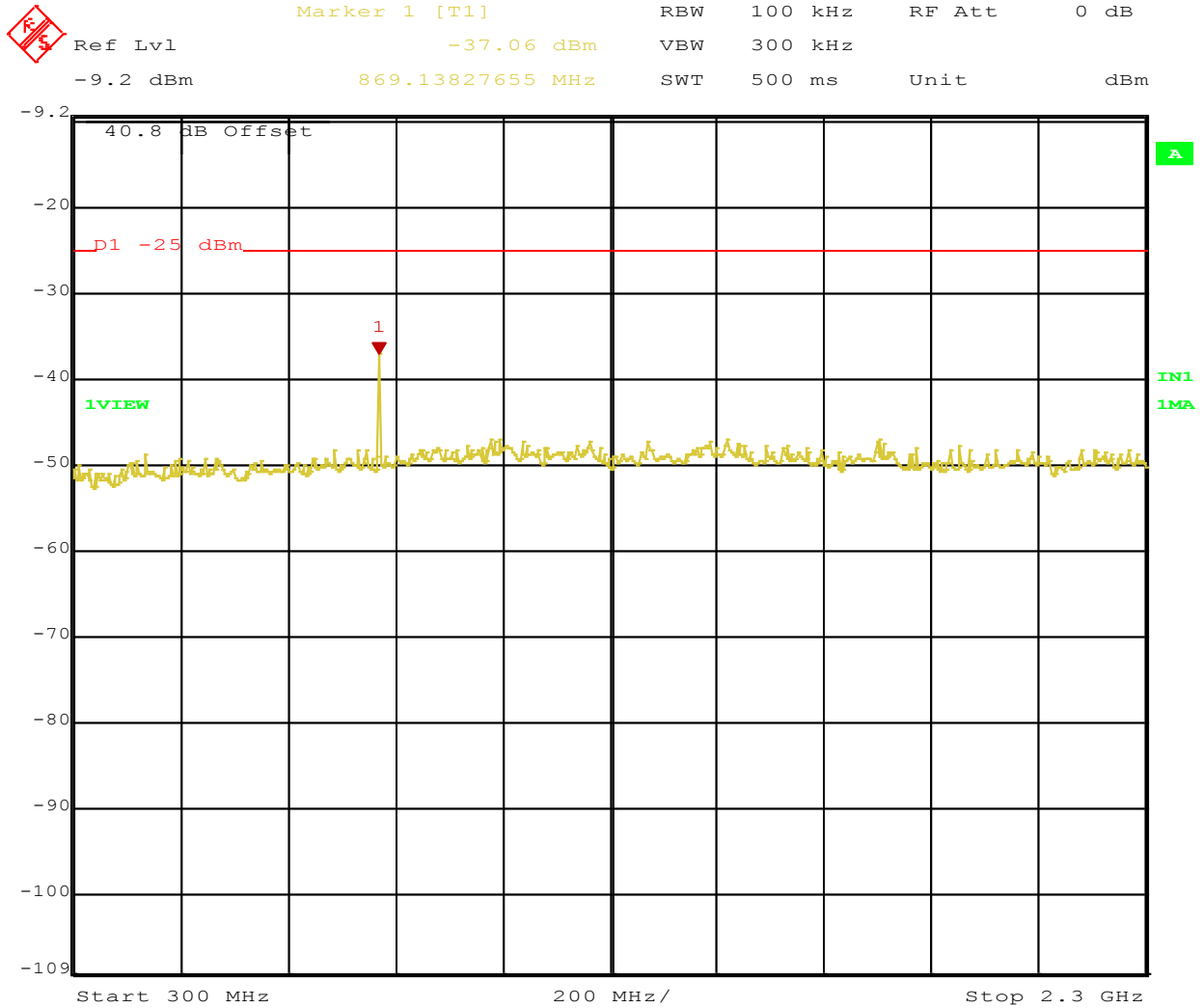
Figure 68: Out of Band Emissions Operating Channel 217.5 MHz, 32 QPSK Plot 2
