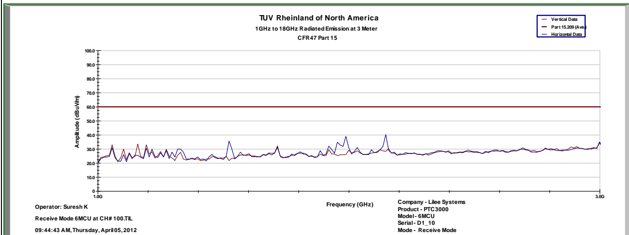
Above 1GHz Plot for Receive Mode
