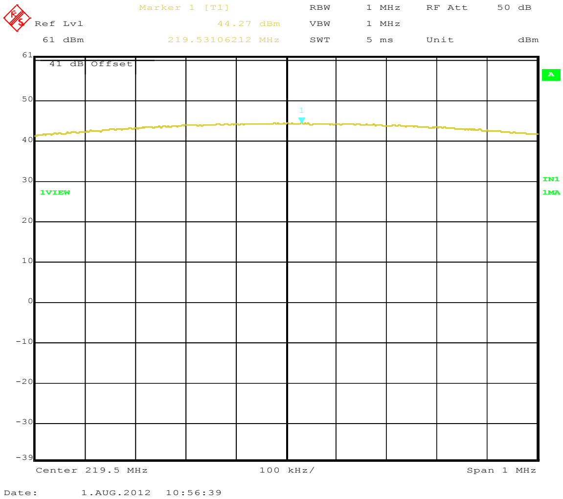
Figure 28: Maximum Transmitted Power, 219.5 MHz at 32 QPSK Power for mobile application
