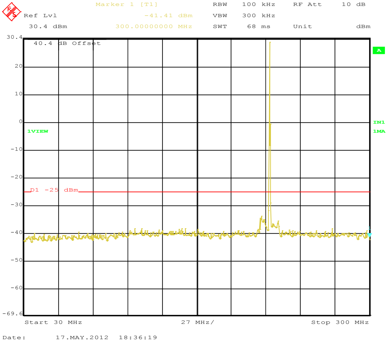
Figure 87: Out of Band Emissions Operating 222 MHz GSM Plot 1
