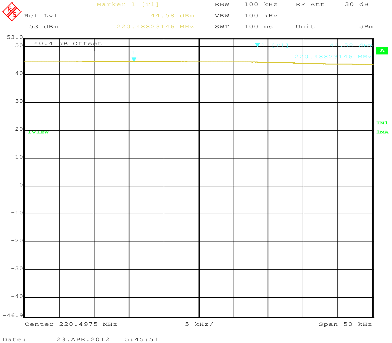
Figure 13: Maximum Transmitted Power, 220.4875 MHz at GMSK
