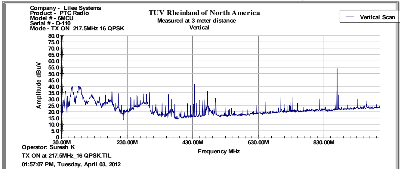
30 MHz to 1GHz Plot for Transmit Mode: 217.5 MHz at 16 QPSK
