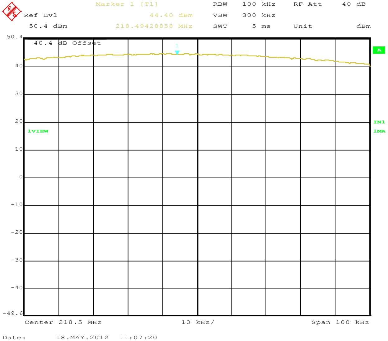
Figure 23: Maximum Transmitted Power, 218.5 MHz at 16 QPSK Mobile application
