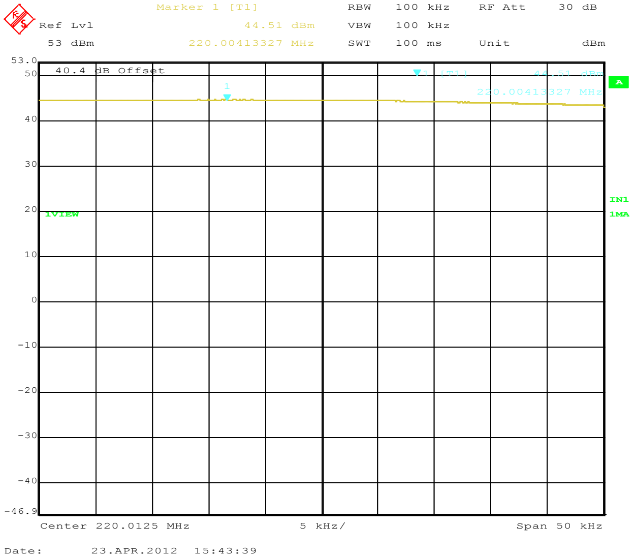
Figure 10: Maximum Transmitted Power, 220.0125 MHz at GMSK
