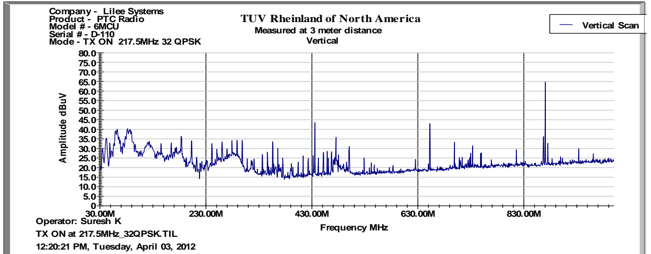
30 MHz to 1GHz Plot for Transmit Mode: 32 QPSK
