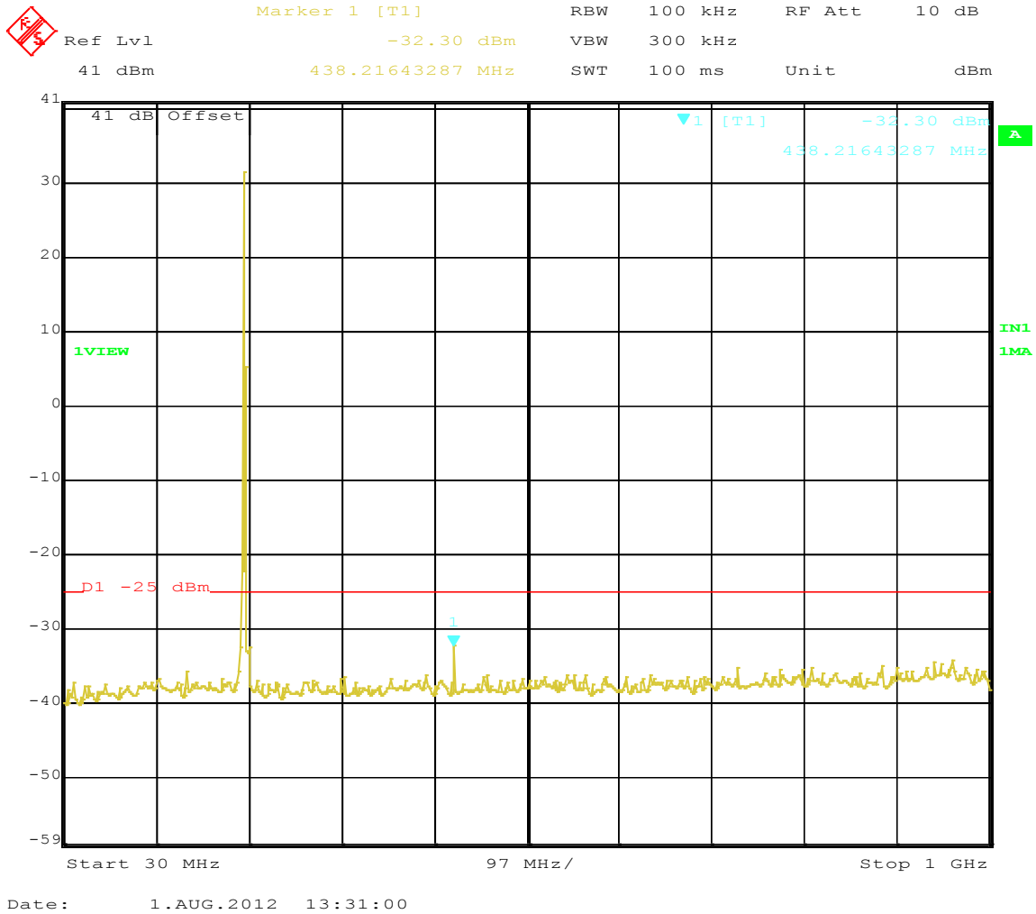
Figure 93: Out of Band Emissions Operating 219.5 MHz 16 QPSK Plot 1
