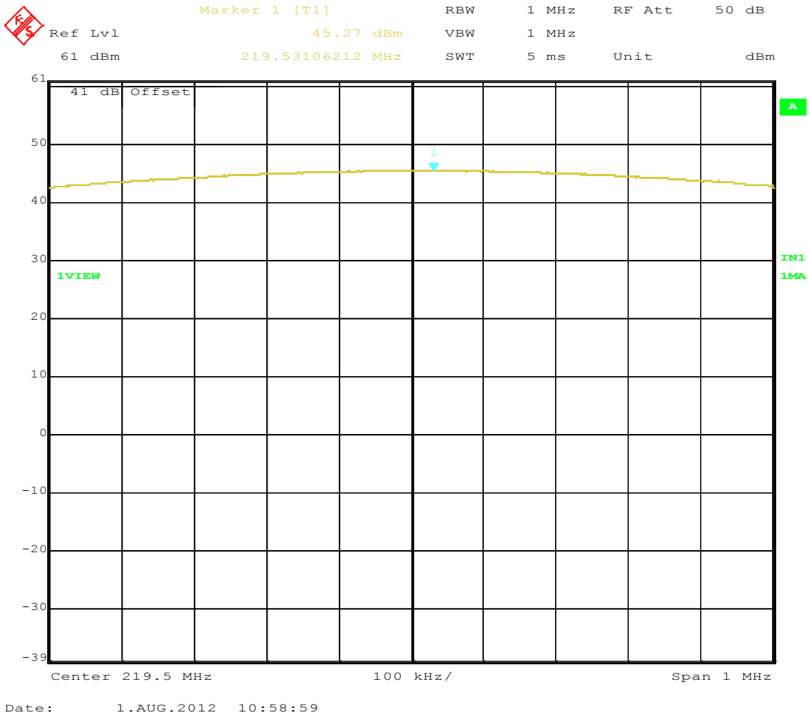
Figure 27: Maximum Transmitted Power, 219.5 MHz at 16 QPSK Power for Base station application
