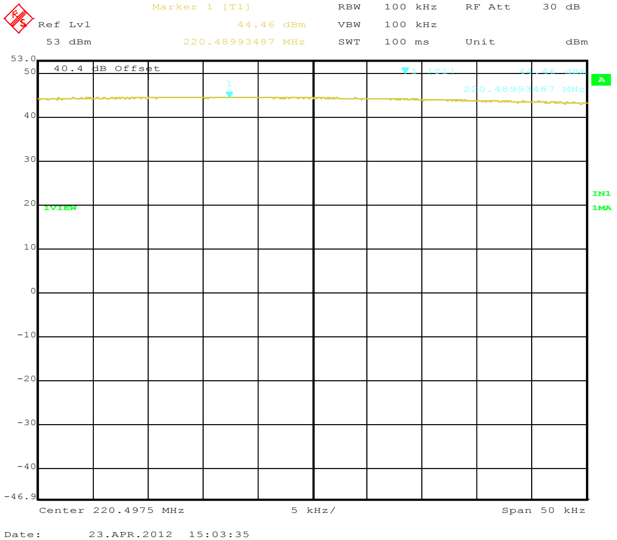
Figure 14: Maximum Transmitted Power, 220.4875 MHz at 16 QPSK
