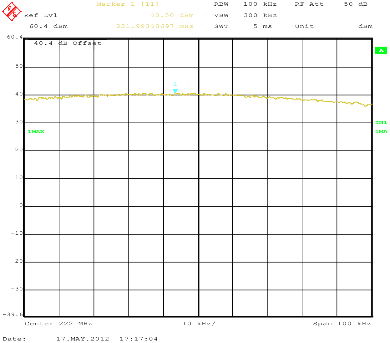
Figure 21: Maximum Transmitted Power, 222 MHz at 32 QPSK
