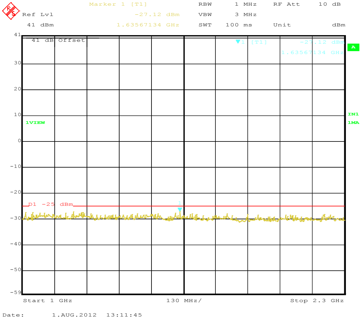
Figure 96: Out of Band Emissions Operating 219.5 MHz 32QPSK Plot 2
