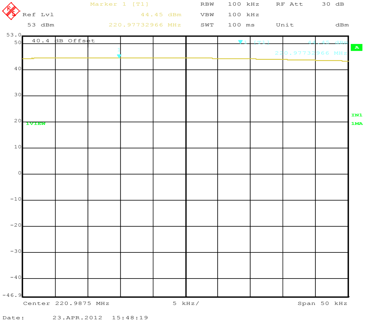
Figure 16: Maximum Transmitted Power, 220.9875 MHz at GMSK
