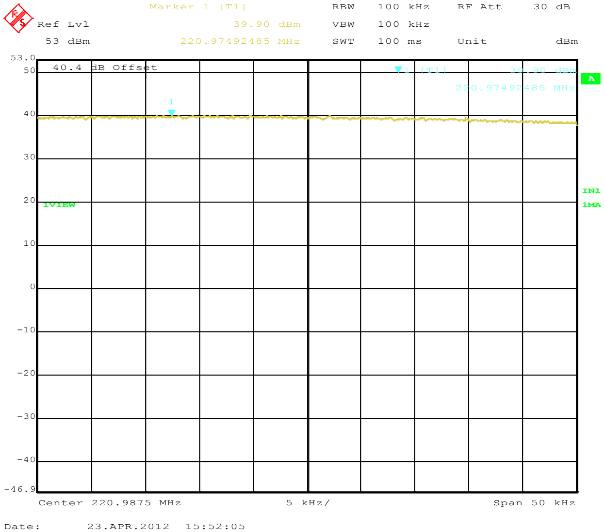
Figure 18: Maximum Transmitted Power, 220.9875 MHz at 32 QPSK
