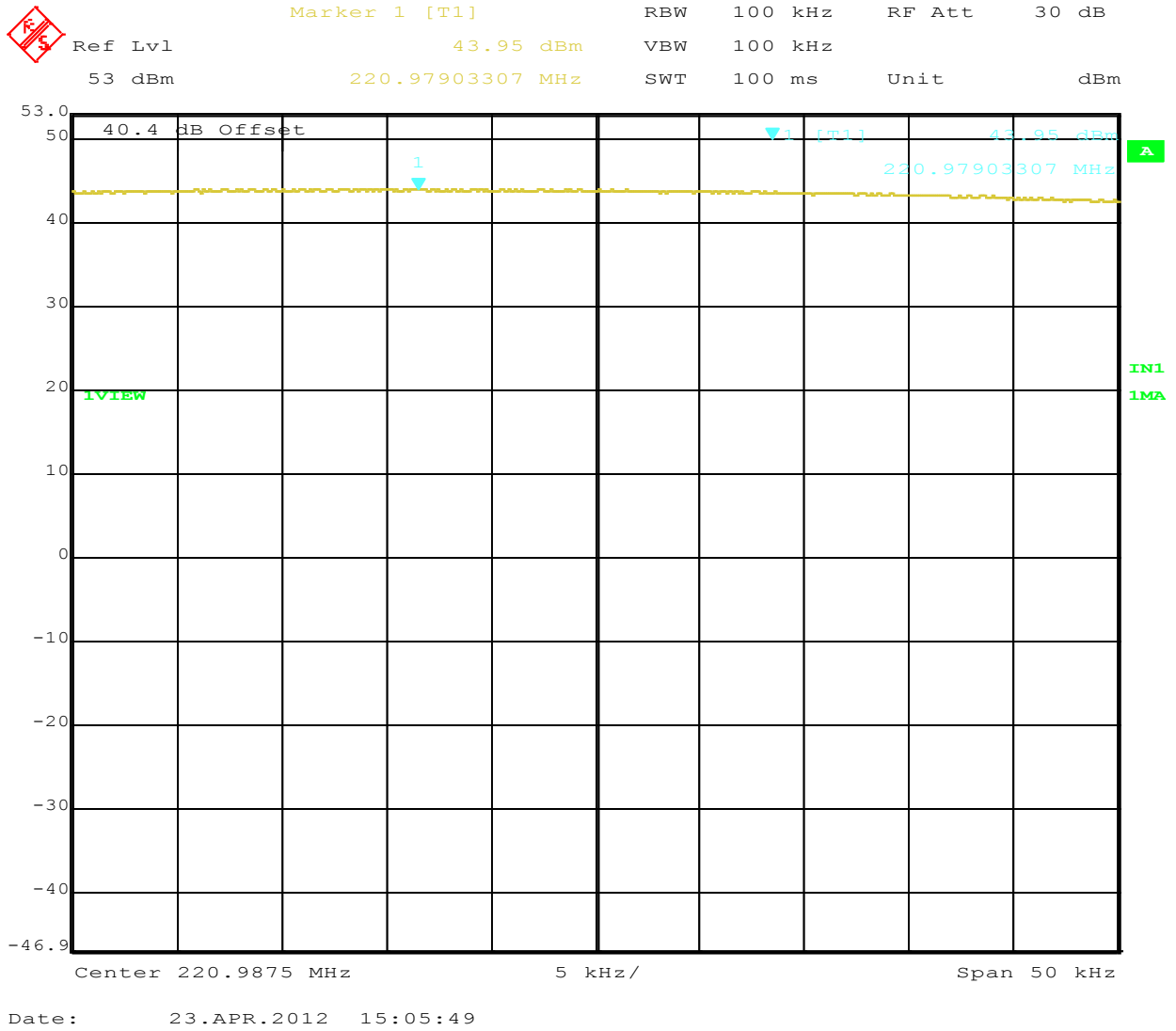
Figure 17: Maximum Transmitted Power, 220.9875 MHz at 16 QPSK
