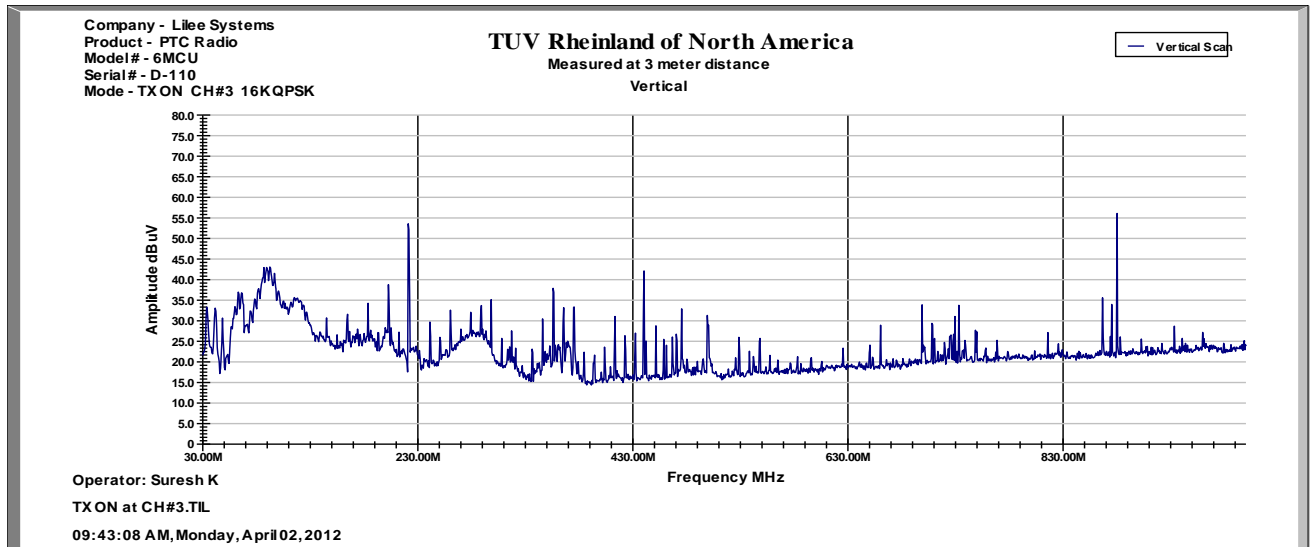
30 MHz to 1GHz Plot for Transmit Mode: TX On 220.0125MHz 16 QPSK
