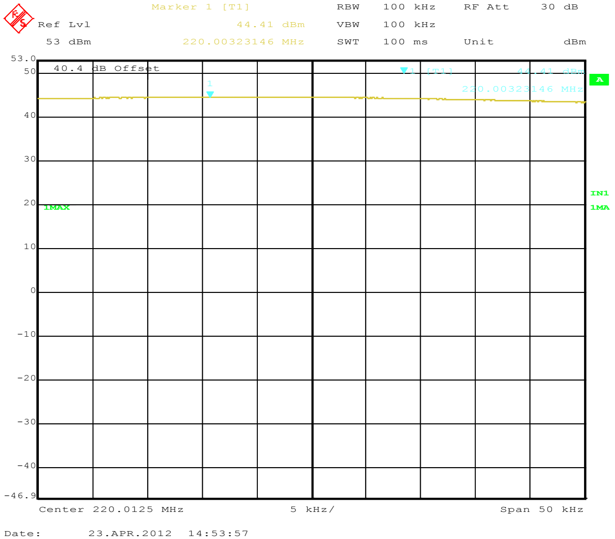
Figure 11: Maximum Transmitted Power, 220.0125 MHz at 16 QPSK
