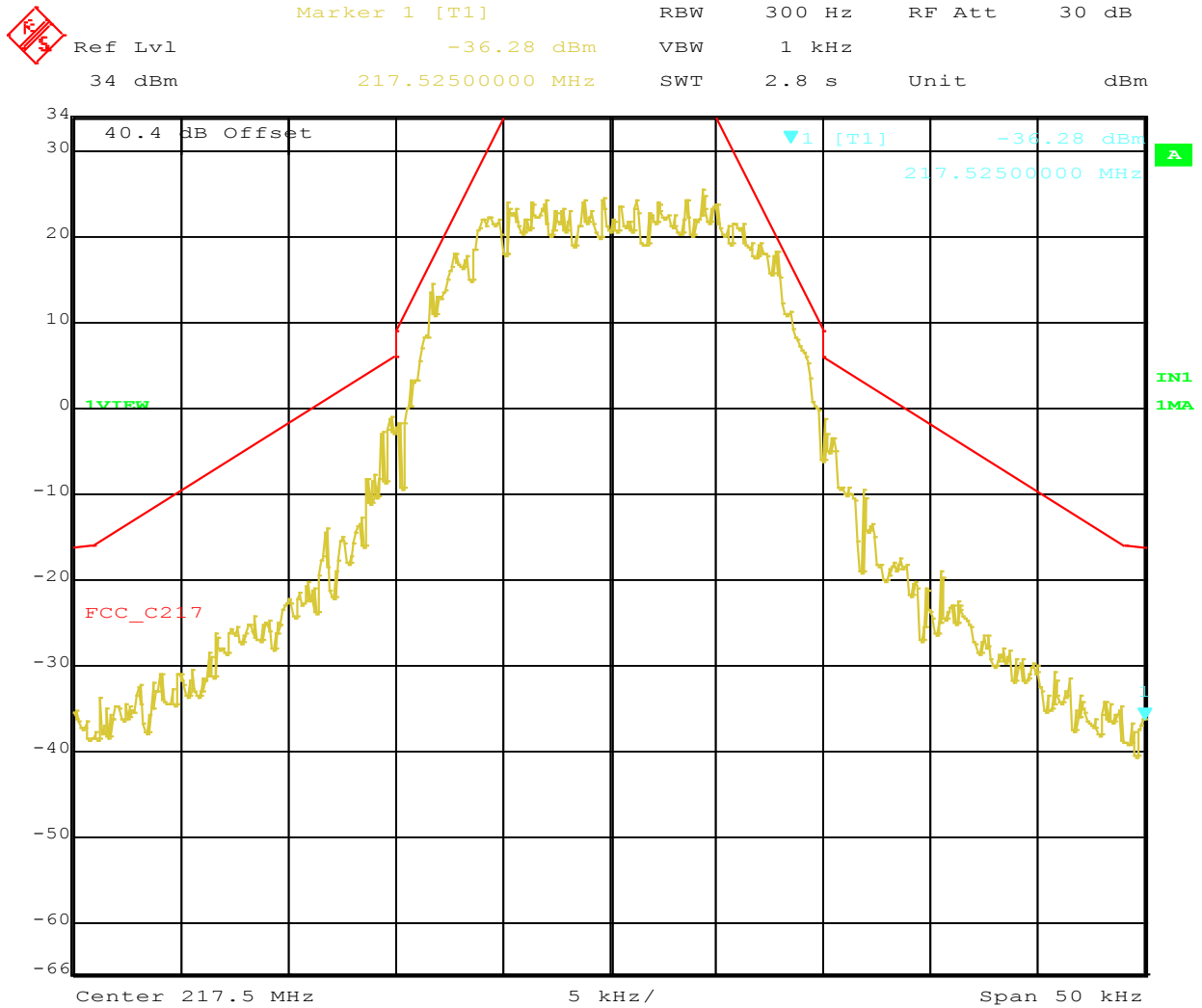
Figure 49: Emission mask C Requirement at Operating Channel 217.5 MHz, 32 QPSK (2 Channel Aggregation)
