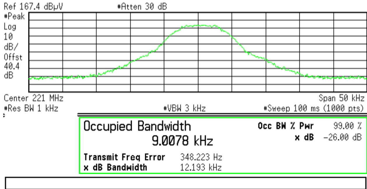
Figure 41: Occupied Bandwidth at Operating Channel 220.9875 MHz at GMSK
