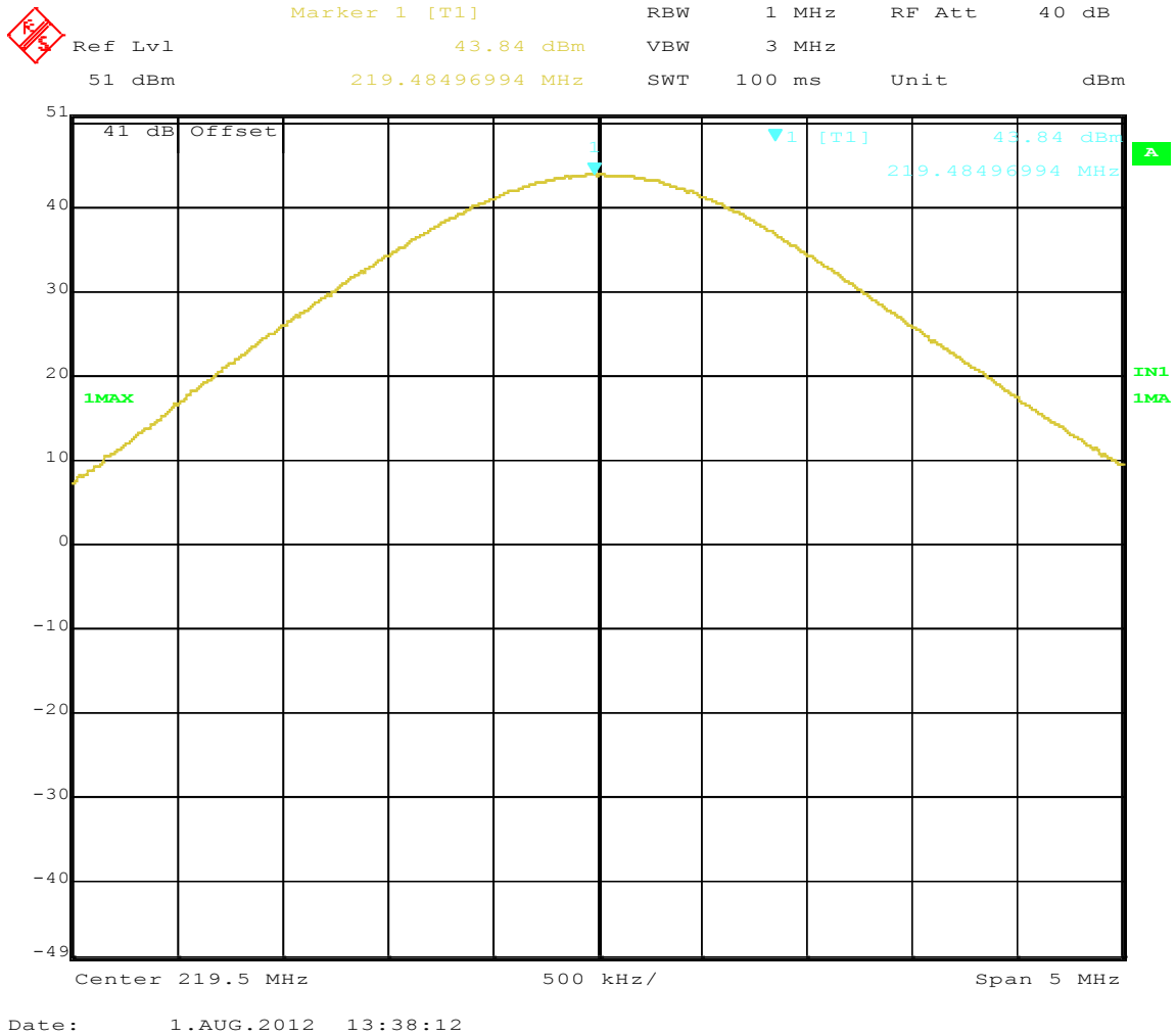
Figure 26: Maximum Transmitted Power, 219.5 MHz at 16 QPSK Power for Base station and mobile application
