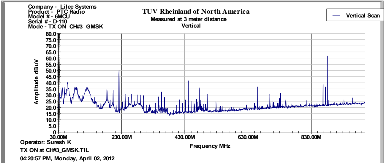
30 MHz to 1GHz Plot for Transmit Mode: 220.0125 MHz at GMSK
