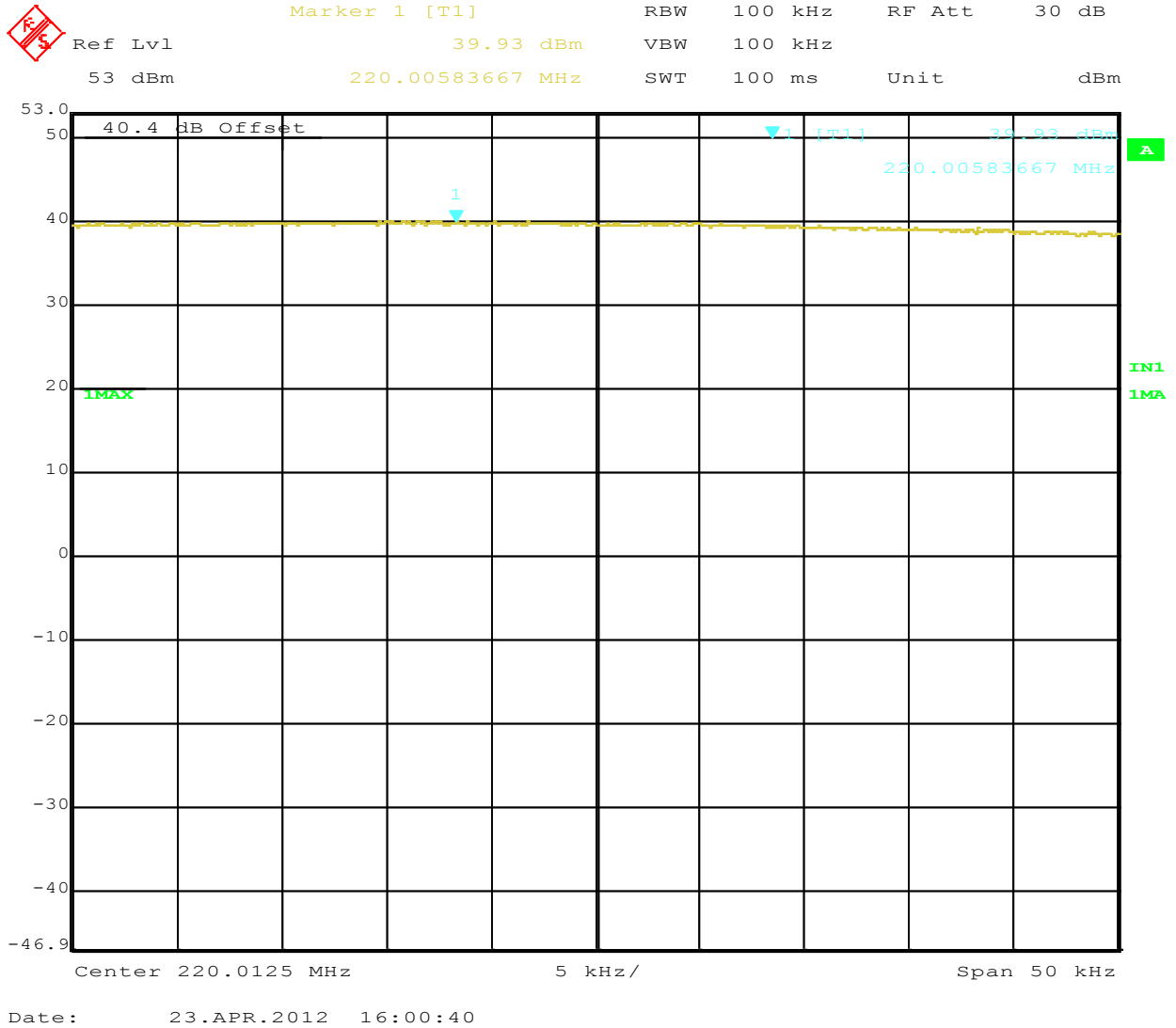
Figure 12: Maximum Transmitted Power, 220.0125 MHz at 32 QPSK
