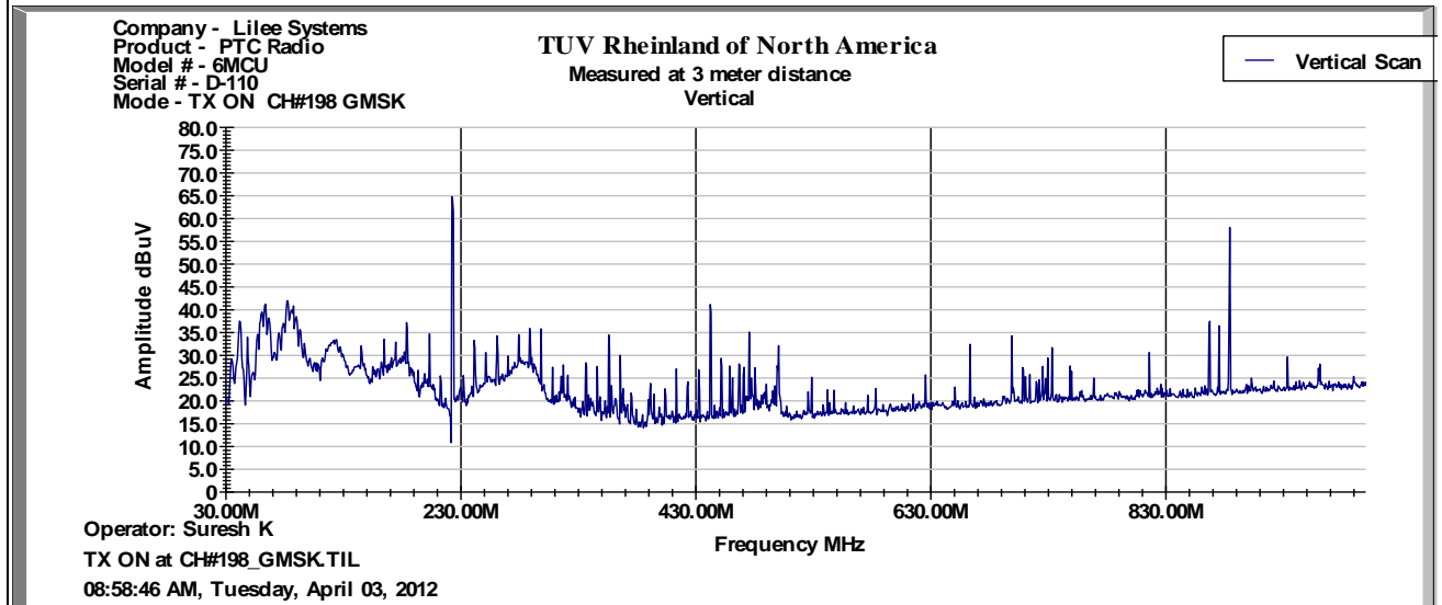
30 MHz to 1GHz Plot for Transmit Mode: 220.9875MHz GMSK
