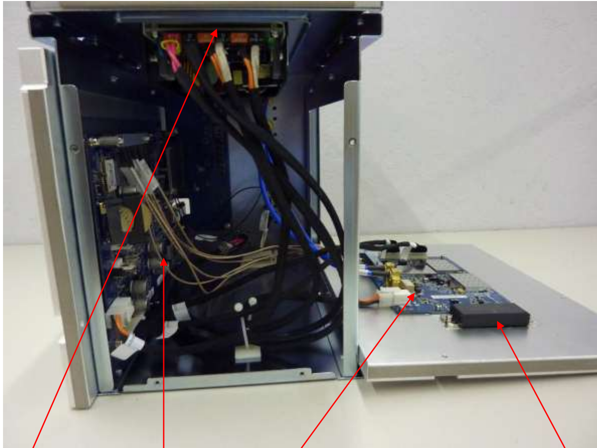
Power Supply
