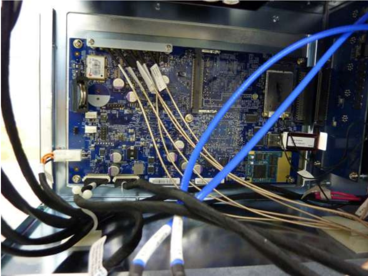
Mainboard inside the housing
