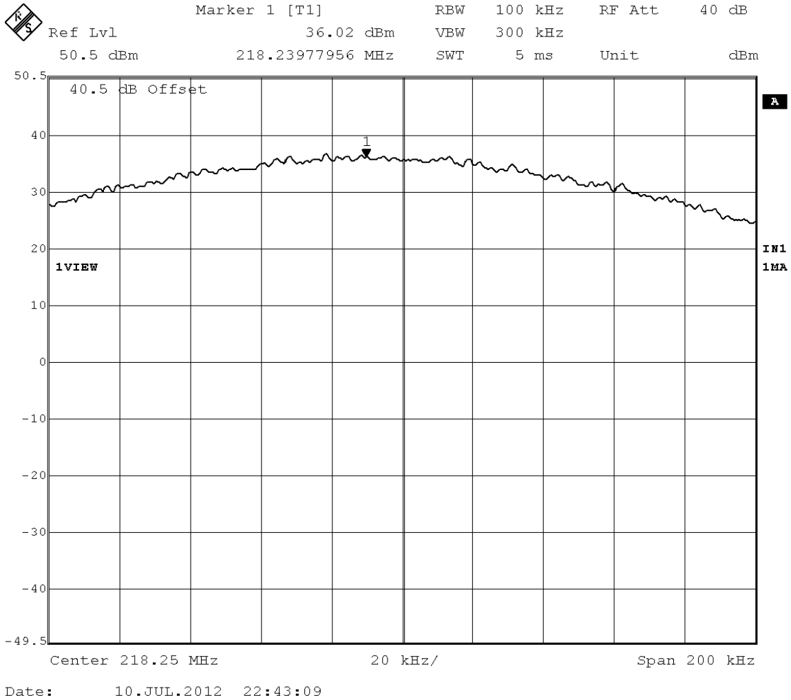
Figure 2: Maximum Transmitted Power, 218.250 MHz at 16 QPSK
