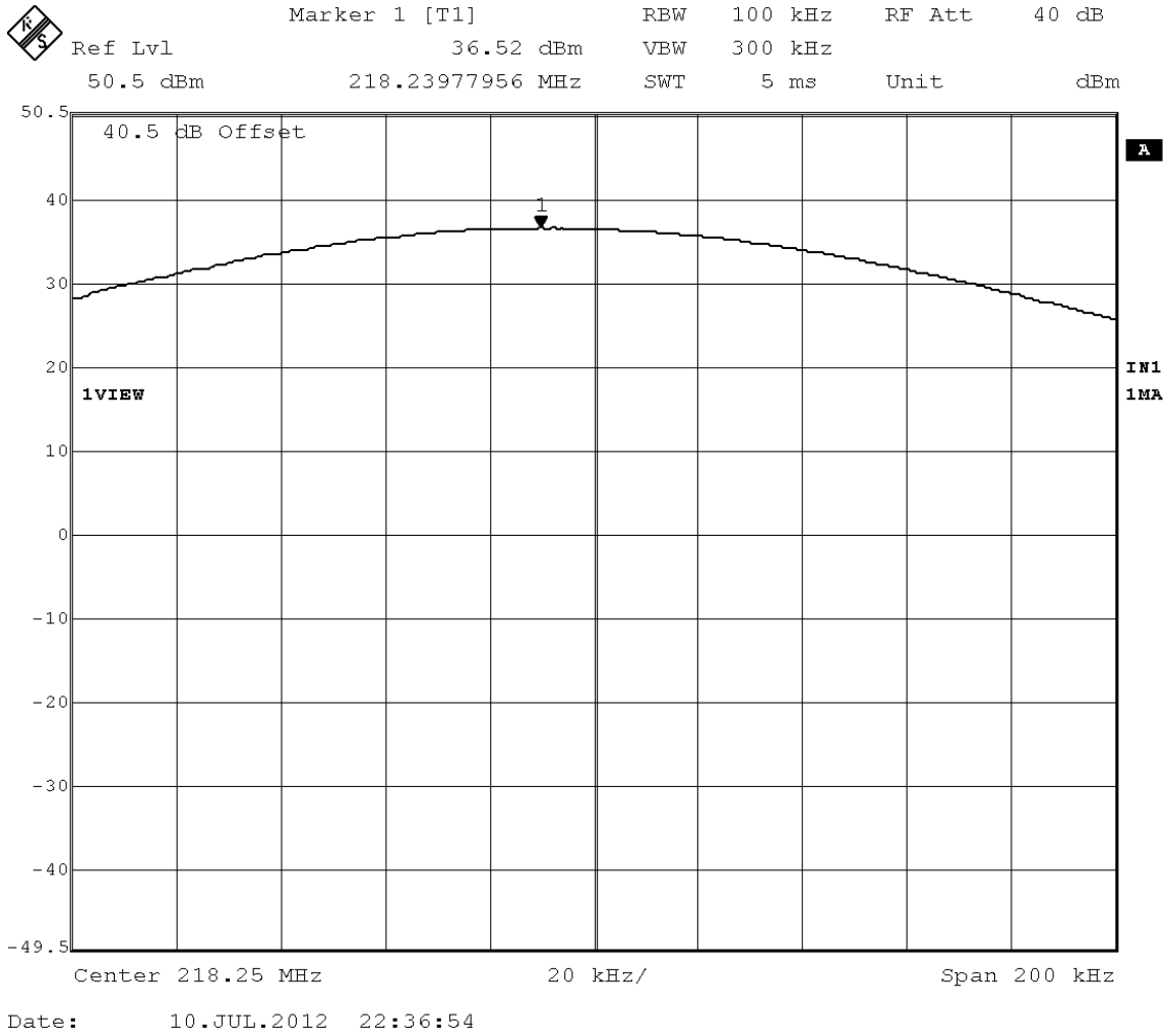
Figure 1: Maximum Transmitted Power, 218.250 MHz at GMSK 9600
