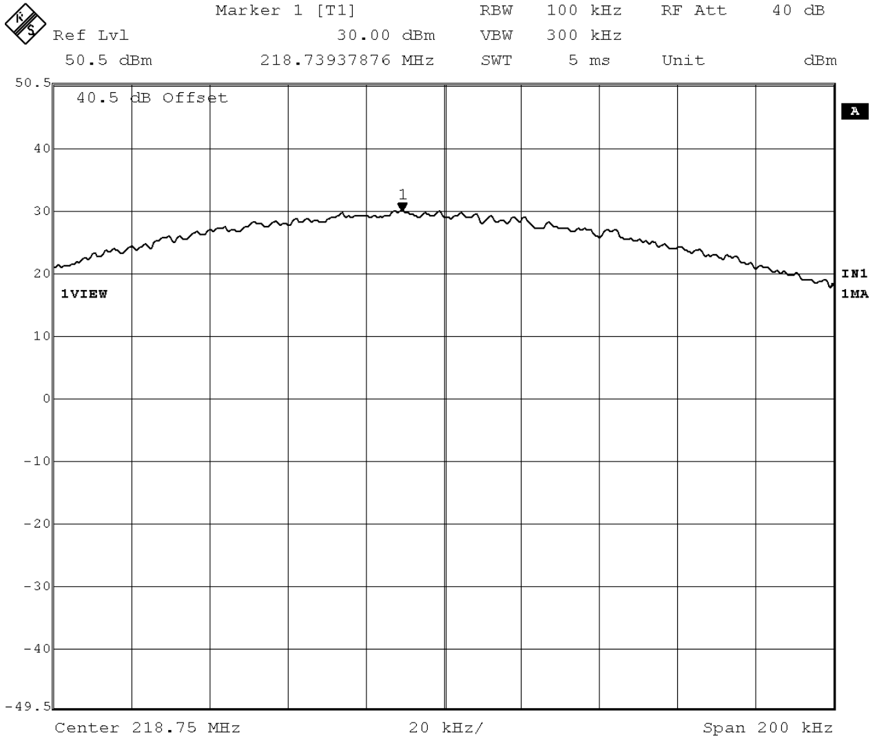
Figure 11: Maximum Transmitted Power, 218.750MHz at 16 QPSK
