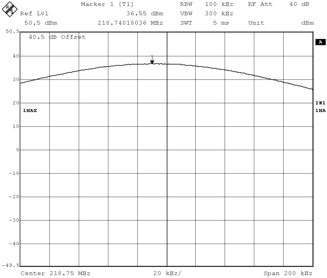
Figure 4: Maximum Transmitted Power, 218.750 MHz at GMSK 9600
