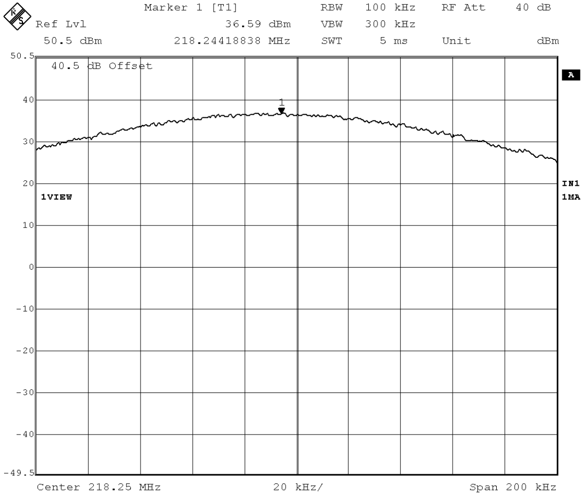
Figure 3: Maximum Transmitted Power, 218.250 MHz at 32 QPSK
