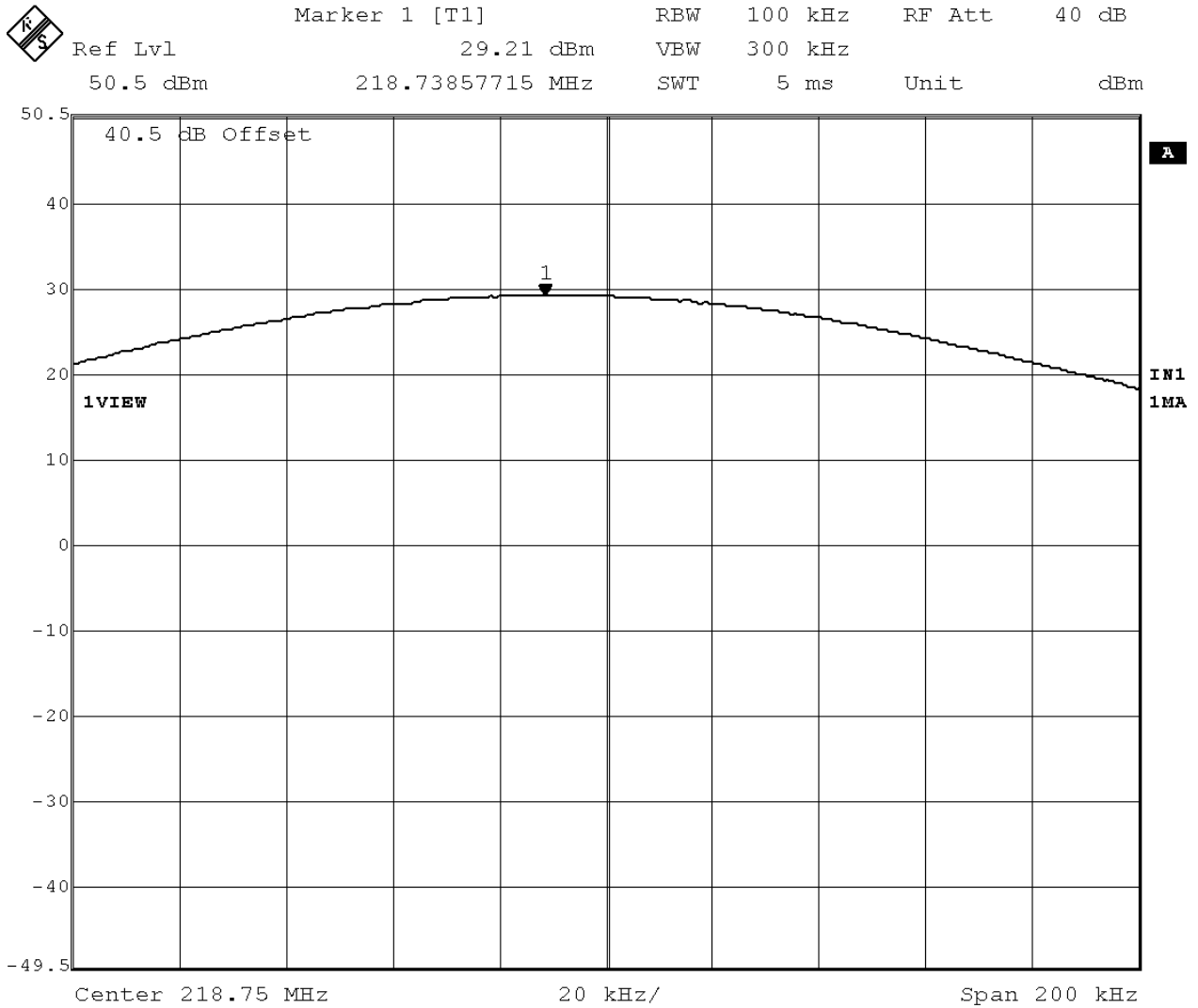
Figure 10: Maximum Transmitted Power, 218.75 MHz GMSK
