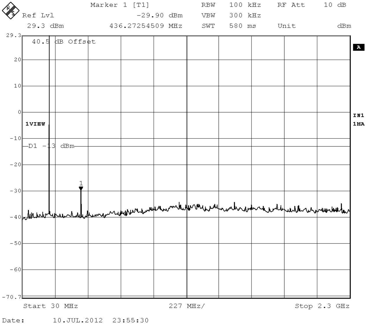
Figure 24: Out of Band Emissions Operating Channel 218.5 MHz at 32 QPSK
