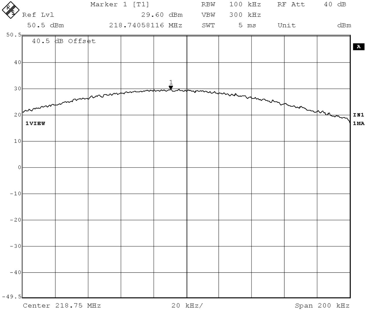
Figure 12: Maximum Transmitted Power, 218.75 MHz at 32 QPSK
