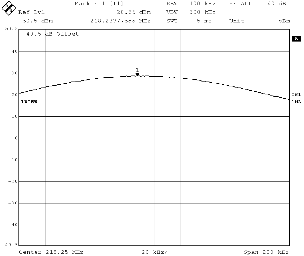
Figure 7: Maximum Transmitted Power, 218.25 MHz at GMSK
