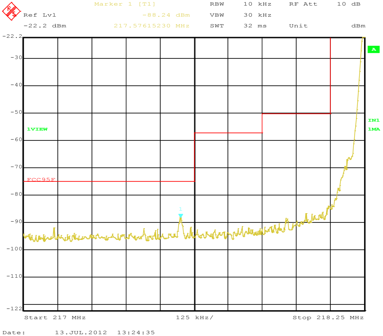
Figure 19: Emission mask Requirement at Operating Channel 218.25 MHz at 16 QPSK
