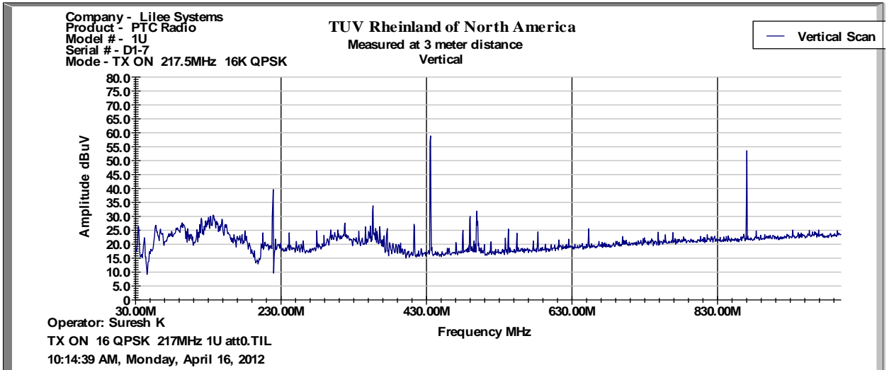
30 MHz to 1GHz Plot for Transmit Mode: 217.5 MHz at 16 QPSK
