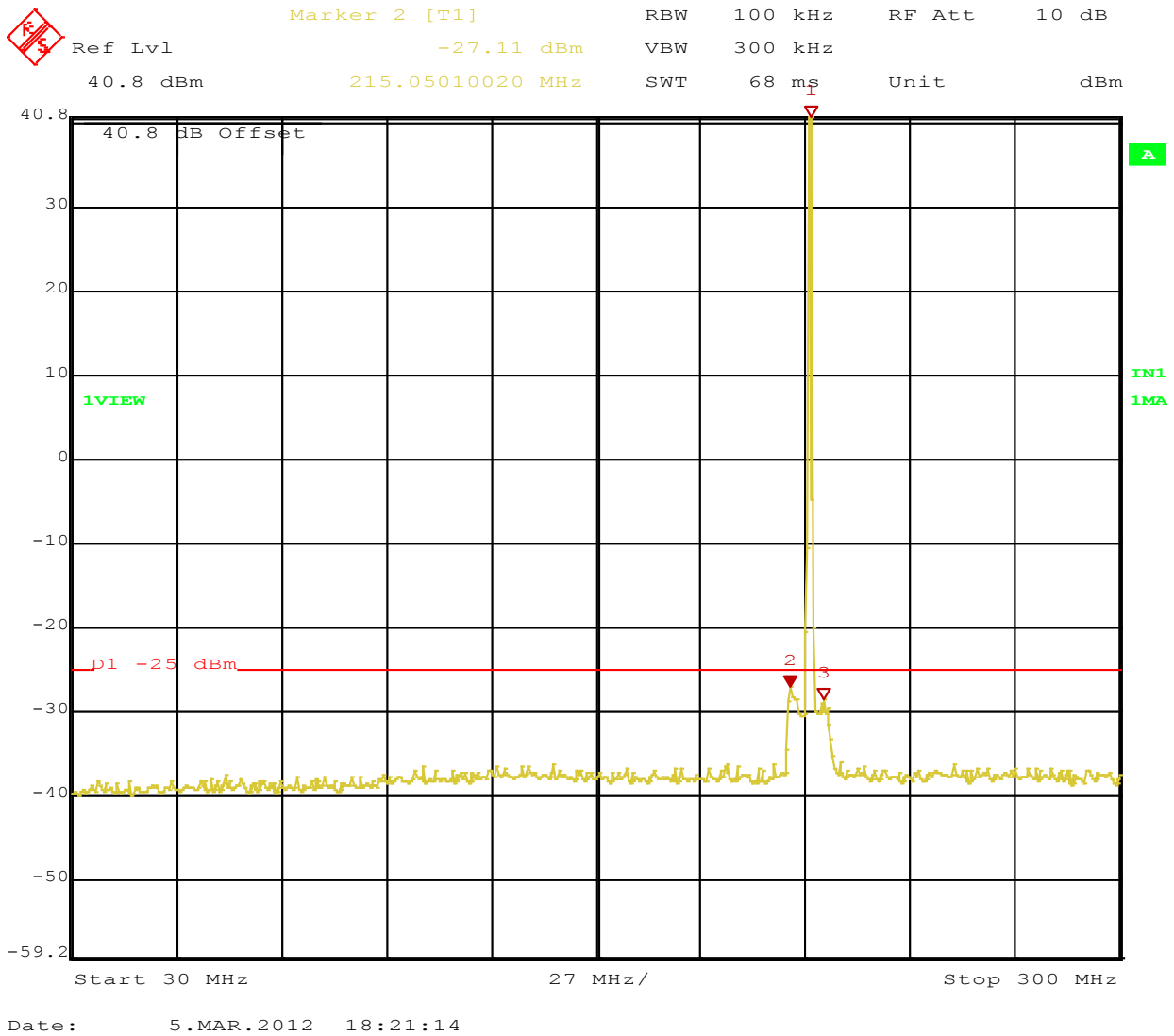
Figure 79: Out of Band Emissions Operating Channel 220.0125 MHz, 32 QPSK Plot 1
