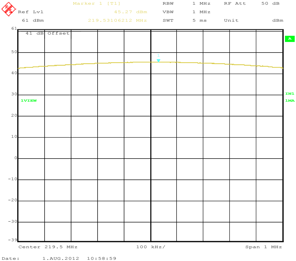
Figure 27: Maximum Transmitted Power, 219.5 MHz at 16 QPSK Power for Base Station application
