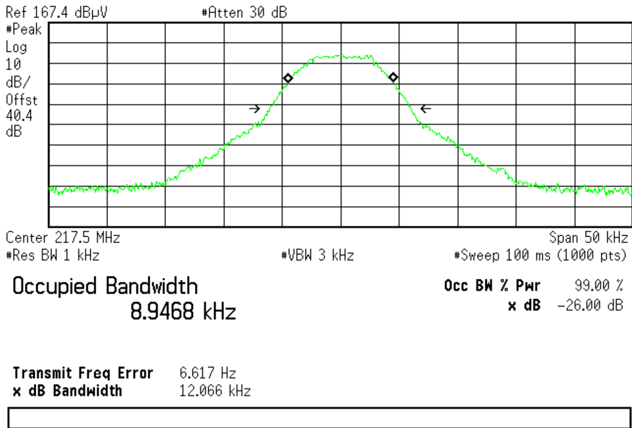
Figure 32: Occupied Bandwidth at Operating Channel 217.5 MHz at GMSK
