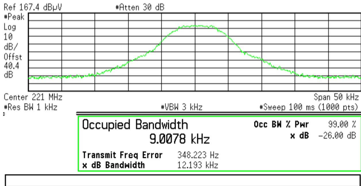
Figure 41: Occupied Bandwidth at Operating Channel 220.9875 MHz GMSK
