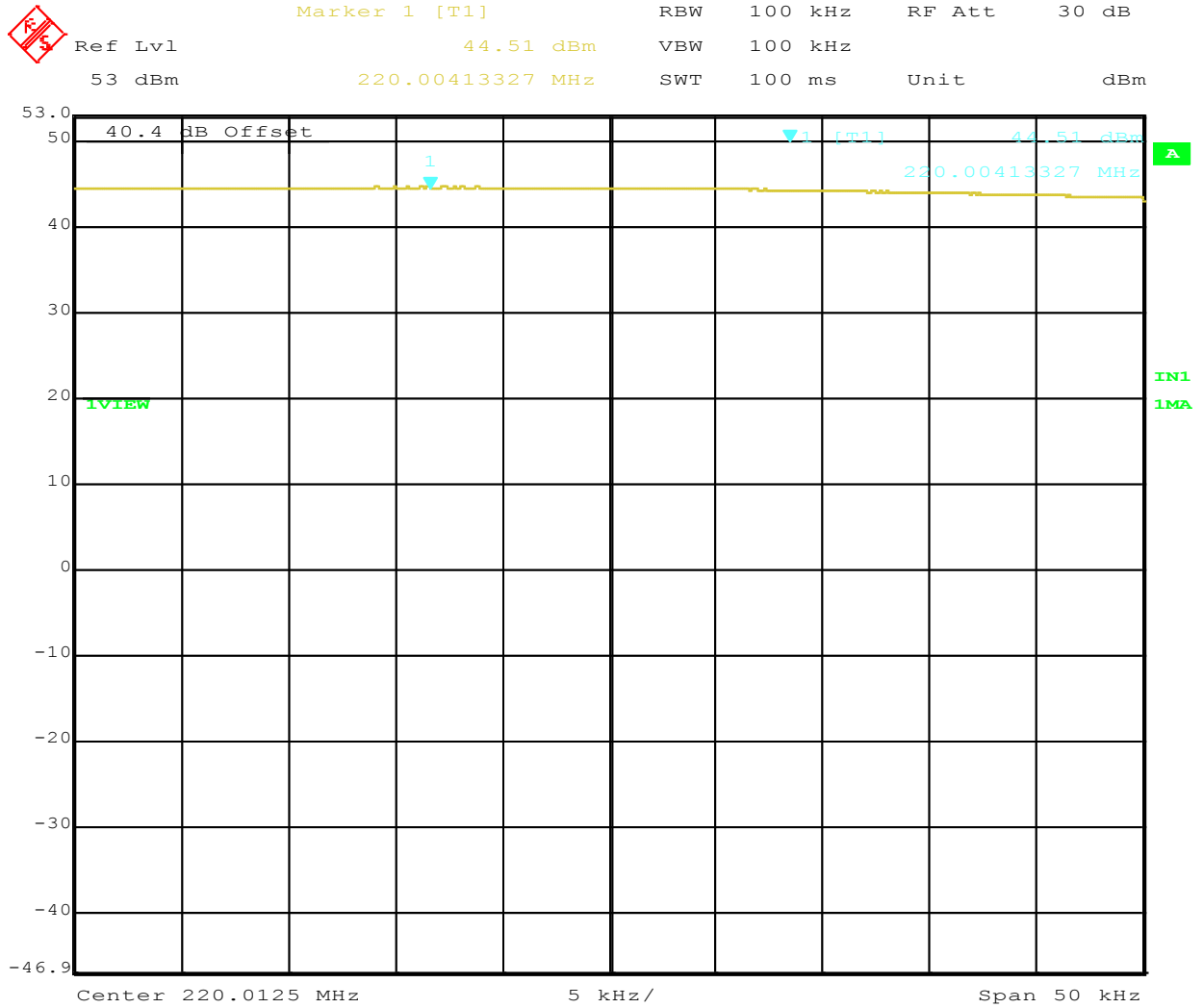
Figure 10: Maximum Transmitted Power, 220.0125 MHz at GMSK
