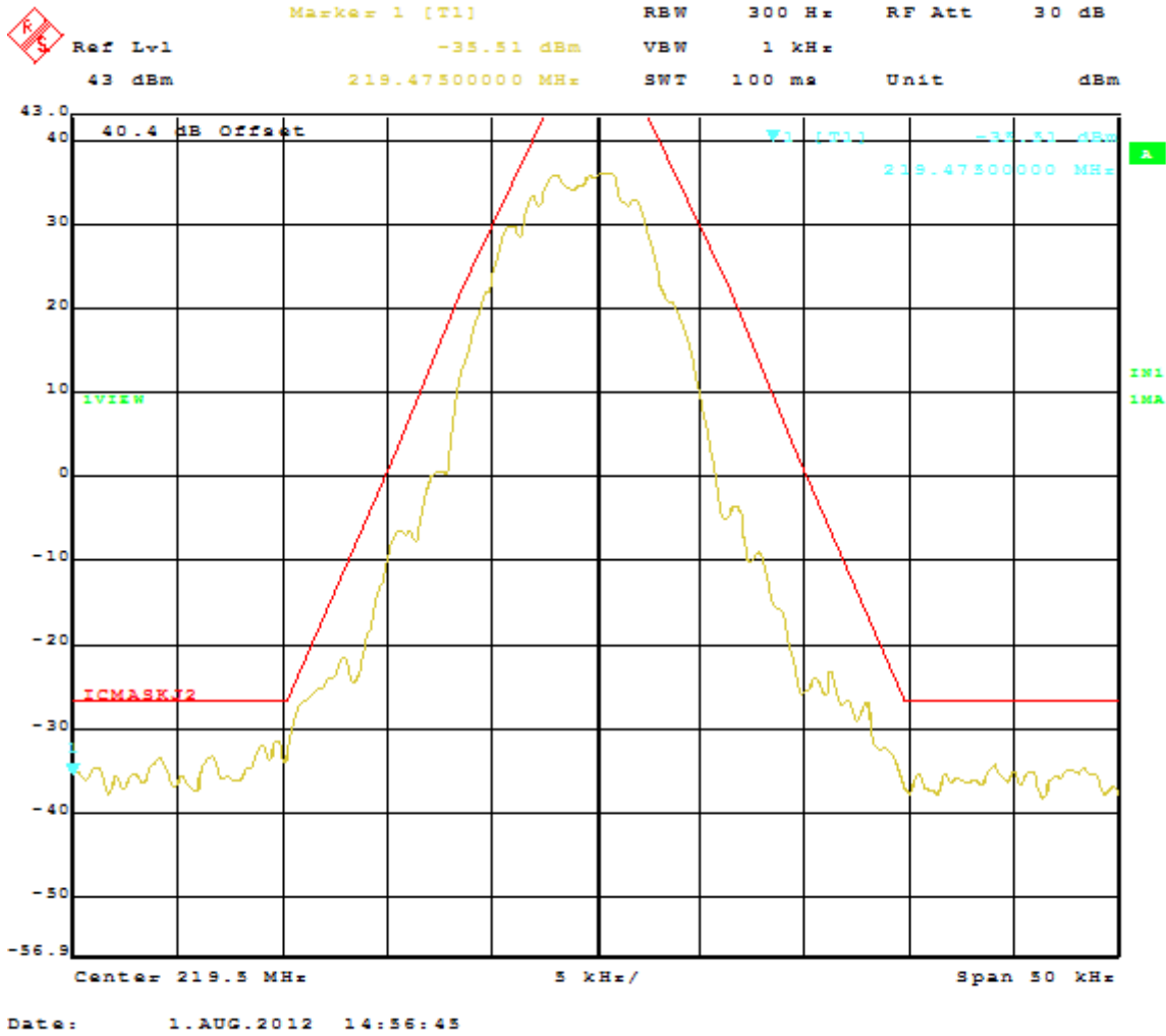
Figure 60: Emission mask J Requirement at Operating Channel 219.5 MHz, GMSK
