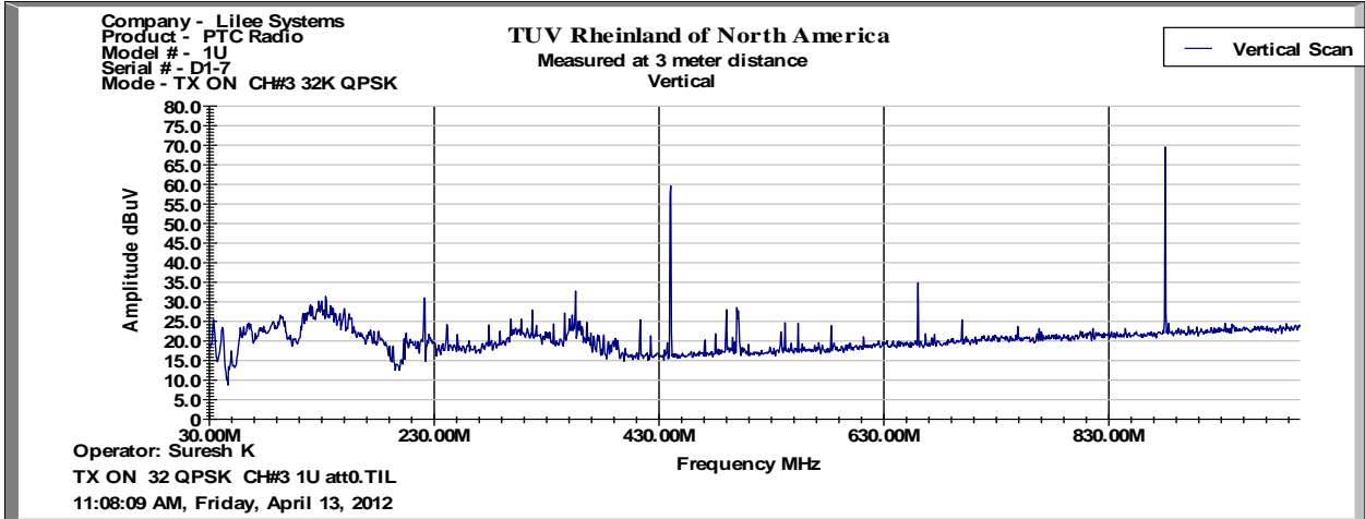
30 MHz to 1GHz Plot for Transmit Mode: 32 QPSK 220.0125 MHz
