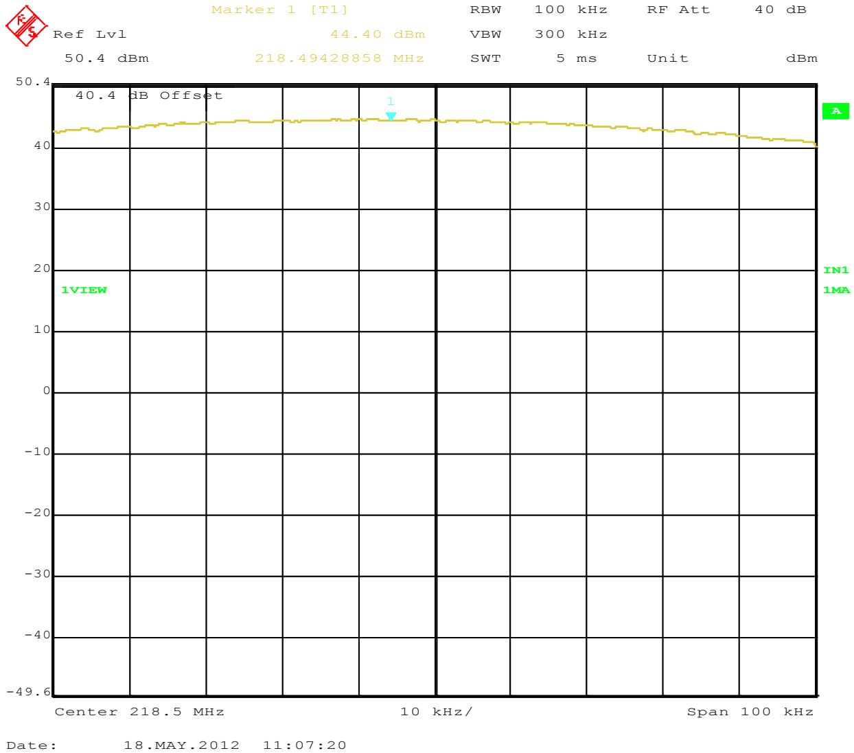
Figure 23: Maximum Transmitted Power, 218.5 MHz at 16 QPSK for Mobile application
