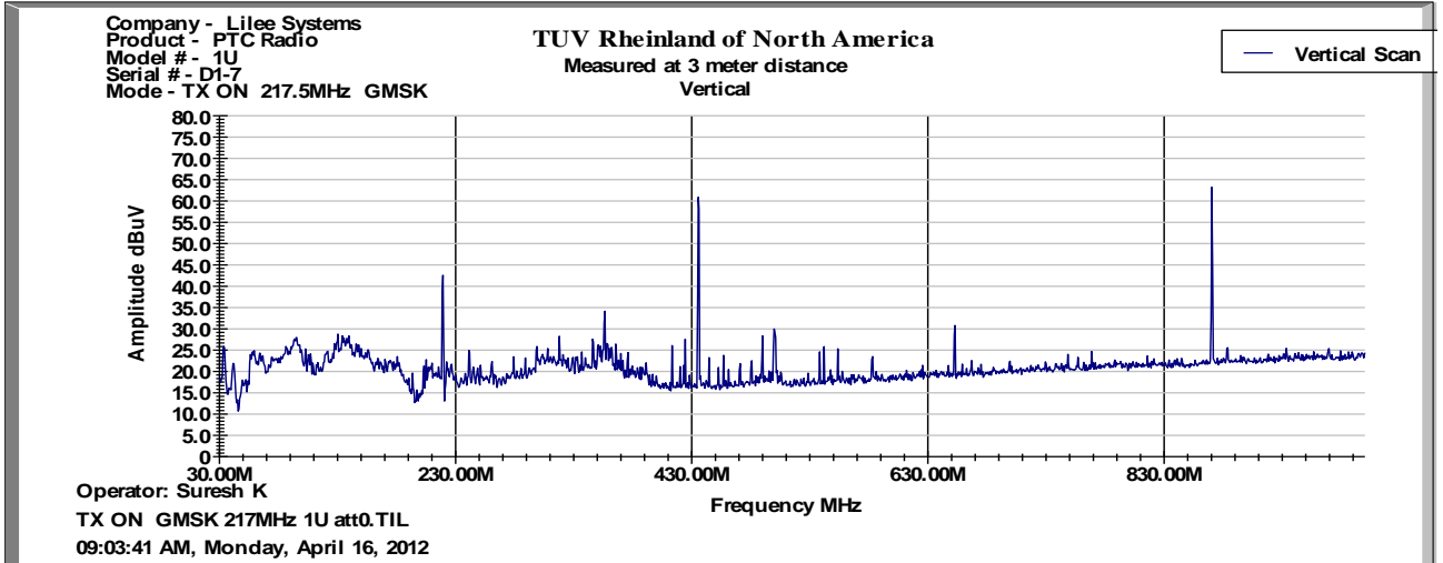
30 MHz to 1GHz Plot for Transmit Mode: GMSK 217.5 MHz
