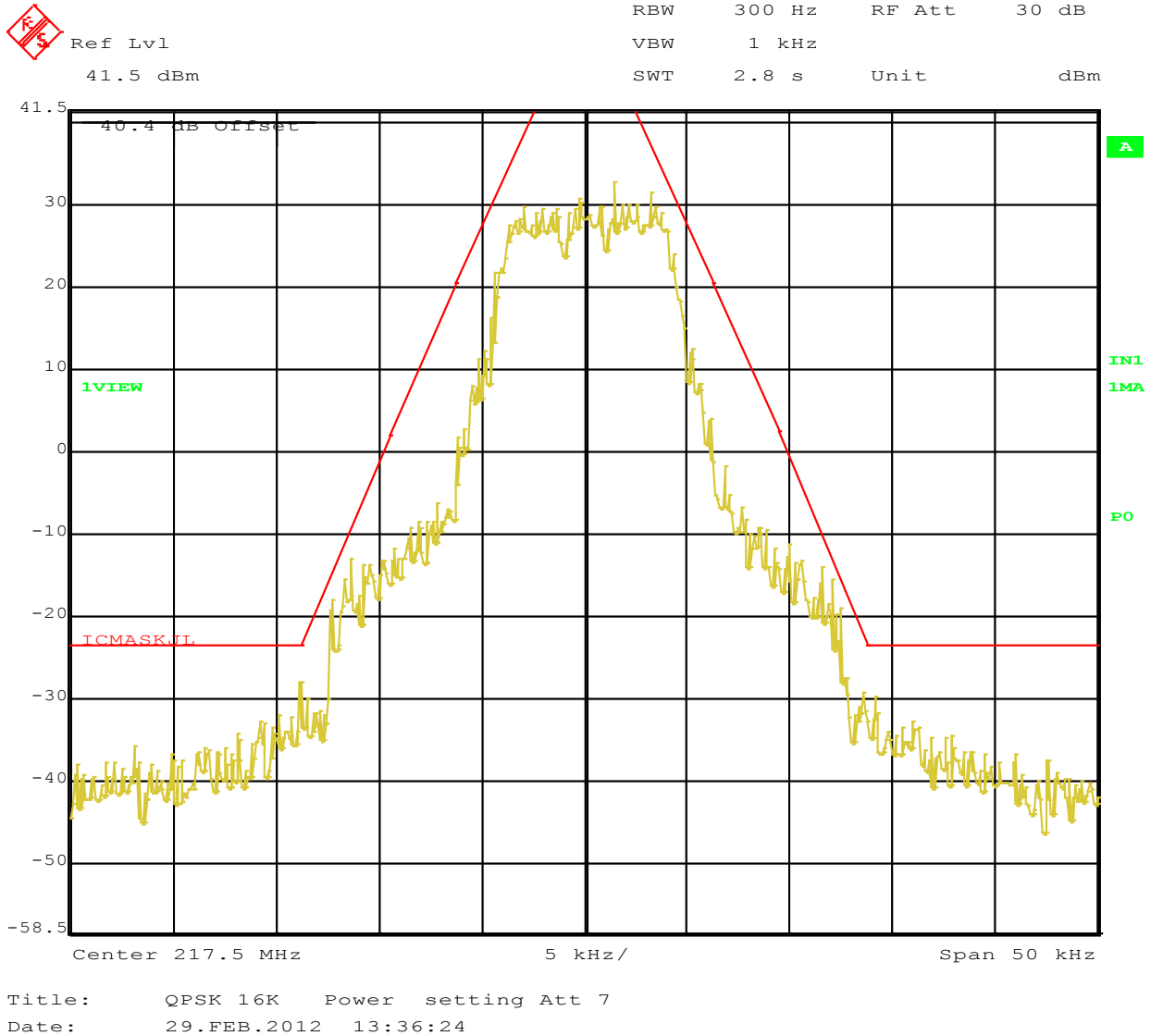
Figure 48: Emission mask J Requirement at Operating Channel 217.5 MHz, 16 QPSK
