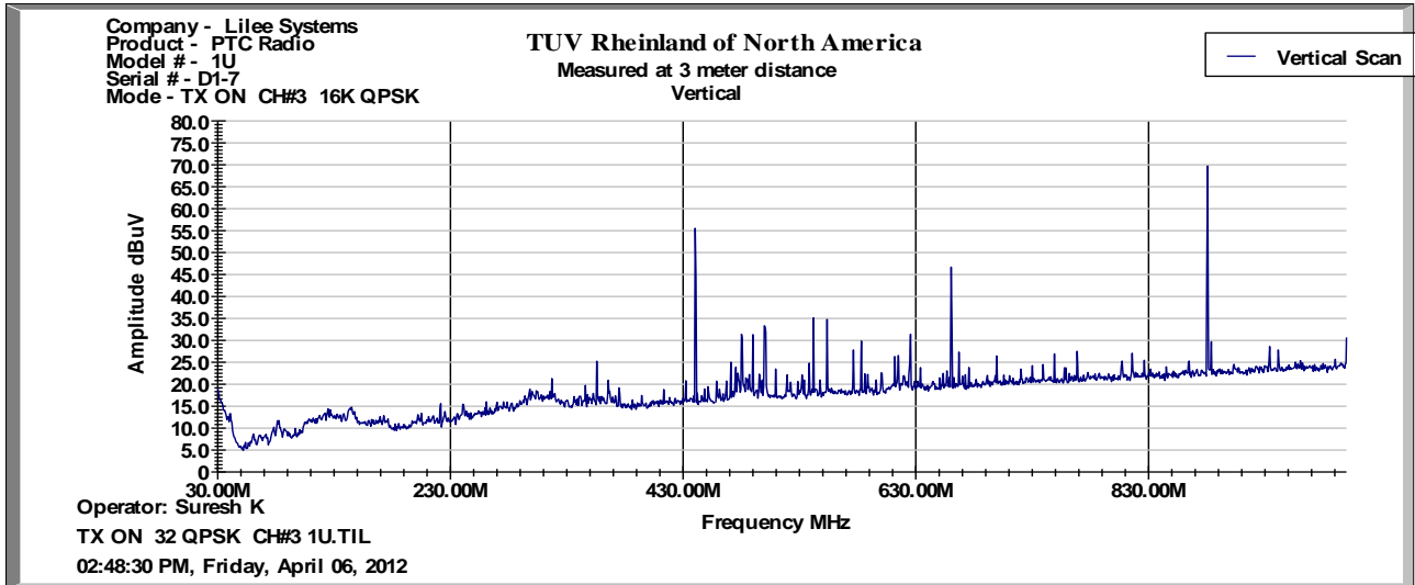
30 MHz to 1GHz Plot for Transmit Mode: 16 QPSK
