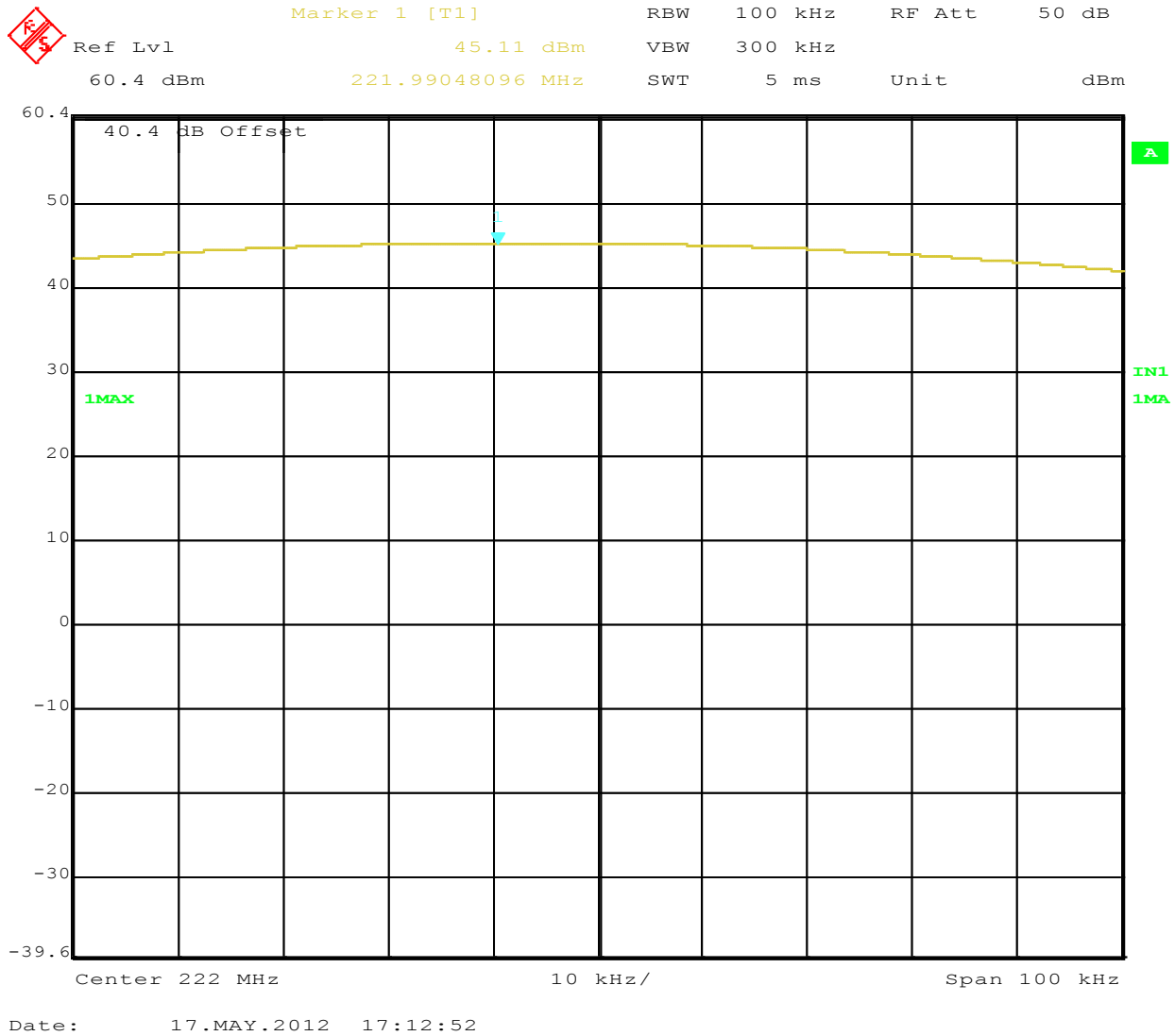
Figure 19: Maximum Transmitted Power, 222 MHz at GMSK
