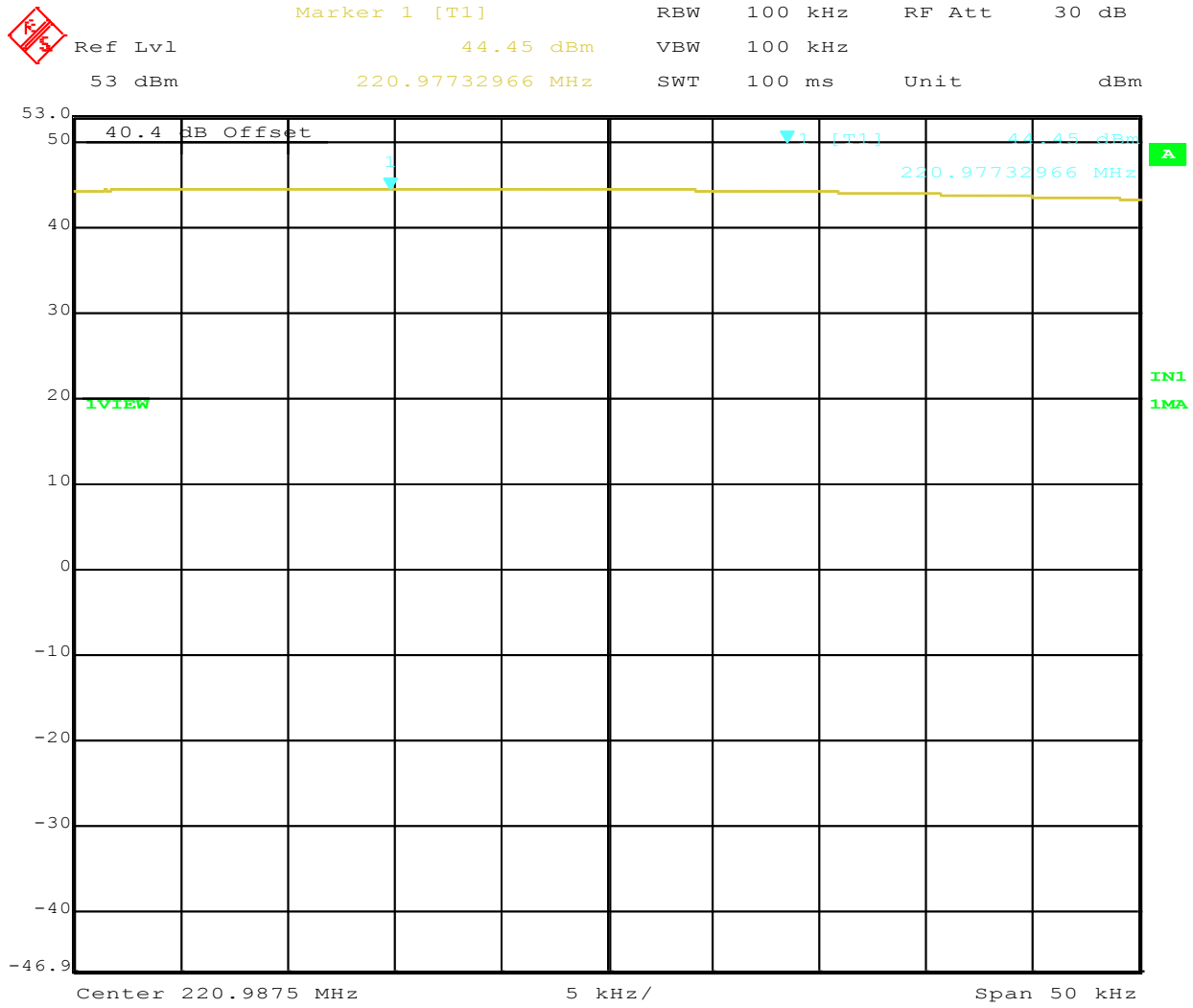
Figure 16: Maximum Transmitted Power, 220.9875 MHz at GMSK
