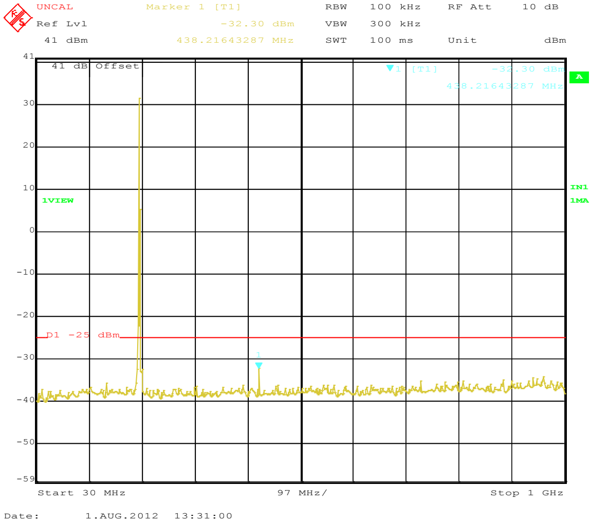
Figure 93: Out of Band Emissions Operating 219.5 MHz 16 QPSK Plot 1
