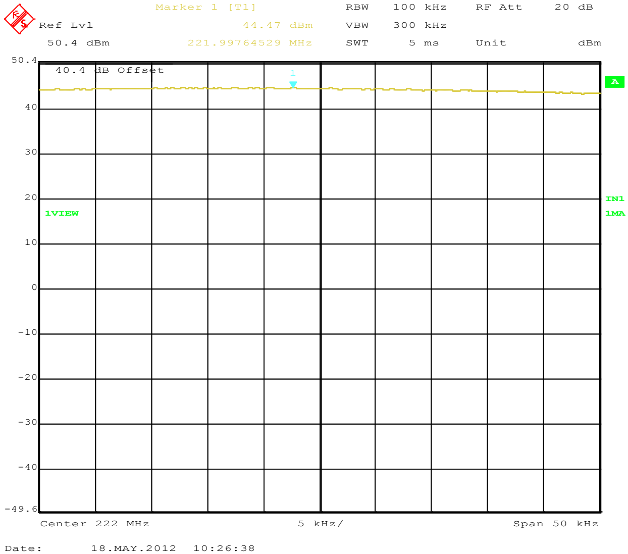
Figure 20: Maximum Transmitted Power, 222 MHz at 16 QPSK
