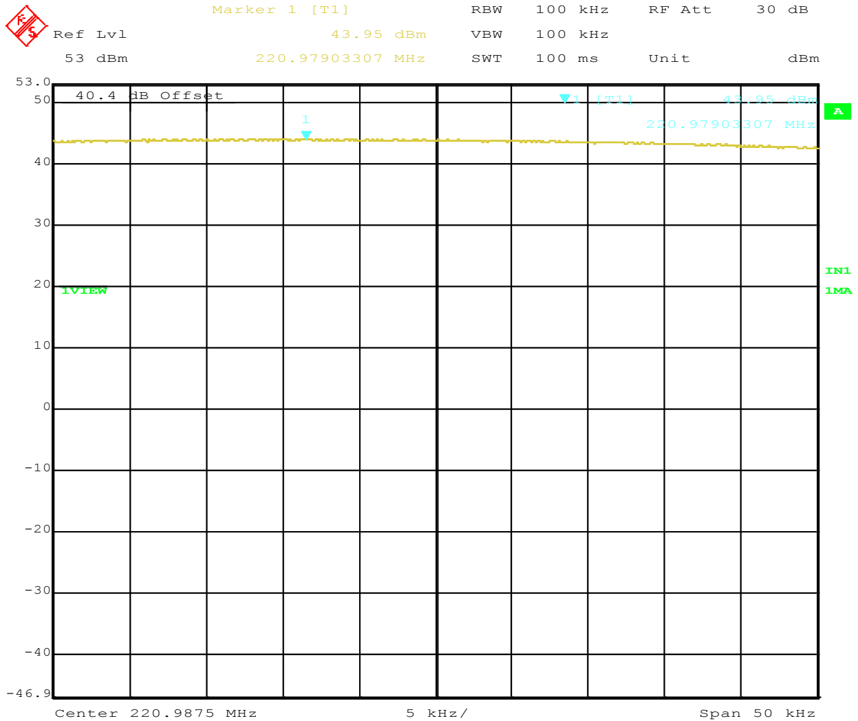
Figure 17: Maximum Transmitted Power, 220.9875 MHz at 16 QPSK
