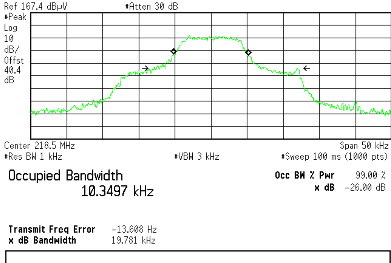
Figure 36: Occupied Bandwidth at Operating Channel 218.5 MHz at 16 QPSK
