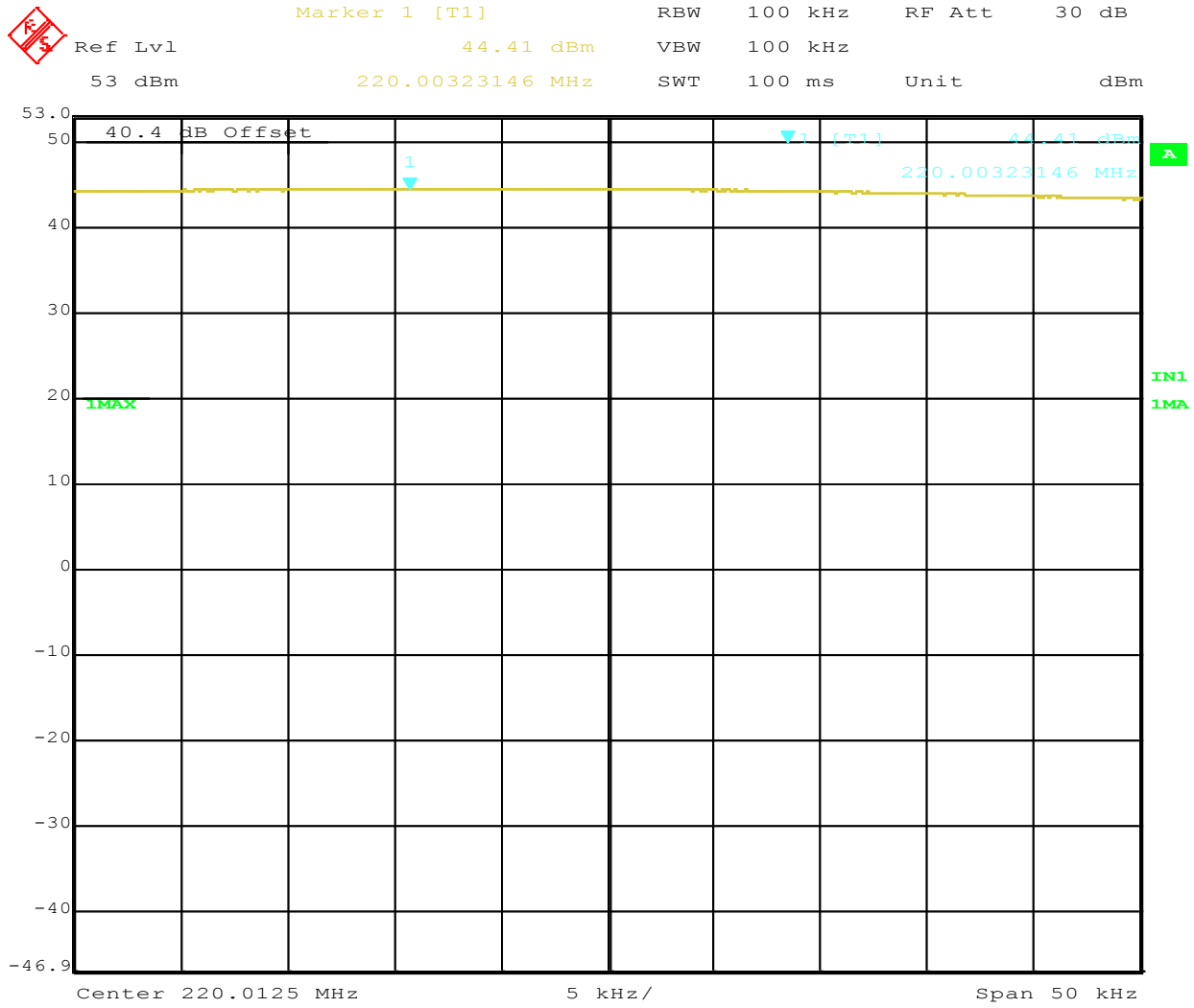
Figure 11: Maximum Transmitted Power, 220.0125 MHz at 16 QPSK
