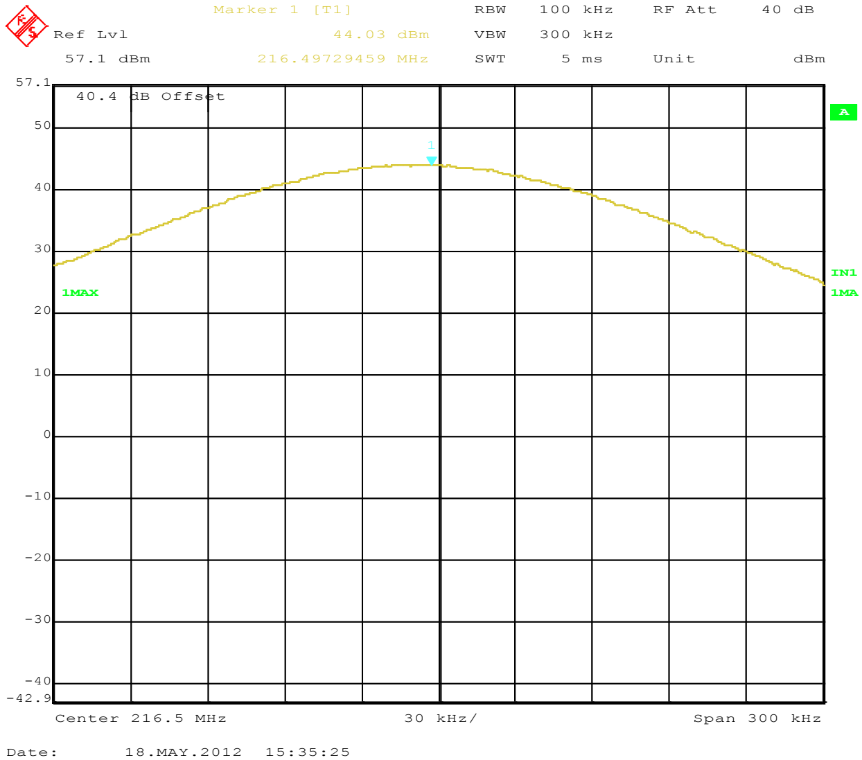
Figure 2: Maximum Transmitted Power, 216.5 MHz at 16 QPSK
