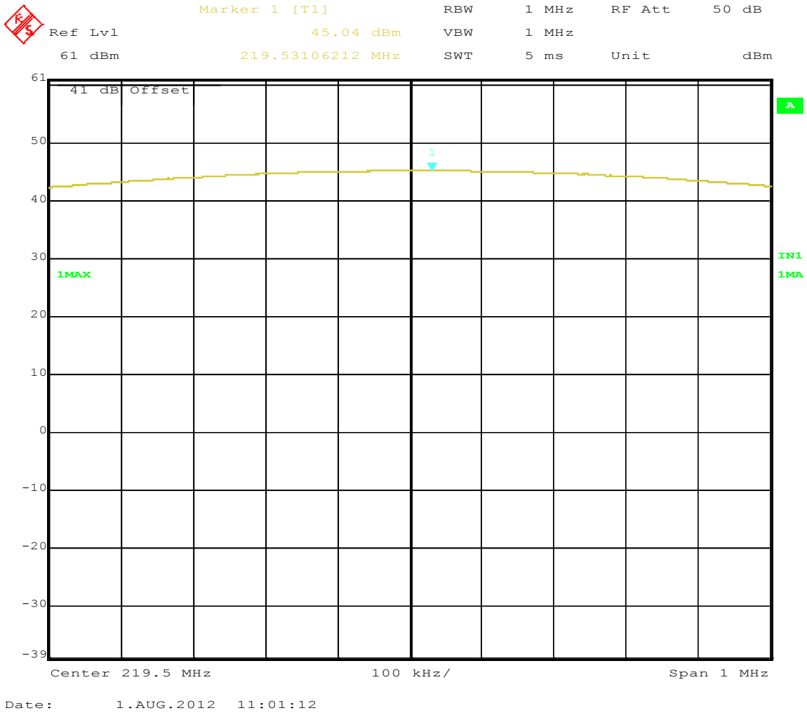
Figure 24: Maximum Transmitted Power, 219.5 MHz at GMSK Power for Fixed application
