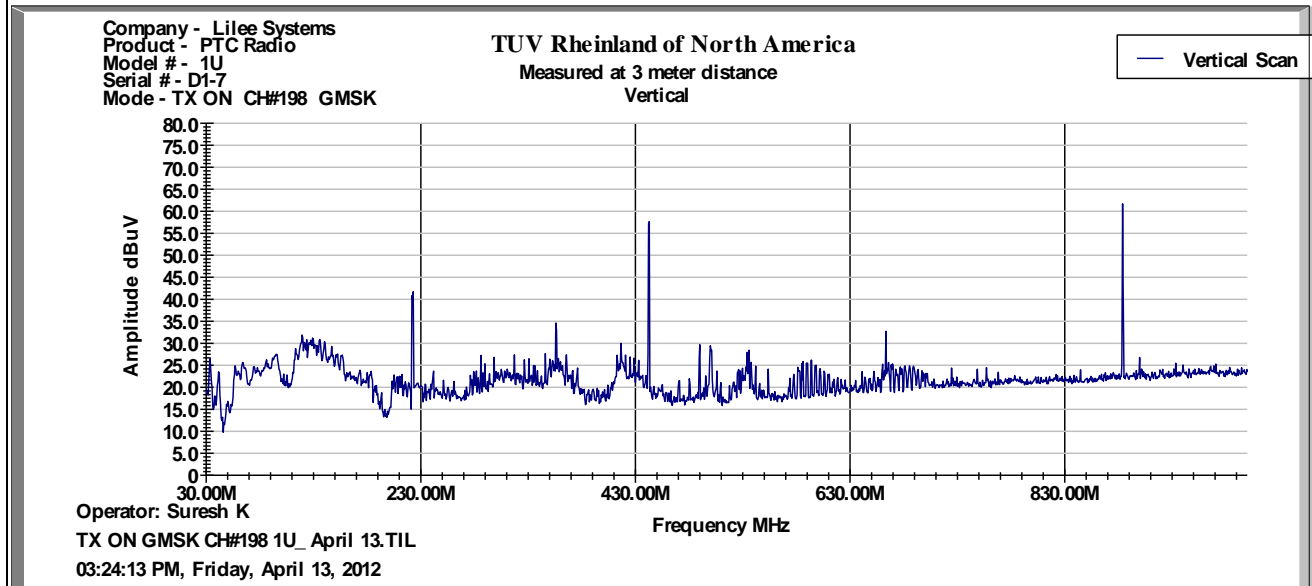
30 MHz to 1GHz Plot for Transmit Mode: GMSK
