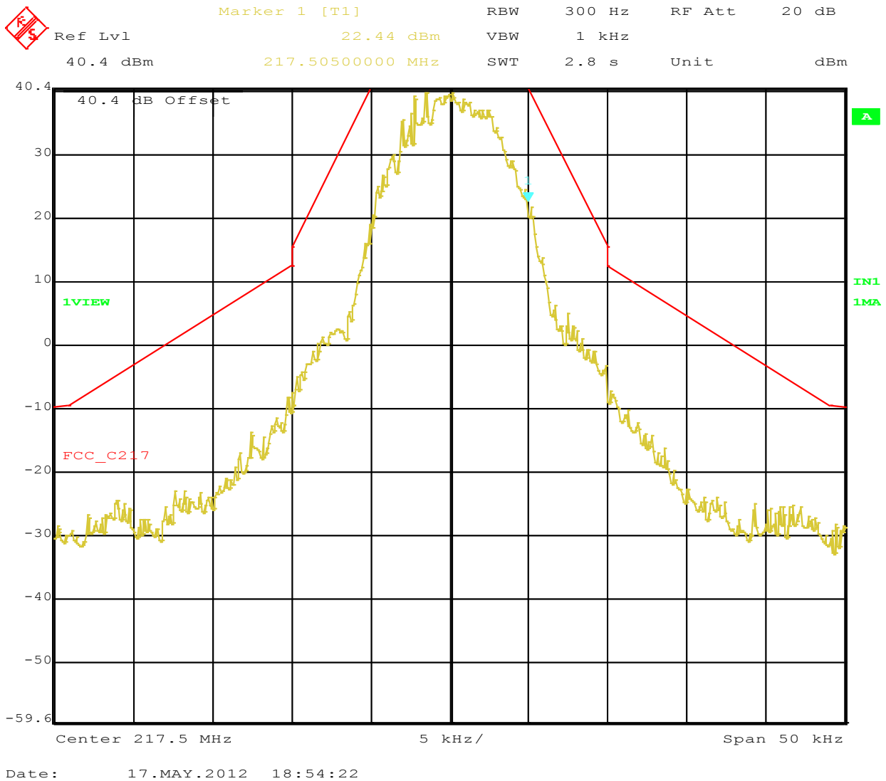
Figure 46: Emission mask C requirement at Operating Channel 217.5 MHz, GMSK
