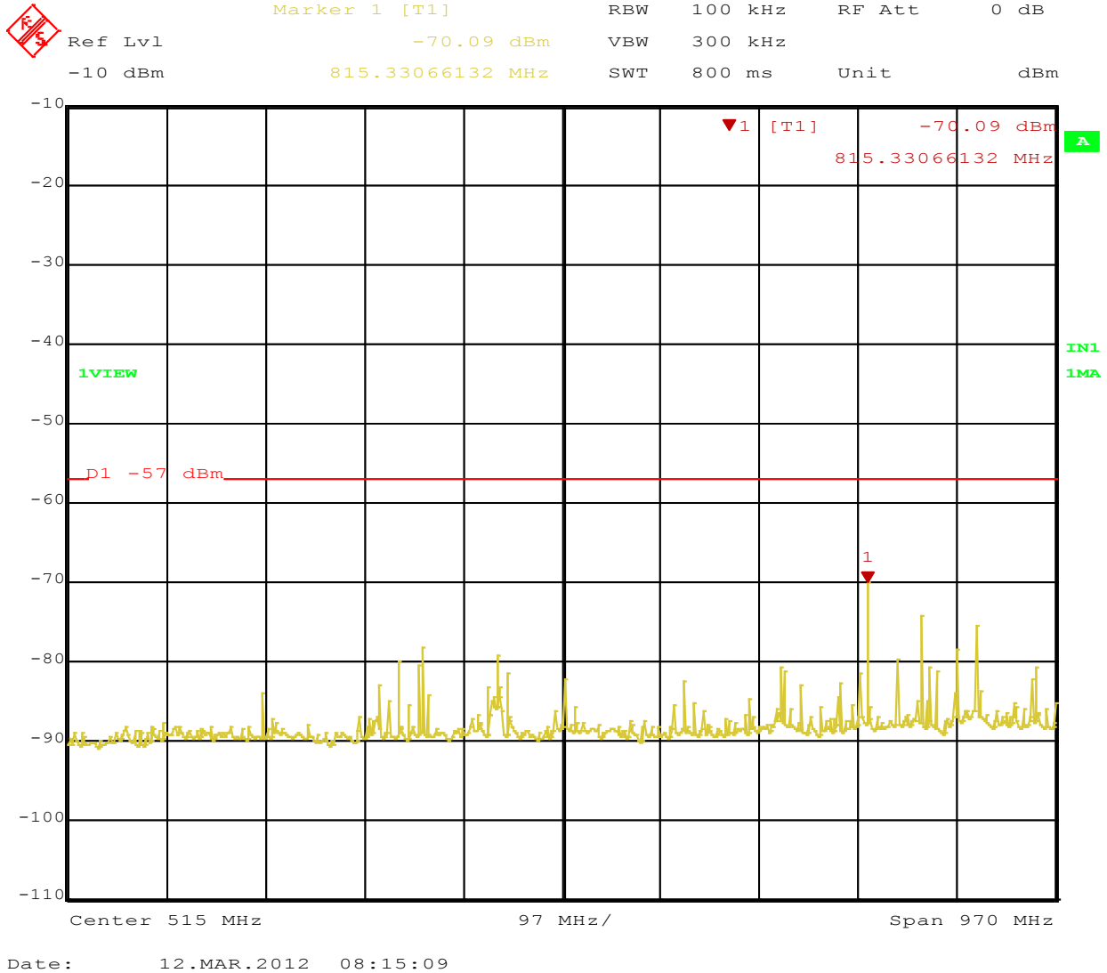
Figure 98: Out of Band Emissions Operating 220.9875 MHz Receive Mode
