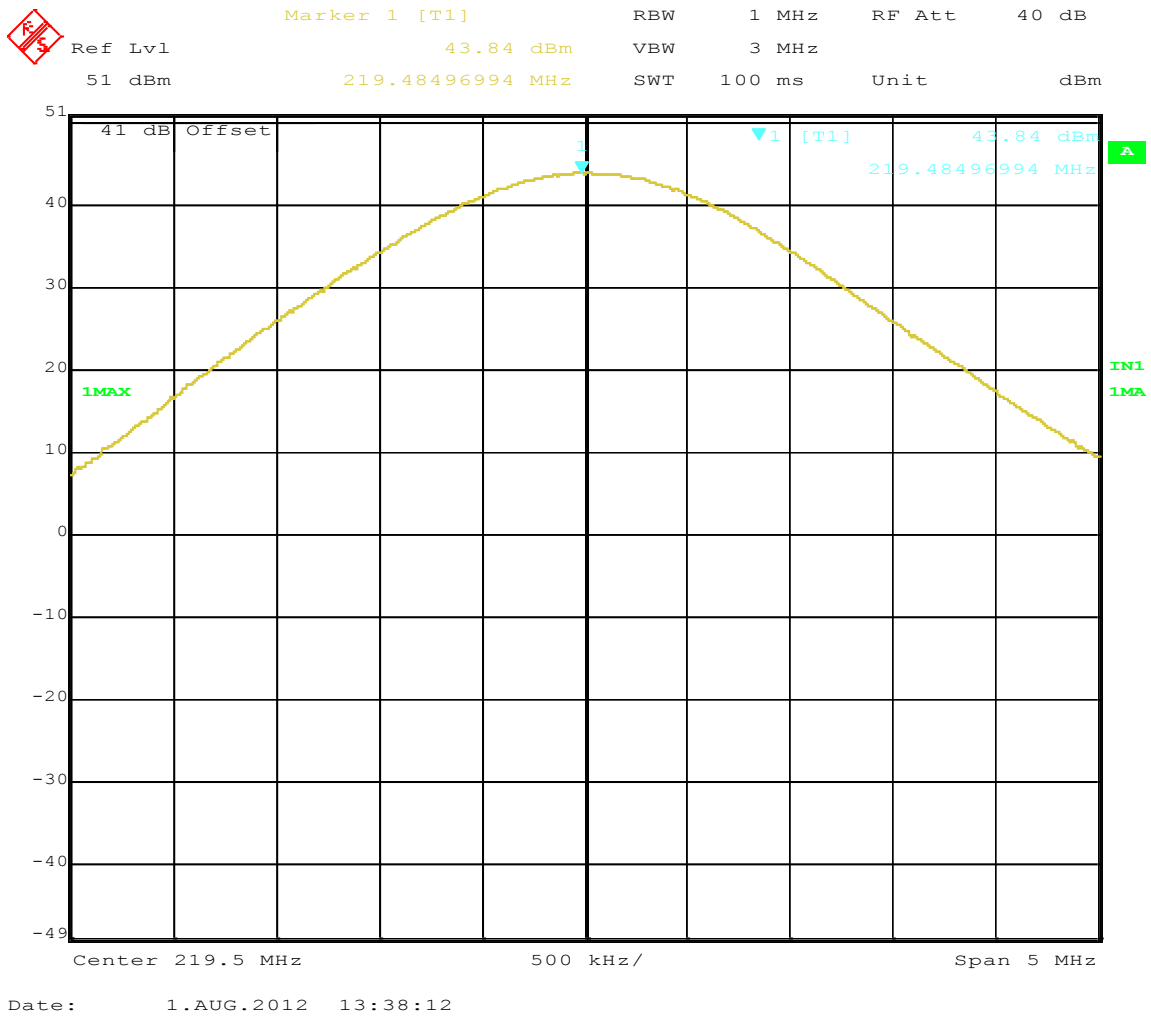
Figure 26: Maximum Transmitted Power, 219.5 MHz at 16 QPSK Power for Base Station and Mobile application
