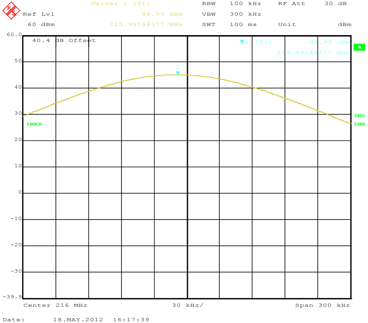
Figure 3: Maximum Transmitted Power, 216 MHz at 32 QPSK
