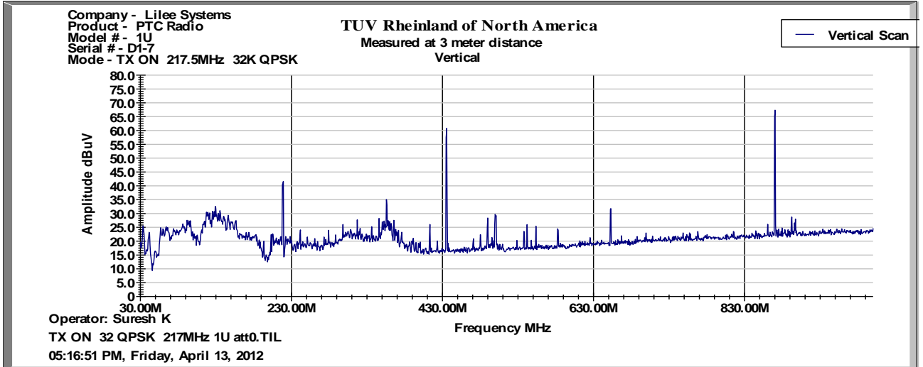
30 MHz to 1GHz Plot for Transmit Mode: 32 QPSK
