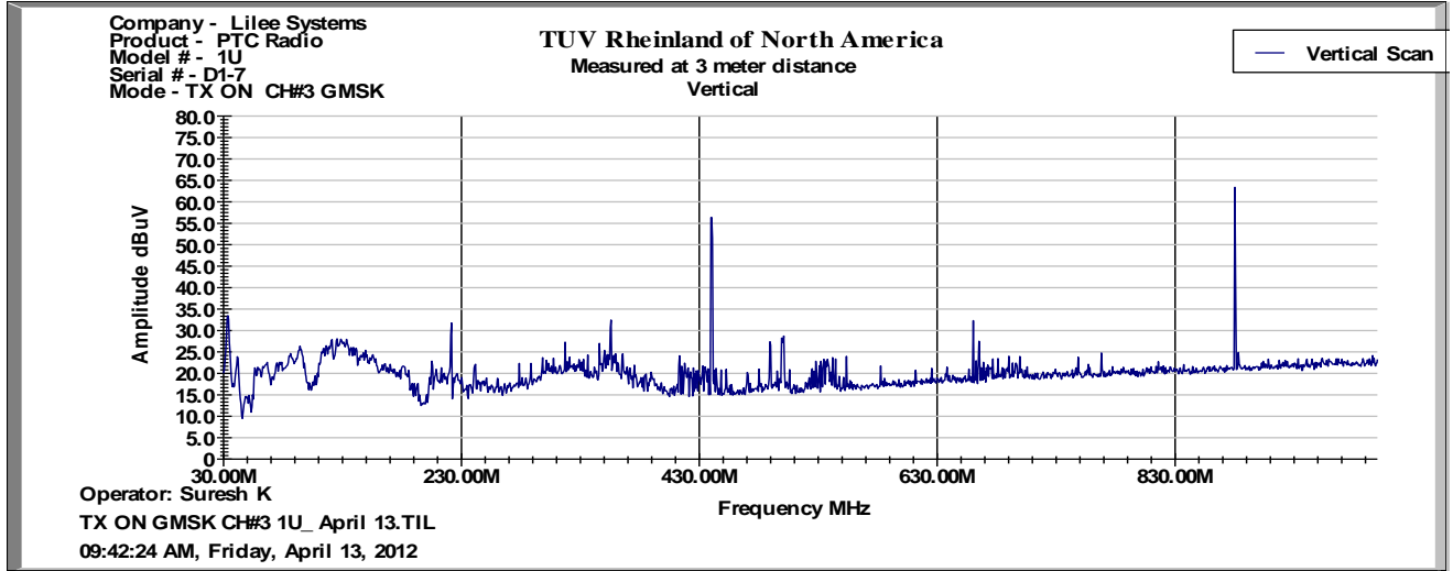
30 MHz to 1GHz Plot for Transmit Mode: 220.0125 MHz at GMSK
