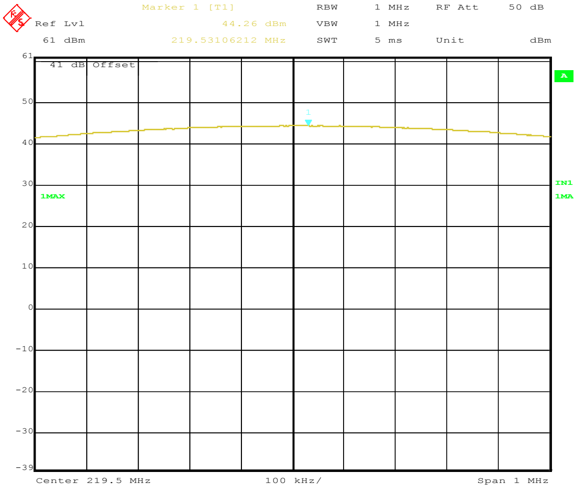
Figure 25: Maximum Transmitted Power, 219.5 MHz at GMSK Power for Mobile application
