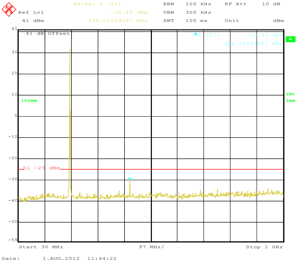
Figure 95: Out of Band Emissions Operating 219.5 MHz 32 QPSK Plot 1
