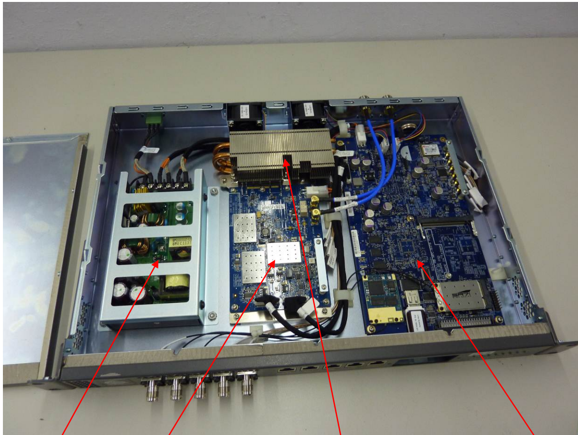
Power Supply
