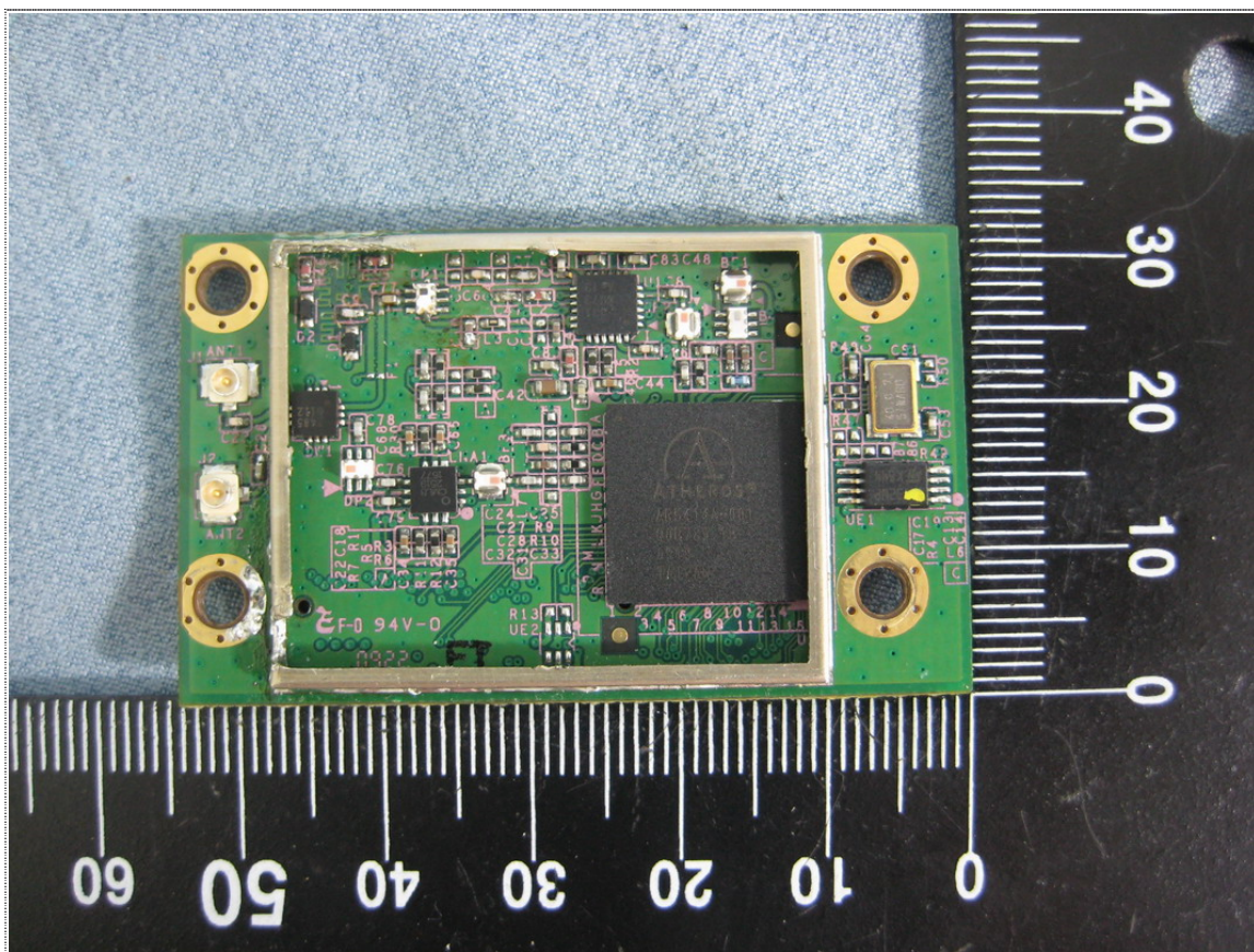
Front View of EUT-2
