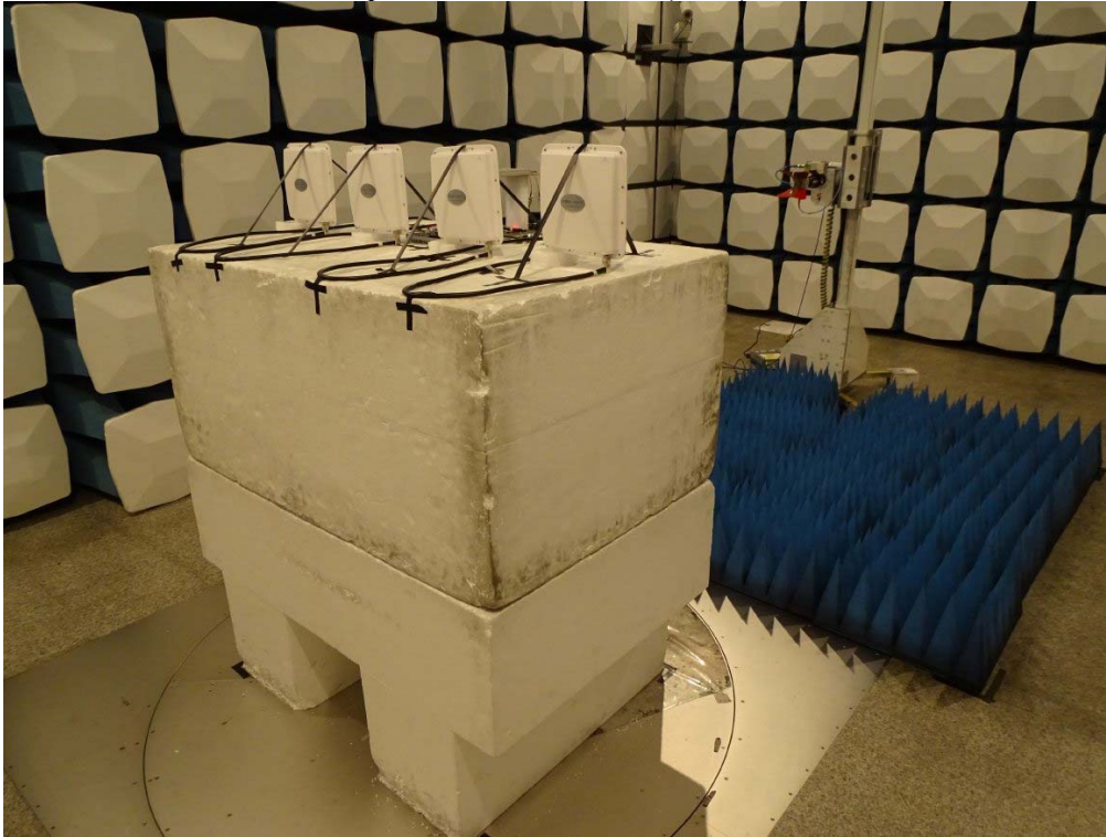
Front View of Spurious Emission Test (Horn)-Patch Antenna
