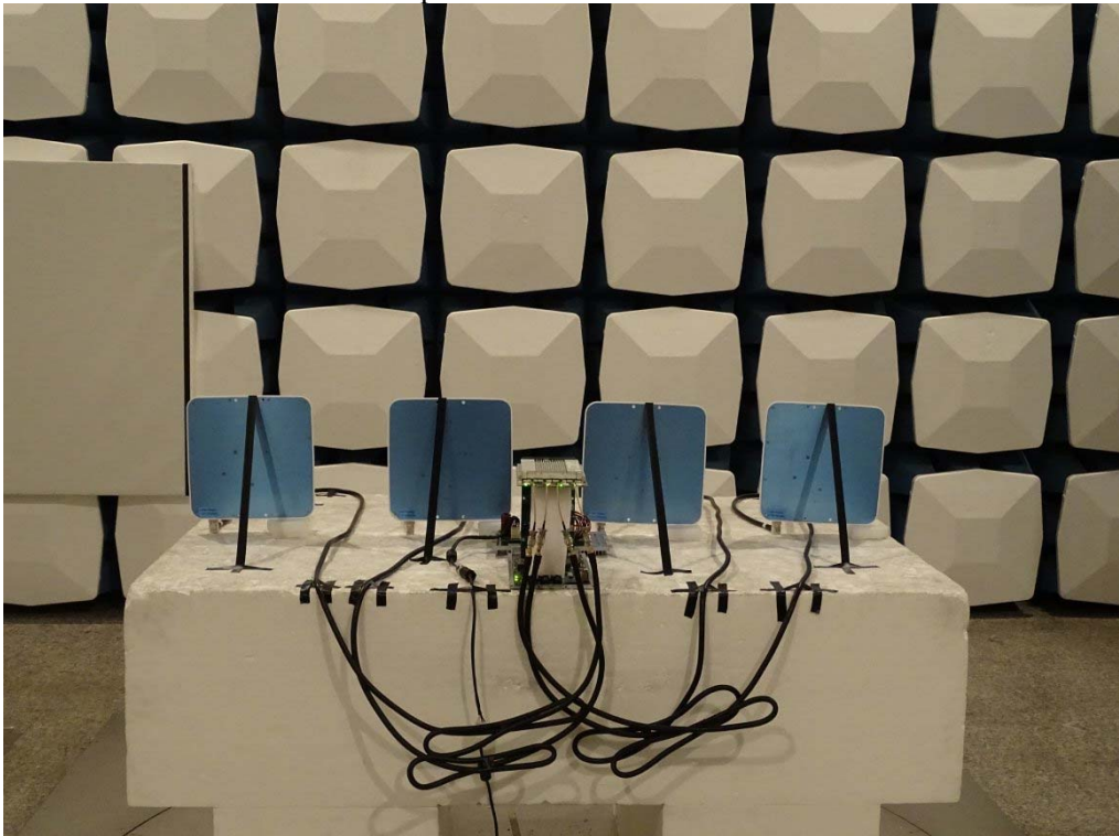
Back View of Spurious Emission Test-Patch Antenna
