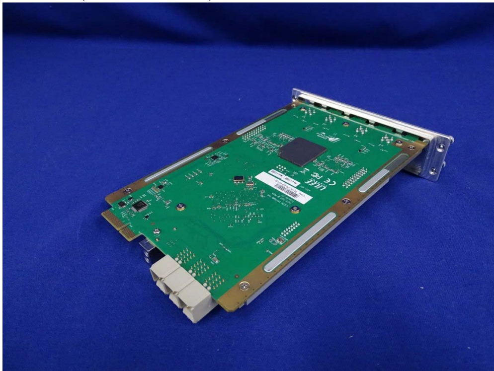
(18) EUT Photo (M/N: SM-SDR-2400)
