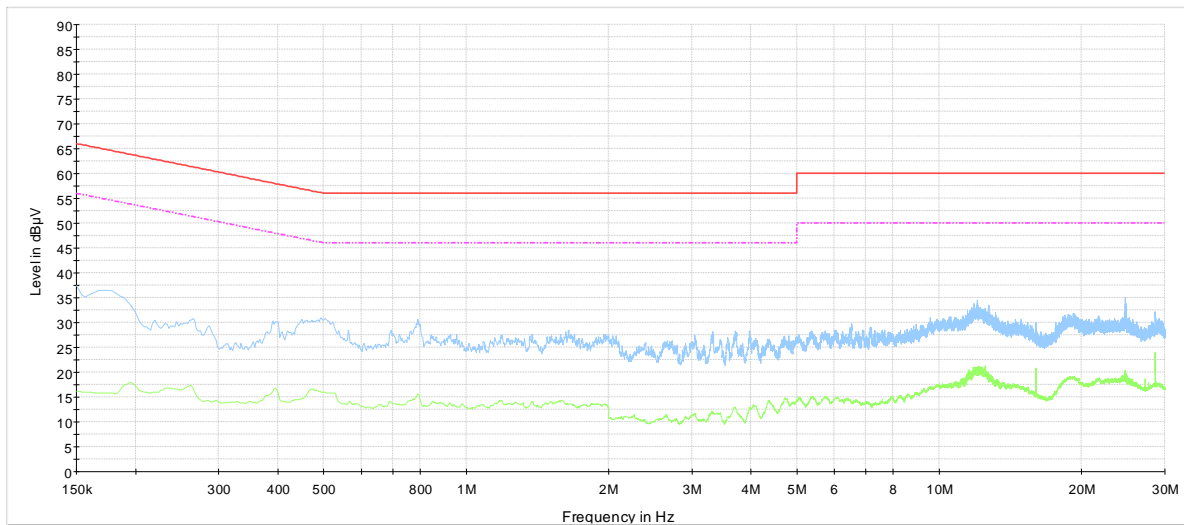
NEX-234511 120 Vac 60 Hz Neutral scan — CISPR 22 Mains QP Class B - - - CISPR 22 Mains AV Class B — Preview Result 1-PK+ — Preview Result 2-AVG
