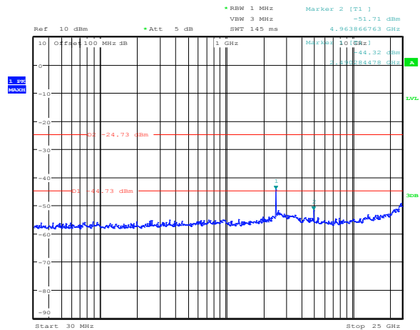
Figure 8.4-4: Conducted spurious emissions within restricted bands at low channel
