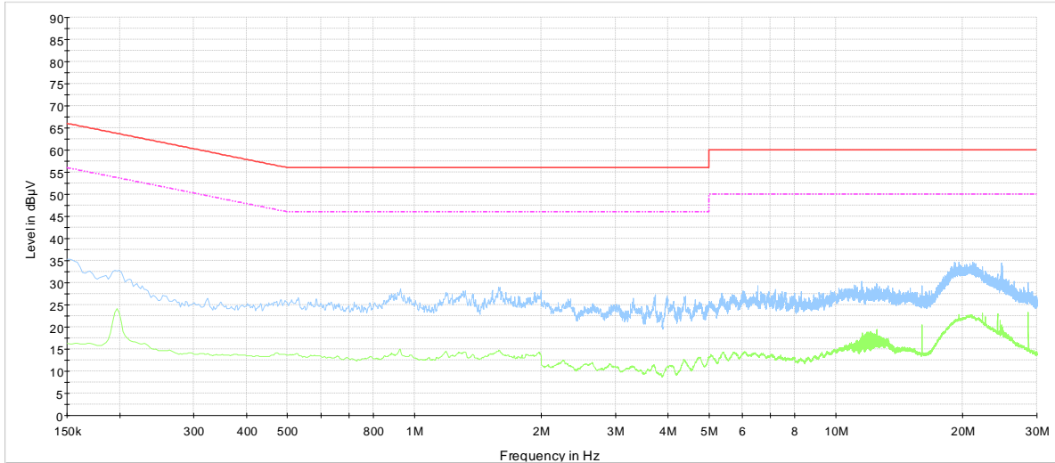
NEX-234511 120 Vac 60 Hz Phase scan — CISPR 22 Mains QP Class B - - - CISPR 22 Mains AV Class B — Preview Result 1-PK+ — Preview Result 2-AVG
