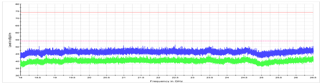
NEX-384022 - Jan 27, 2020 - BLE - High Channel AVG_MAXH PK_MAXH FCC 15.209 and RSS-210 limit line pk FCC 15.209 and RSS-210 limit line
