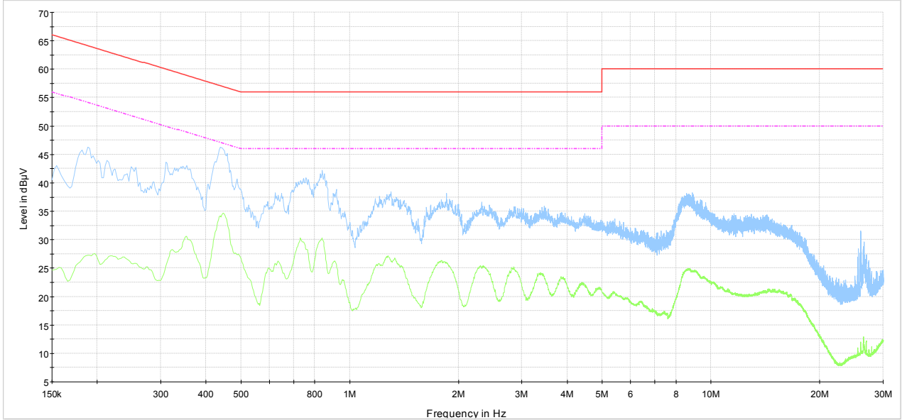
NEX-384022 - Nov 1, 2019 - 230 Vac - 50 Hz - Line - Wifi test mode Preview Result 2-AVG Preview Result 1-PK+ CISPR 32 Limit - Class B, Mains (Quasi-Peak) CISPR 32 Limit - Class B, Mains (Average)
