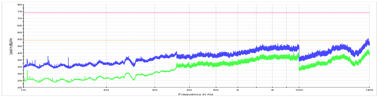
NEX-384022 - Dec 1, 2019 - Bluetooth - pi/4-DPSK Modulation - Mid Channel — AVG_MAXH — PKI_MAXH — FCC 15.209 and RSS-210 limit line pk - - - - - FCC 15.209 and RSS-210 limit line
