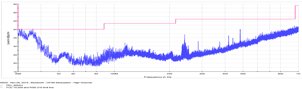
Figure 8.7-31: Radiated spurious emissions for high channel 30 MHz to 1 GHz
