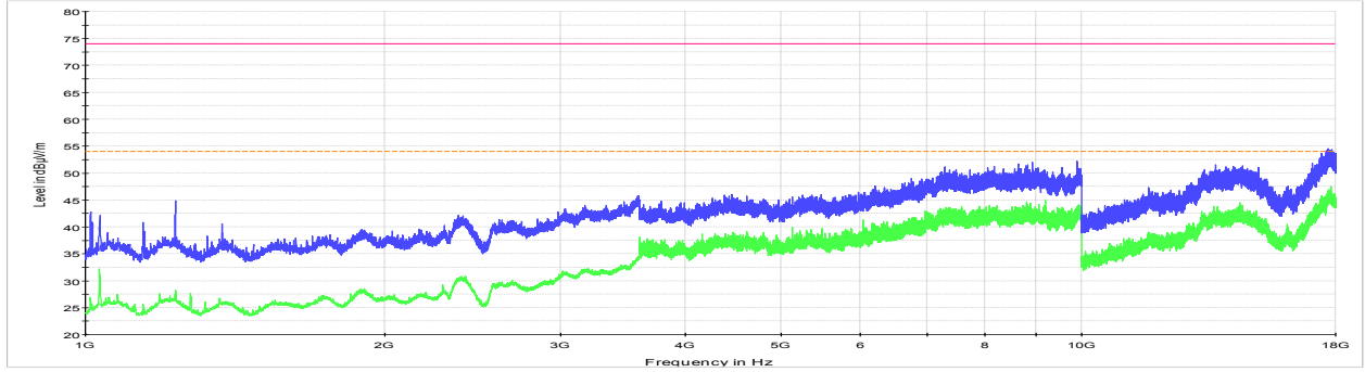
NEX-384022 - Dec 1, 2019 - Bluetooth - pi/4-DPSK Modulation - Low Channel — AVG_MAXH — PKI_MAXH — FCC 15.209 and RSS-210 limit line pk - - - - - FCC 15.209 and RSS-210 limit line
