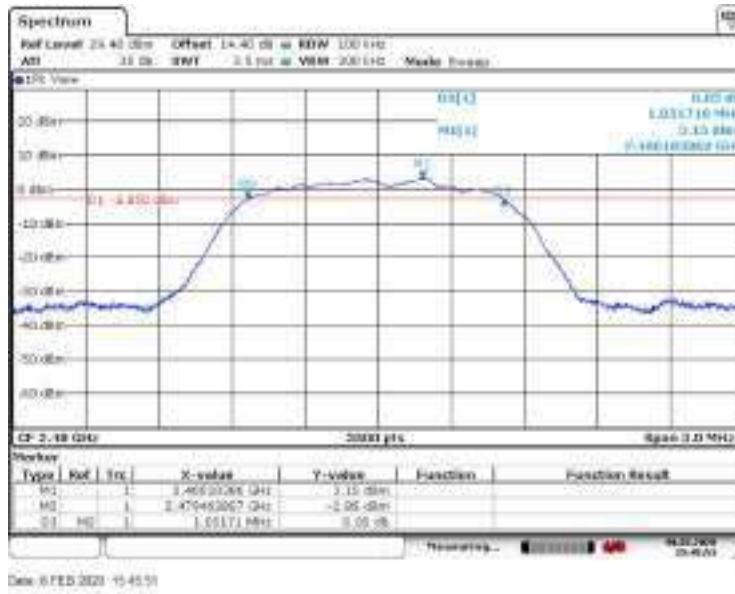
Figure 8.5-9: 6 dB bandwidth on high channel
