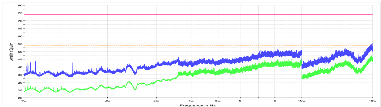
Figure 8.7-44: Radiated spurious emissions for low channel 1 GHz to 18 GHz
