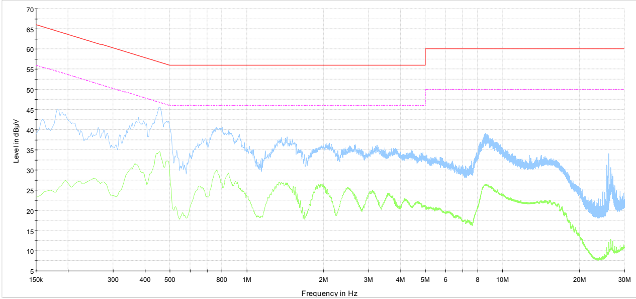
NEX-384022 - Nov 1, 2019 - 230 Vac - 50 Hz - Neutral - Wifi test mode Preview Result 2-AVG Preview Result 1-PK+ CISPR 32 Limit - Class B, Mains (Quasi-Peak) CISPR 32 Limit - Class B, Mains (Average)
