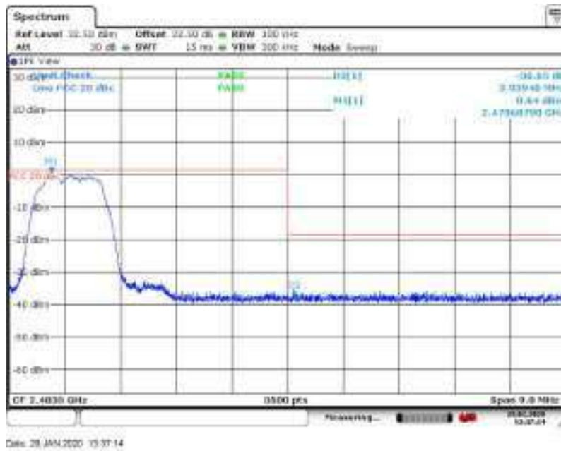
Figure 8.7-16: Band Edge emissions for high channel
