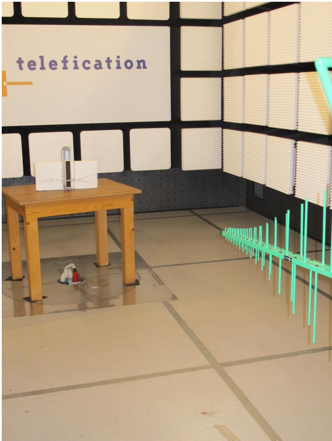
Photograph 2: Test setup radiated emissions (0.03 - 1 GHz)
