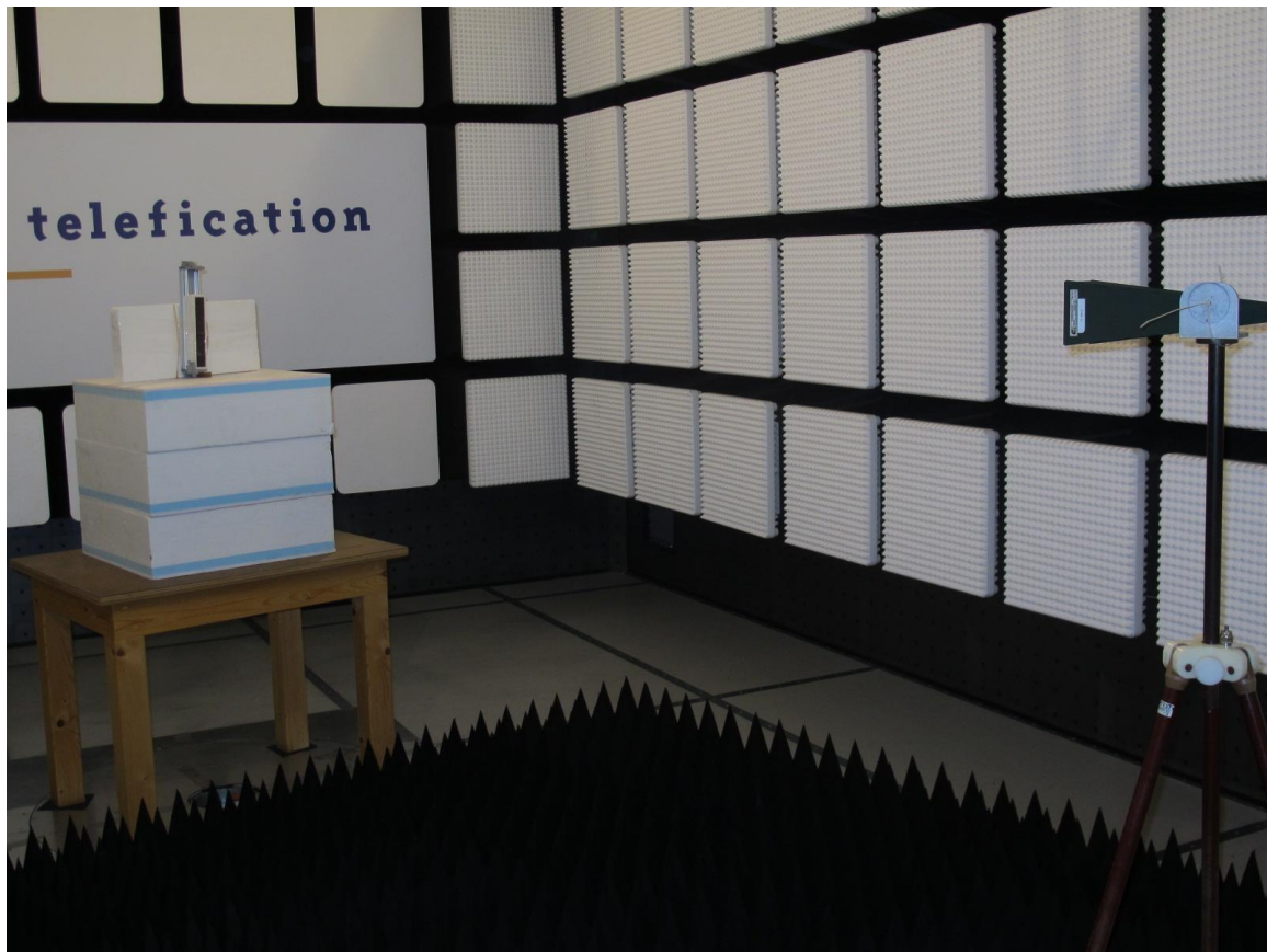
Photograph 4: Radiated emissions test set up 18 -26 GHz
