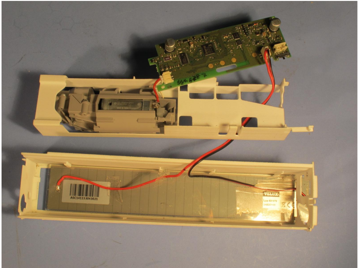
Photograph 2: 3SM S01 WW internal view 2
