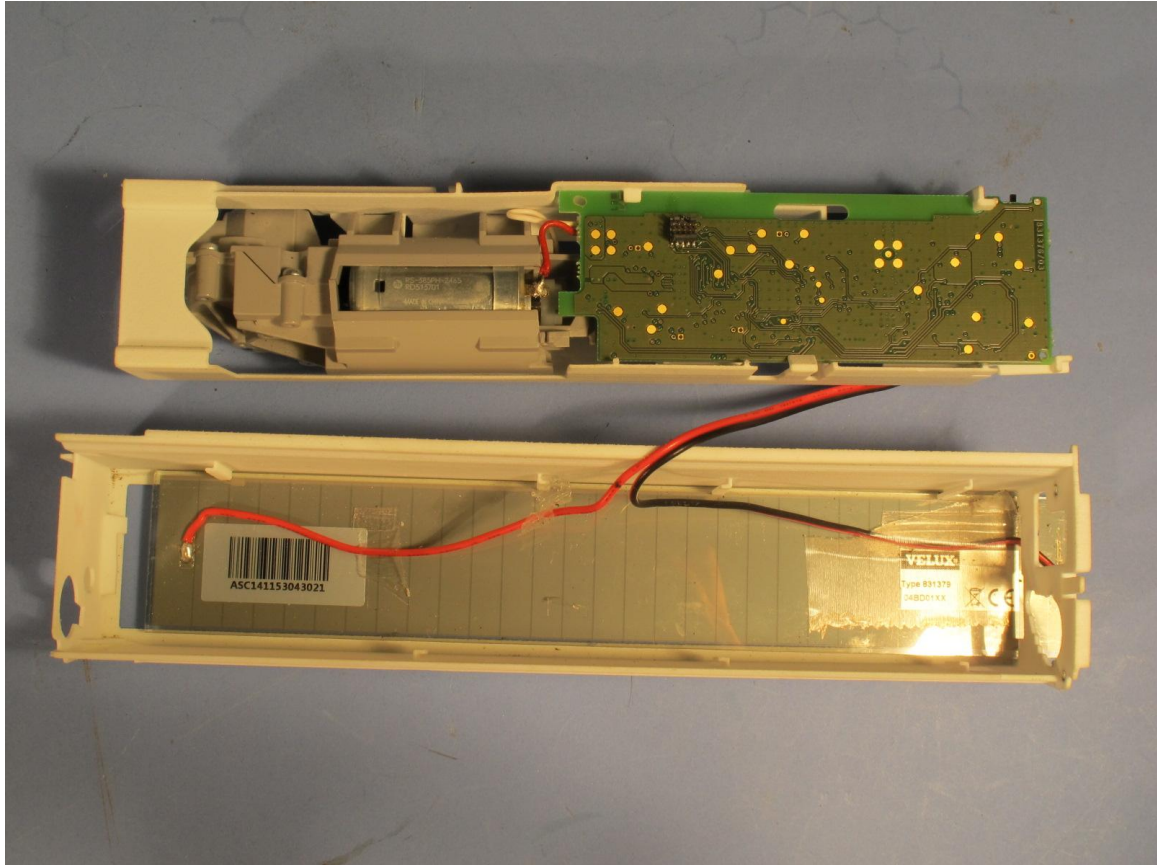
Photograph 1: 3SM S01 WW internal view1
