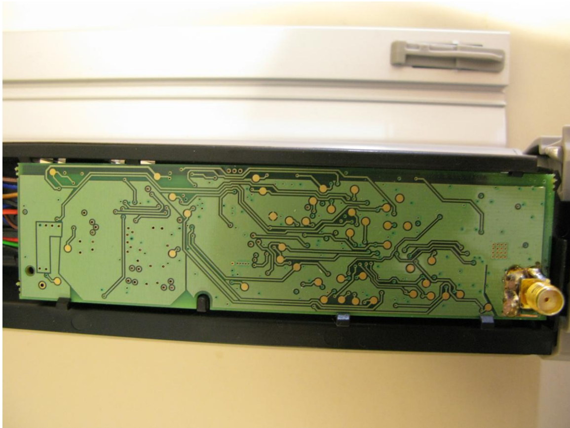
Photograph 3: PCB bottom view and temporary antenna connector
