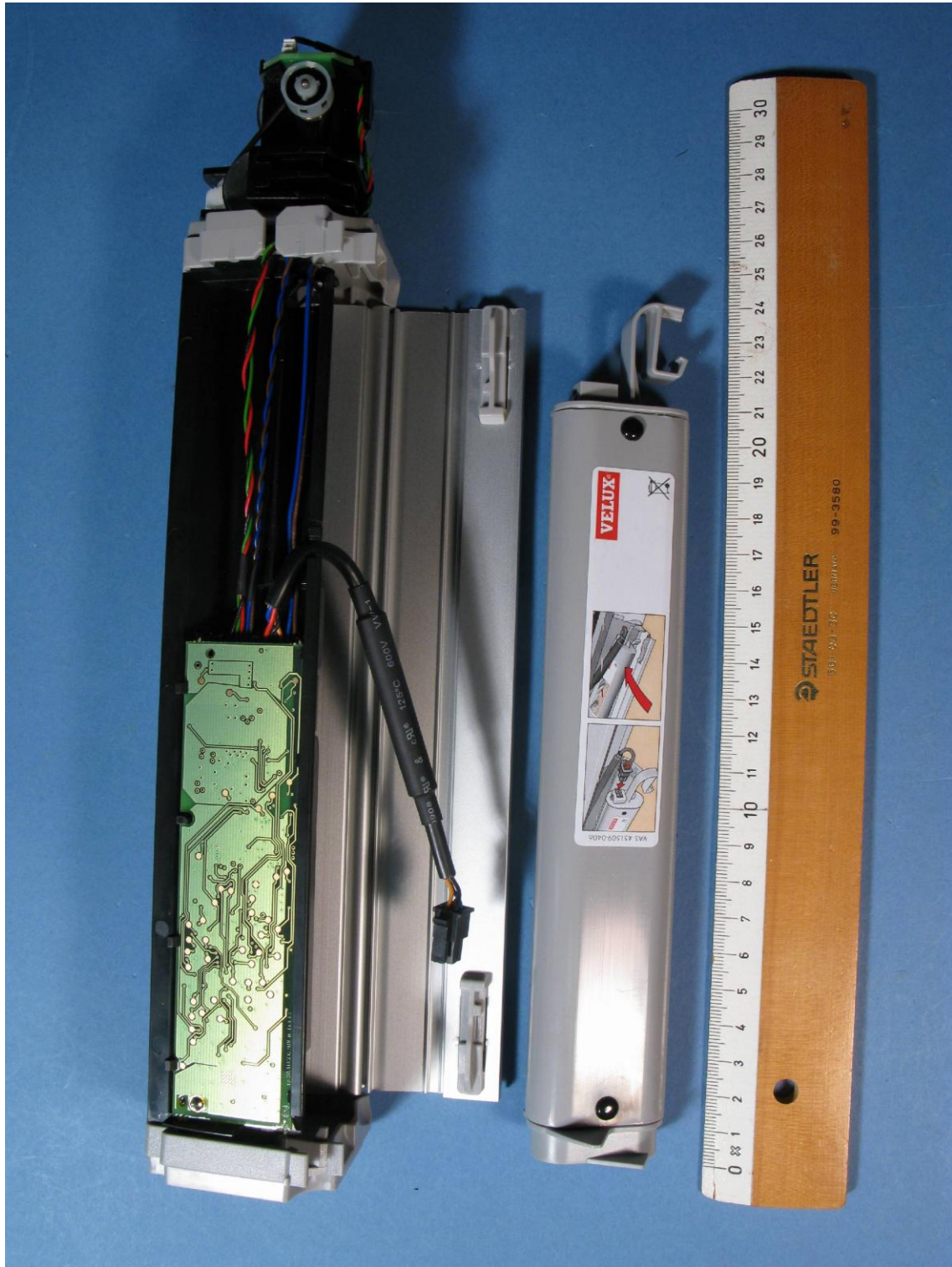
Photograph 1: Internal view, NiMH battery removed
