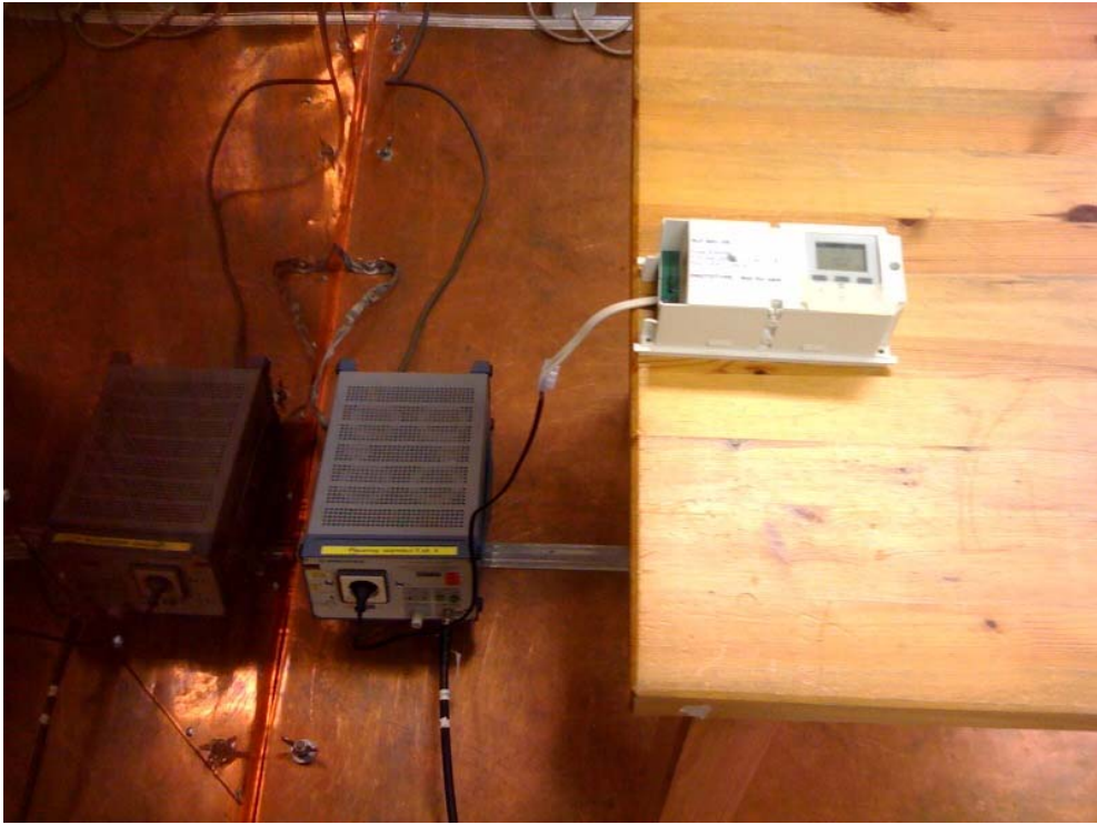
Conducted emission from AC-mains
