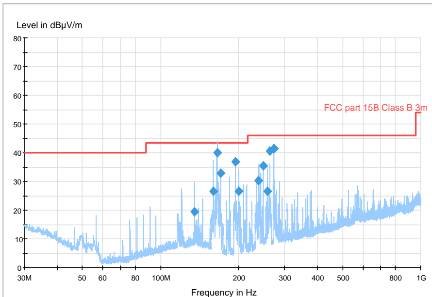
FCC 30 - 1000 MHz FCC class B 3m Fast scan
