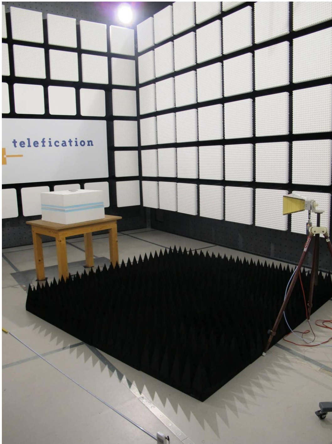
Photograph 3: - 2014-RC003-02, test setup radiated emissions (1 - 26 GHz)
