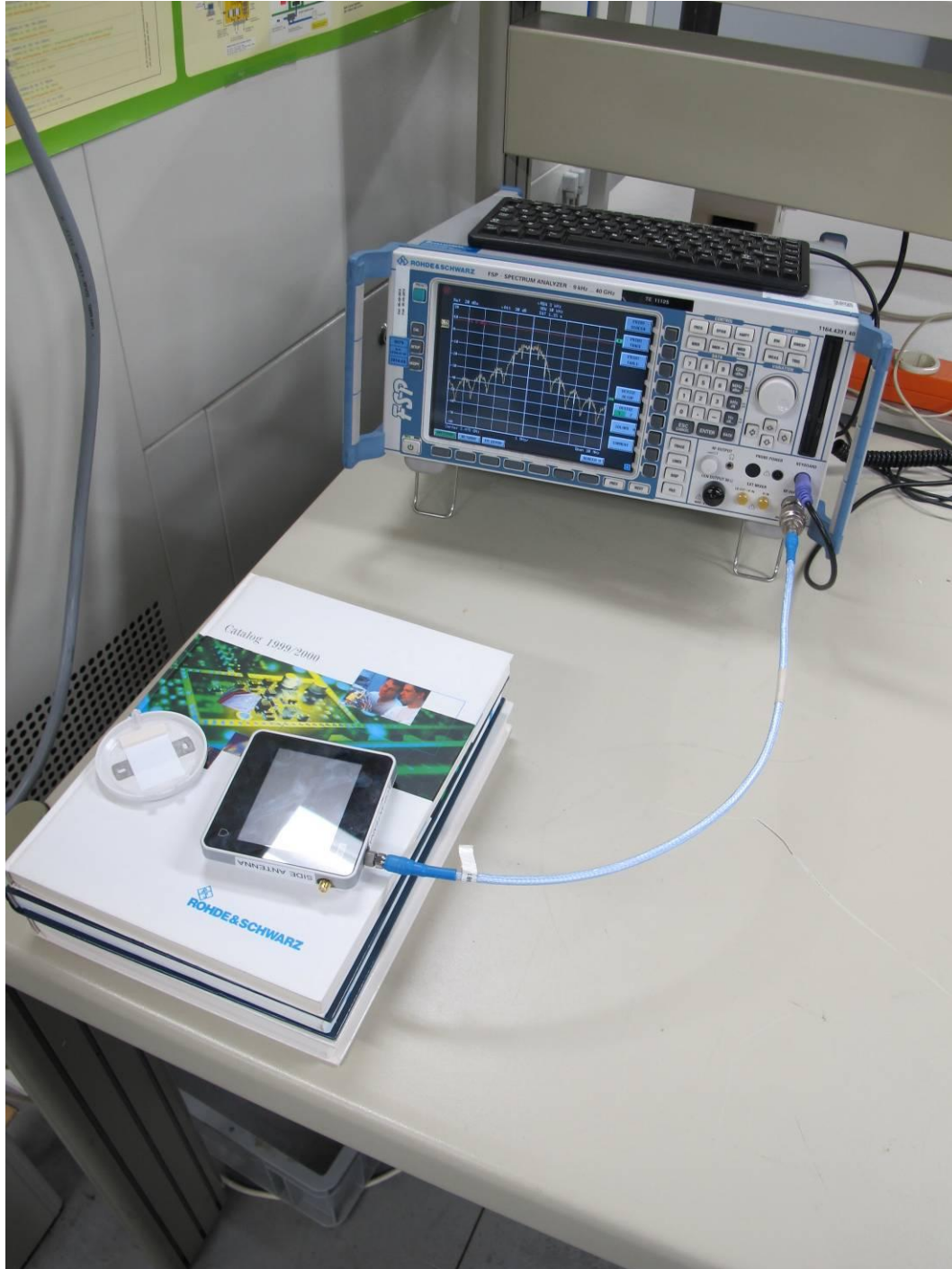
Photograph 1: - 2014-RC003-02, test setup conducted RF measurements
