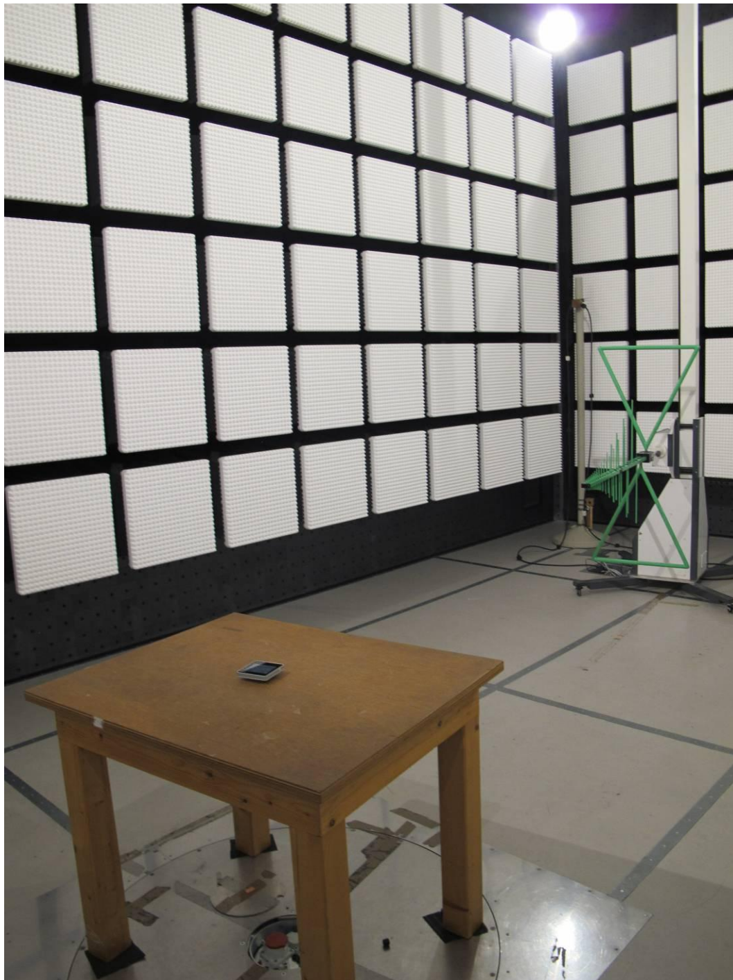
Photograph 2: - 2014-RC003-02, test setup radiated emissions (30 - 1000 MHz)
