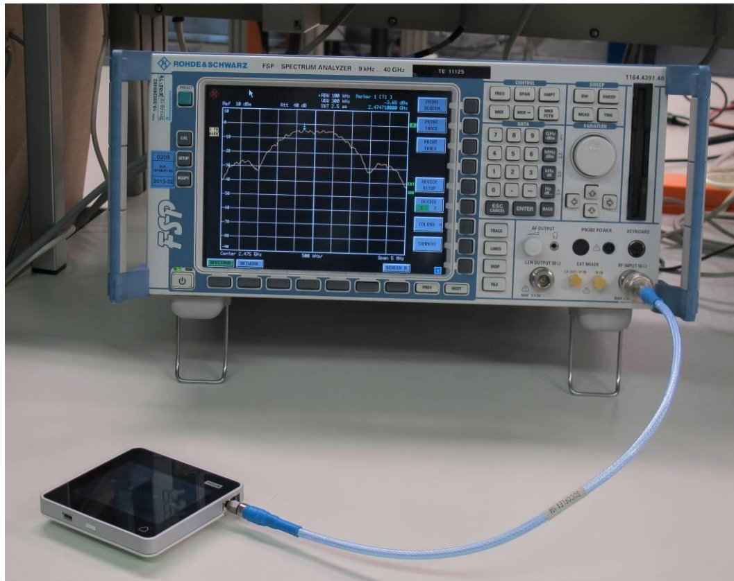
Photograph 1: - 3LR A02 US, test setup conducted RF measurements
