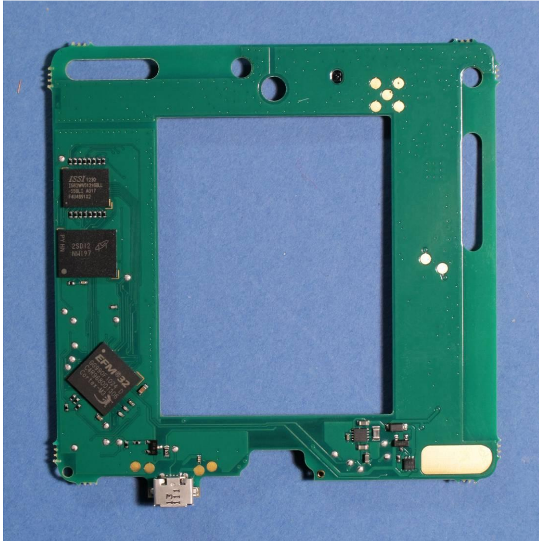
Photograph 4: - Velux 3LR A02 US; PCB bottom view
