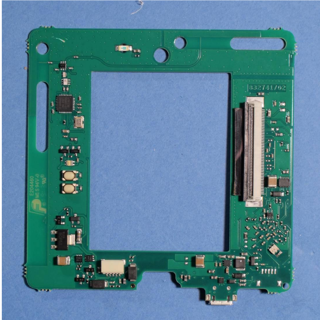
Photograph 3: - Velux 3LR A02 US; PCB top view
