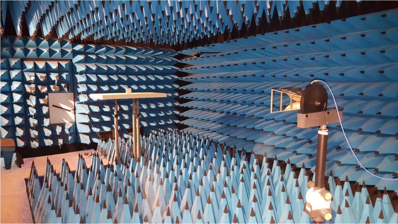
Radiated emissions measurements setup
