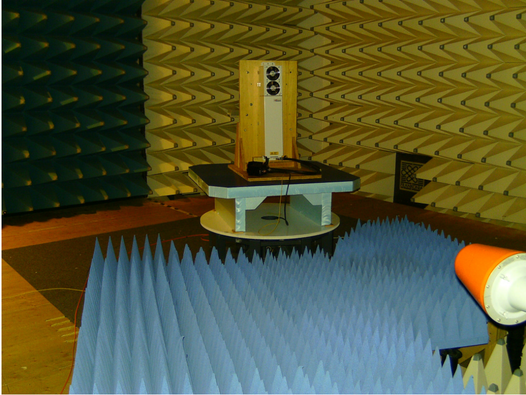
Test setup 1 GHz to 18 GHz
