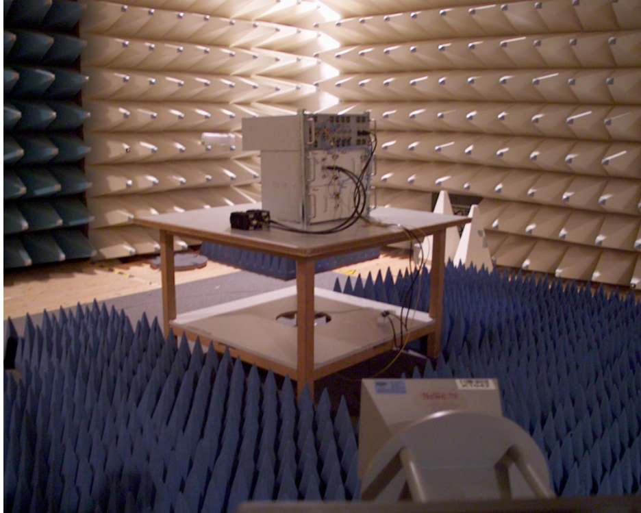
Measurement of radiated spurious emission (18 GHz to 24 GHz)
