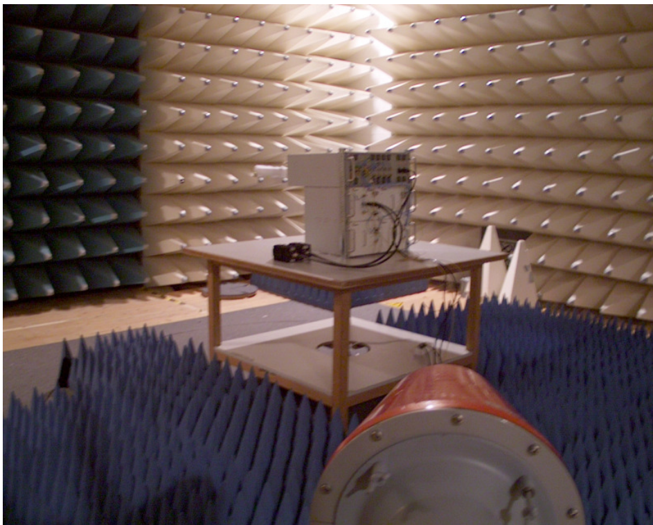
Measurement of radiated spurious emission (1 GHz to 18 GHz)
