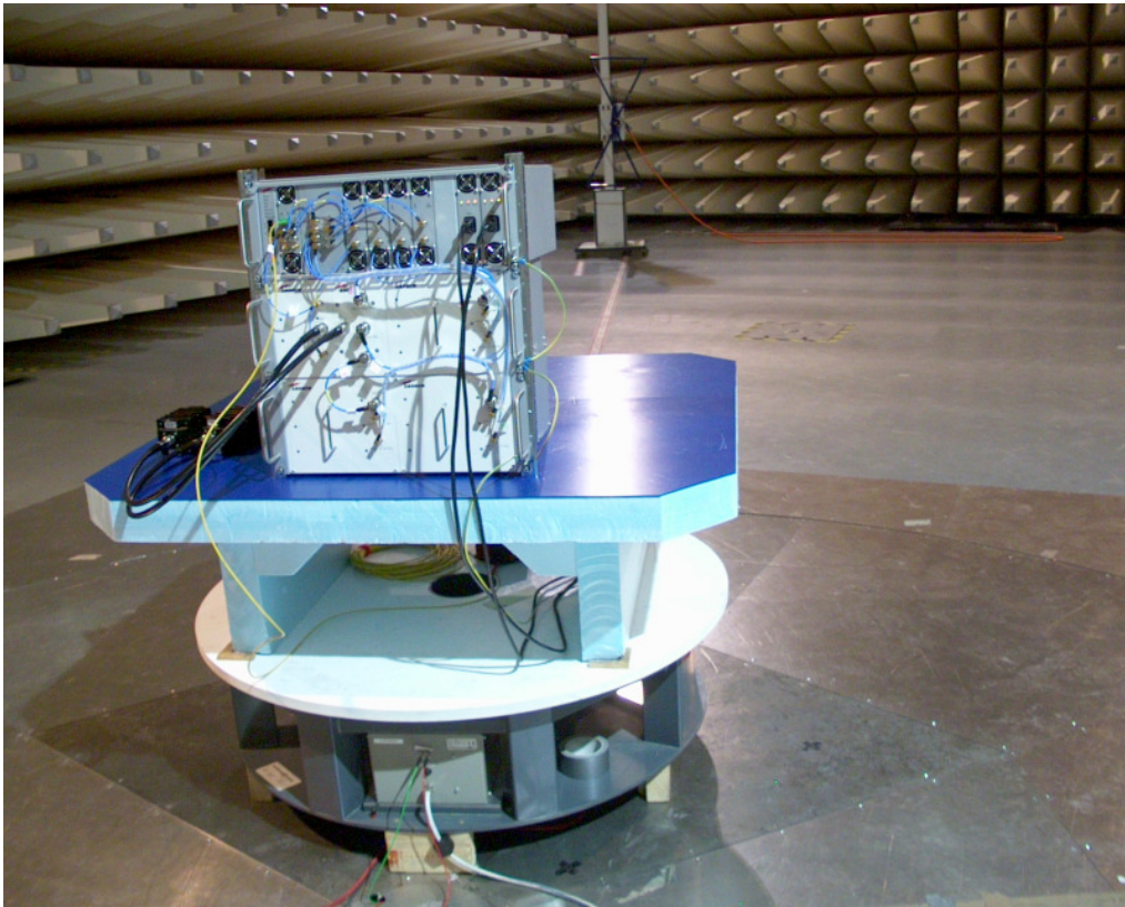
Measurement of radiated spurious emission (30 MHz to 1 GHz)
