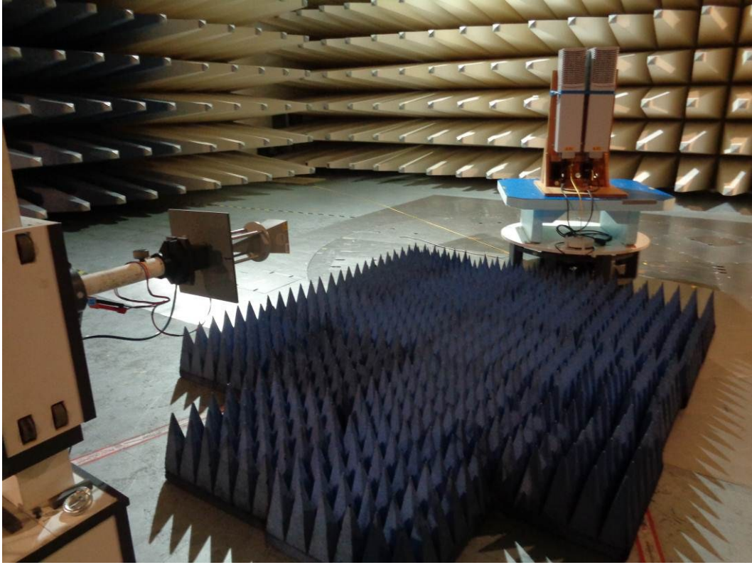
Test setup: Field Strength Emission 18-26 GHz @3m in the SAC (MIMO – RU + EU)
