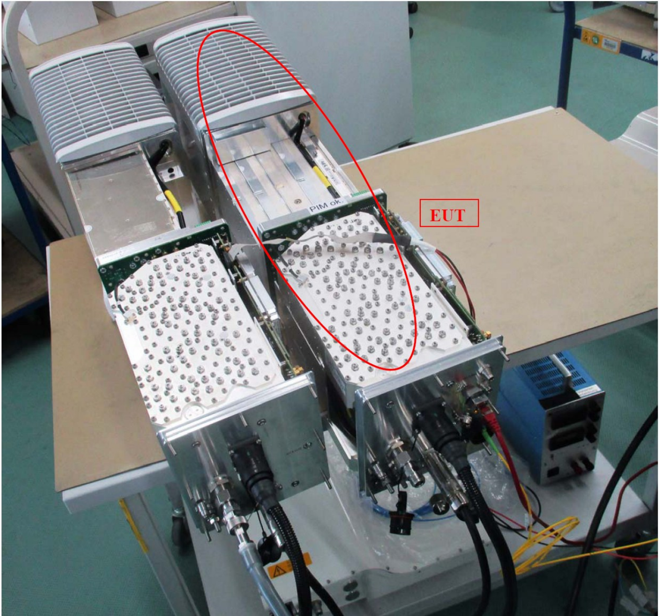
EUT ION-U H 7P/80-85P/17EP/19P & Auxiliary ION-U EU H 7P/80-85P/17EP/19P FCC ID: XS5-UH7817E19P FCC ID: XS5-UEUH7817E19P
