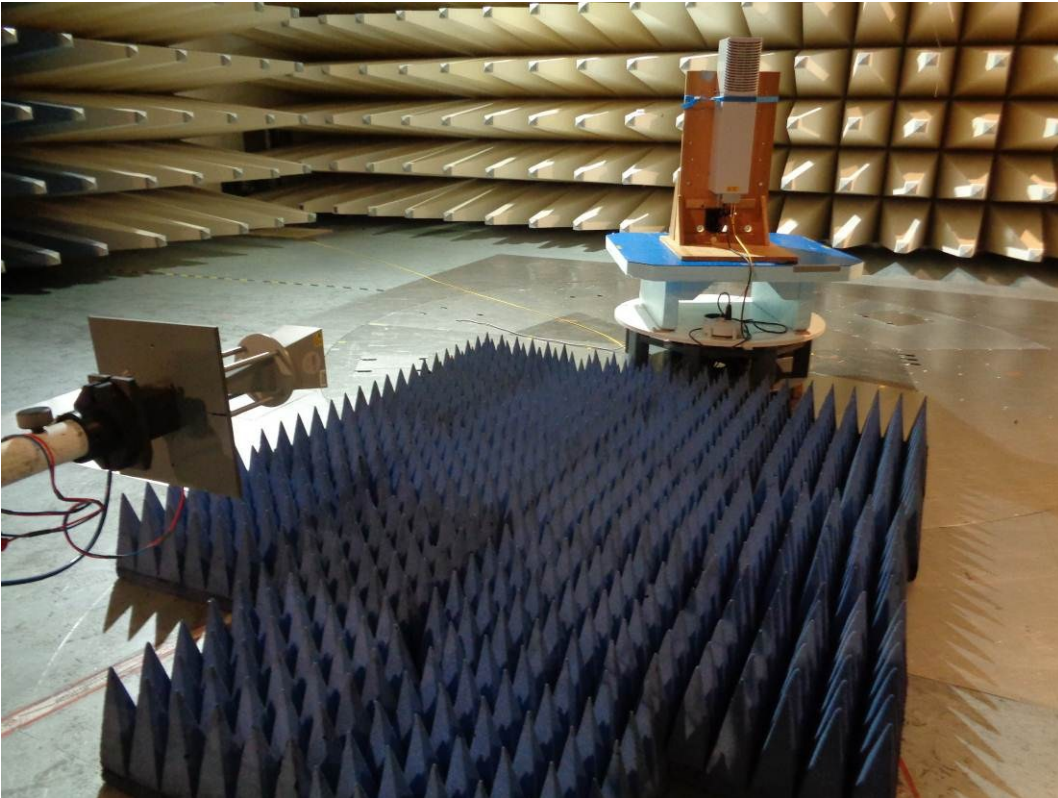
Test setup: Field Strength Emission 18-26 GHz @3m in the SAC (RU only)
