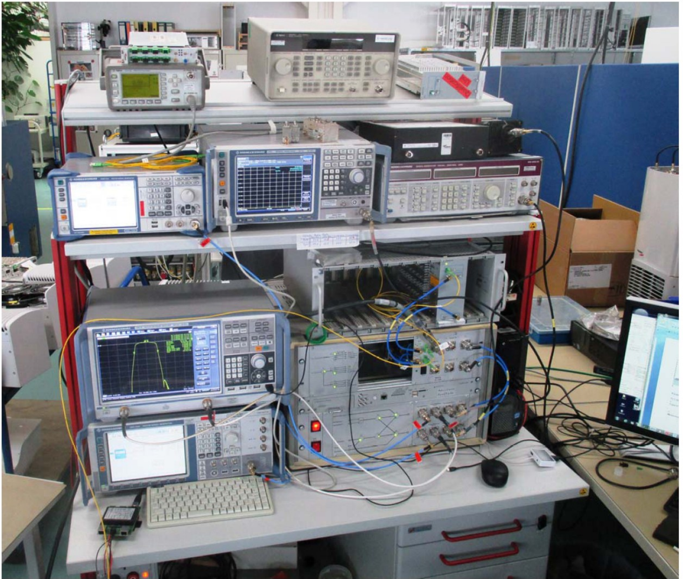
Measurement Equipment
