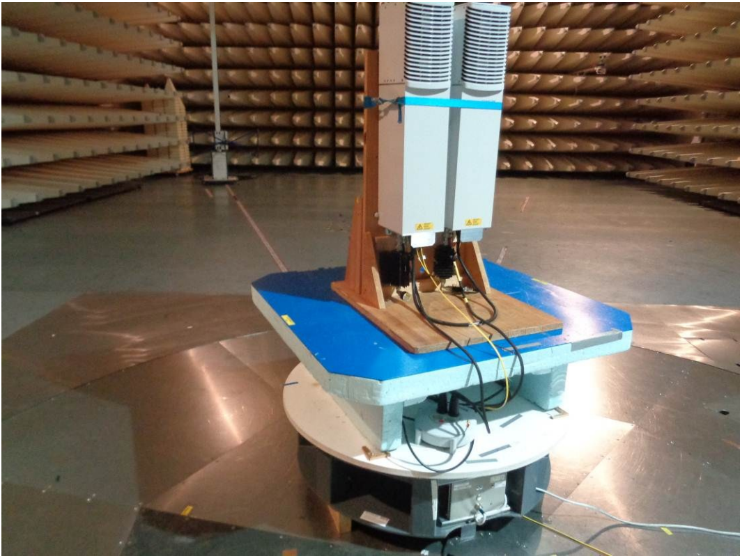
Test setup: Field Strength Emission 30 MHz - 1 GHz @10m in the SAC (MIMO – RU + EU)
