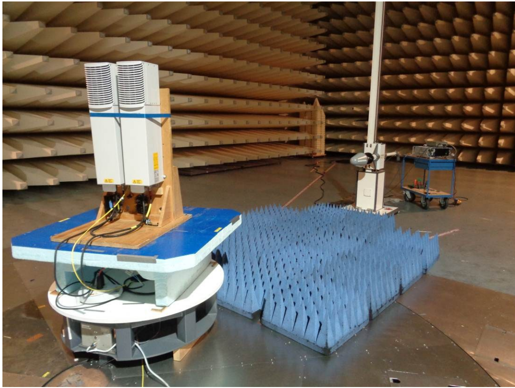
Test setup: Field Strength Emission 1-18 GHz @3m in the SAC (MIMO – RU + EU)
