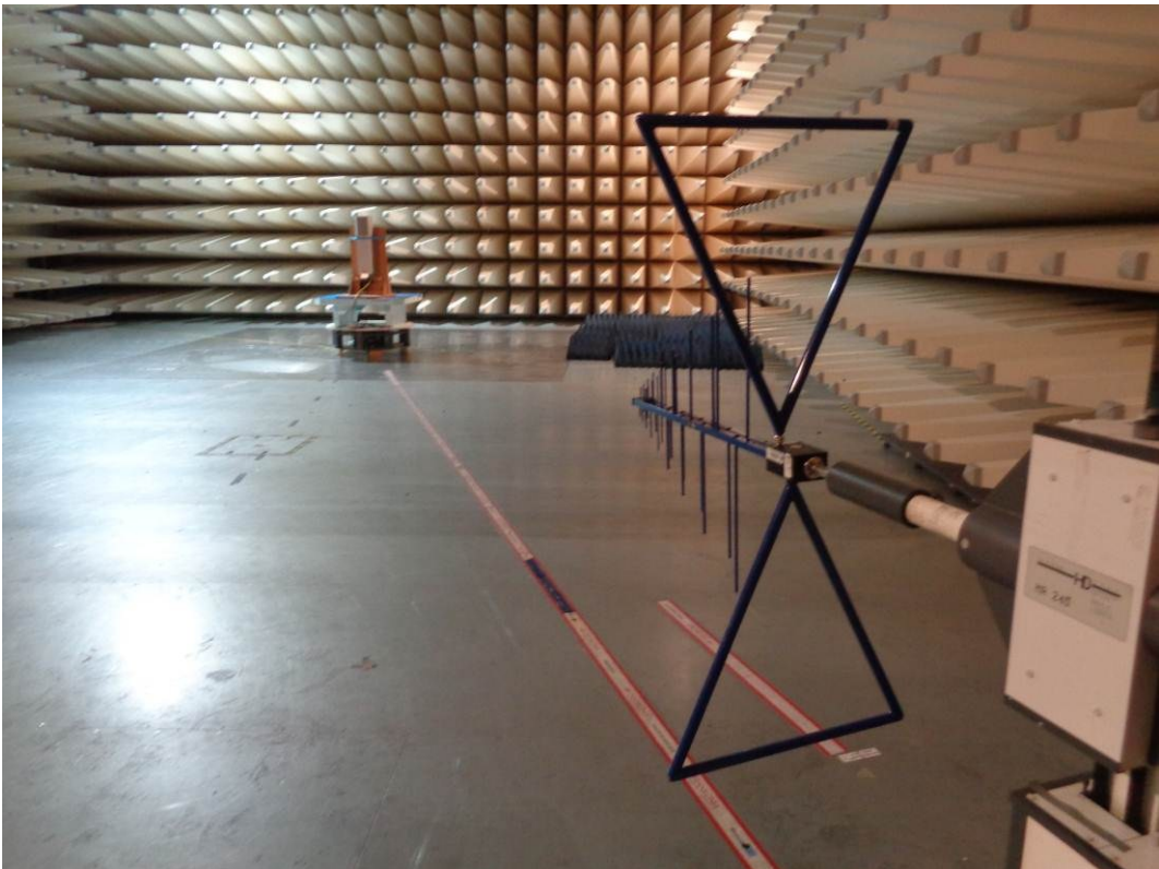
Test setup: Field Strength Emission 30 MHz - 1 GHz @10m in the SAC (RU only)
