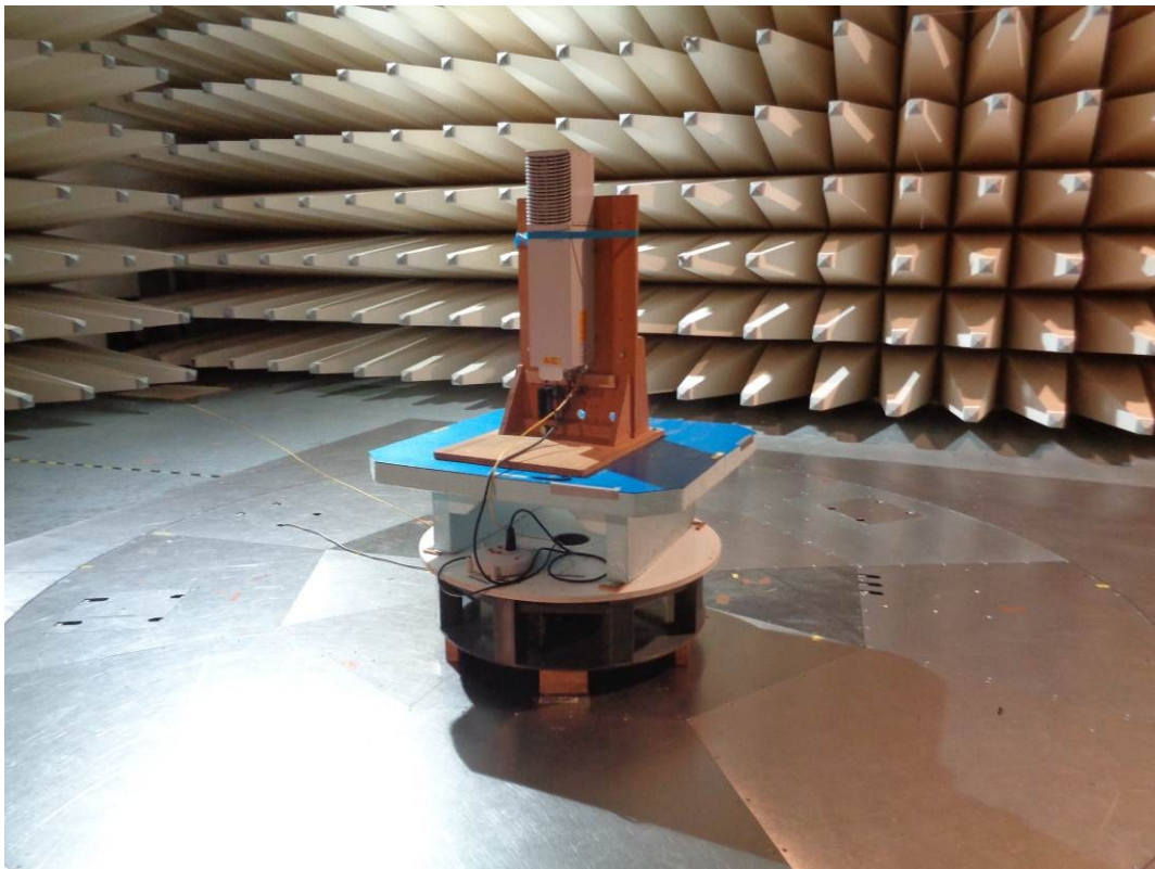
Test setup: Field Strength Emission 1-18 GHz @3m in the SAC (RU only)
