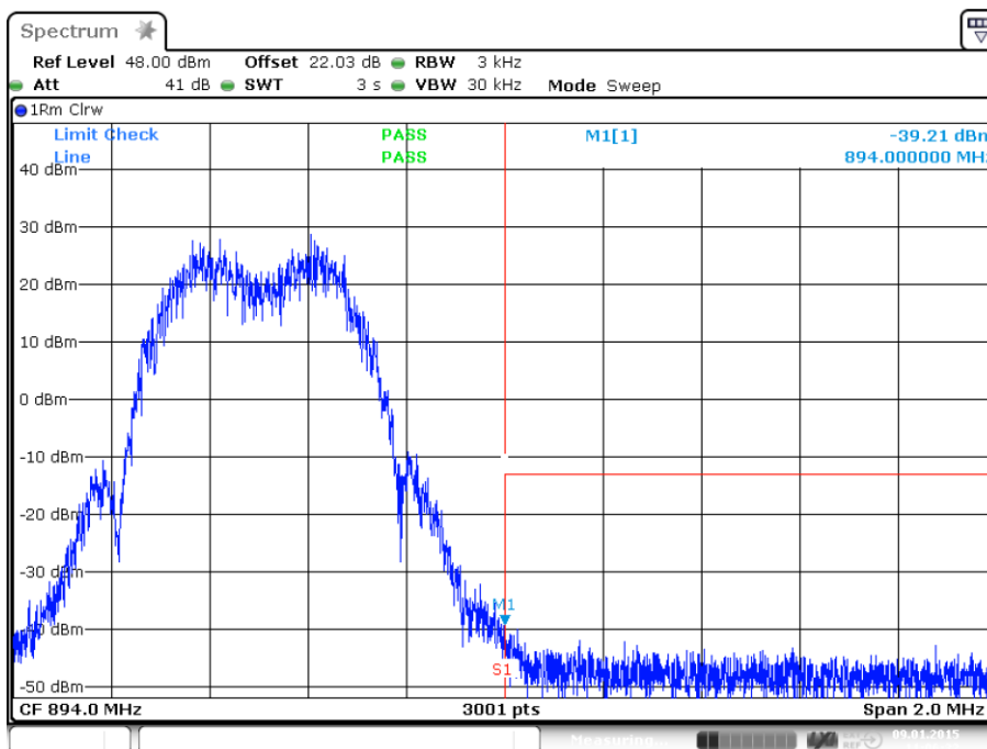
plot 8.3.1.2-#2 Intermodulation: §22.917, §2.1051; Test results; Downlink; EDGE Upper Band Edge
