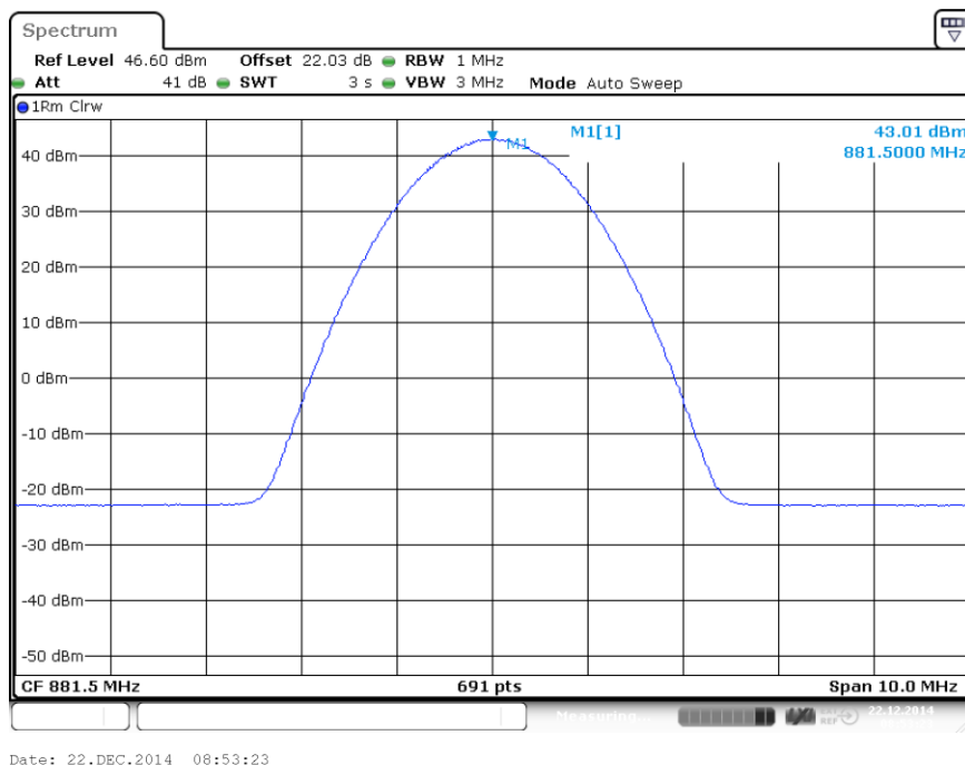
plot 5.3.1.2-#1 RF Power Out: §22.913, §2.1046; Test Results; Downlink; EDGE Middle
