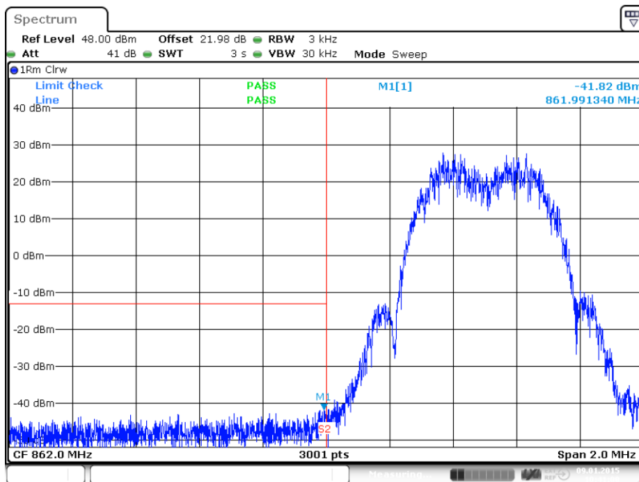
plot 8.3.1.2-#1 Intermodulation: §90.691, §2.1051; Test results; Downlink; EDGE Lower Band Edge
