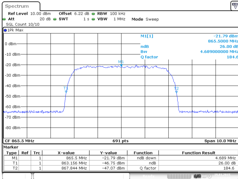
plot 6.3.2.4-#2 Occupied Bandwidth: §90.210, §2.1049; Test results; 26dB Bandwidth; WCDMA Input
