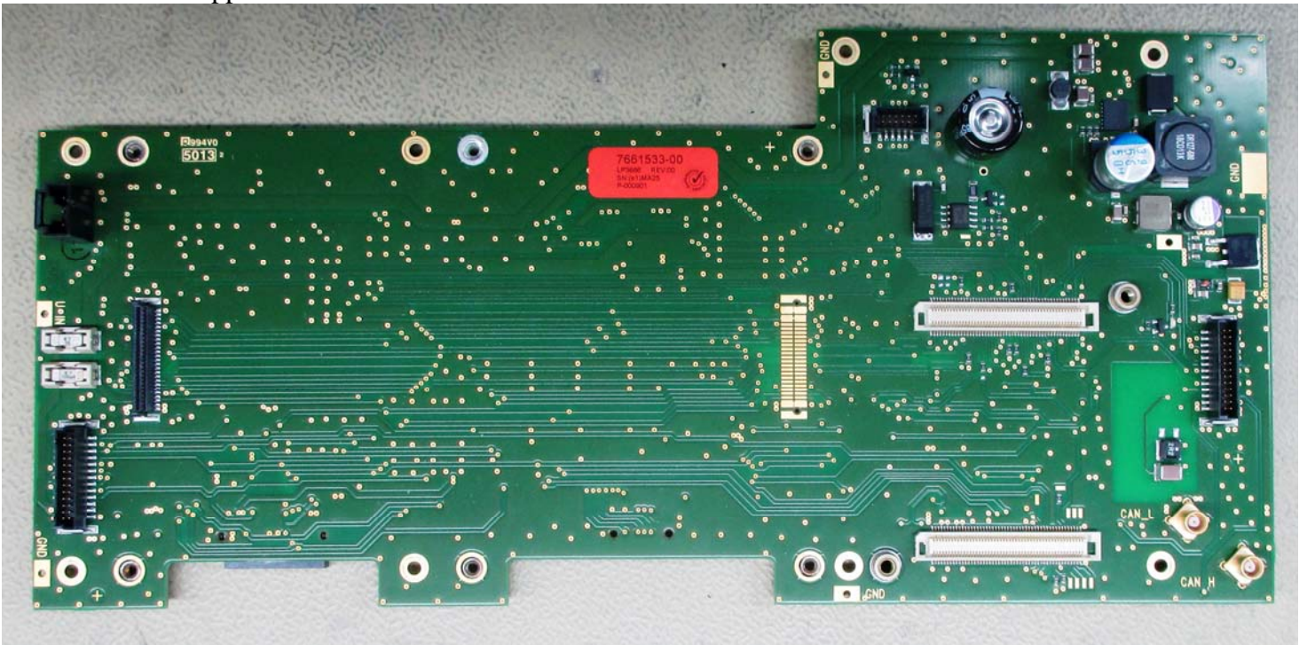
PCB P3686 RU-Application board M2 Cab 7661533-00
