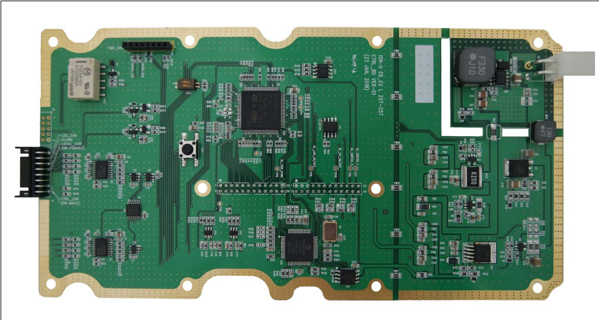
PCB TLCTRL-FMU (Top)
