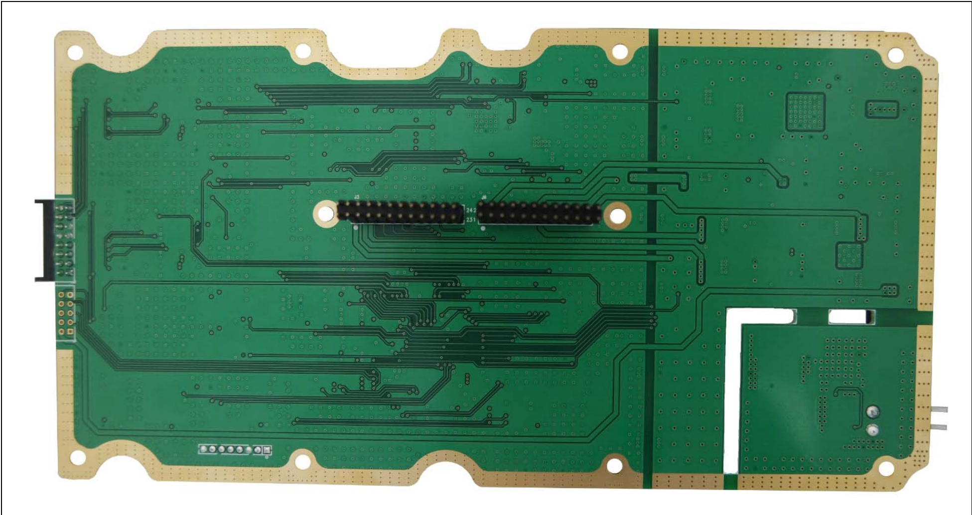
PCB TLCTRL-FMU (Bottom)
