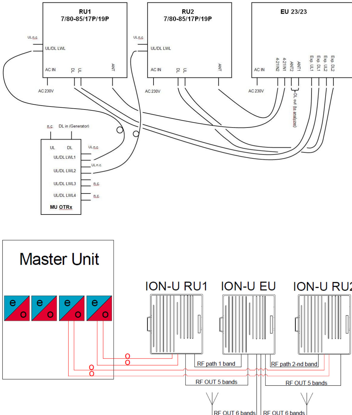
picture 8.3: Test configuration
