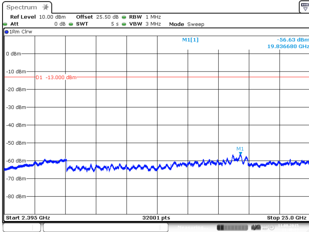
plot 7.3.1.1-#6 Spurious Emissions at Antenna Terminals: §27.53, §2.1051; Test results; Downlink; LTE; 2 x 5 MHz signal; 2.395 GHz – 25 GHz; carrier notched
