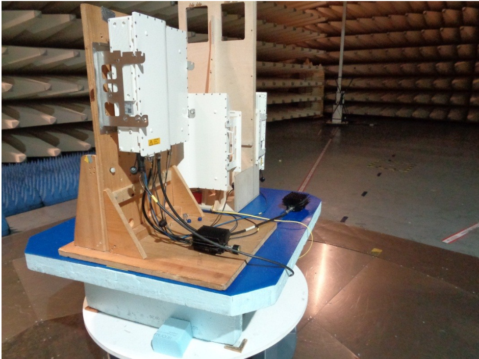
picture 8.3: Test setup
