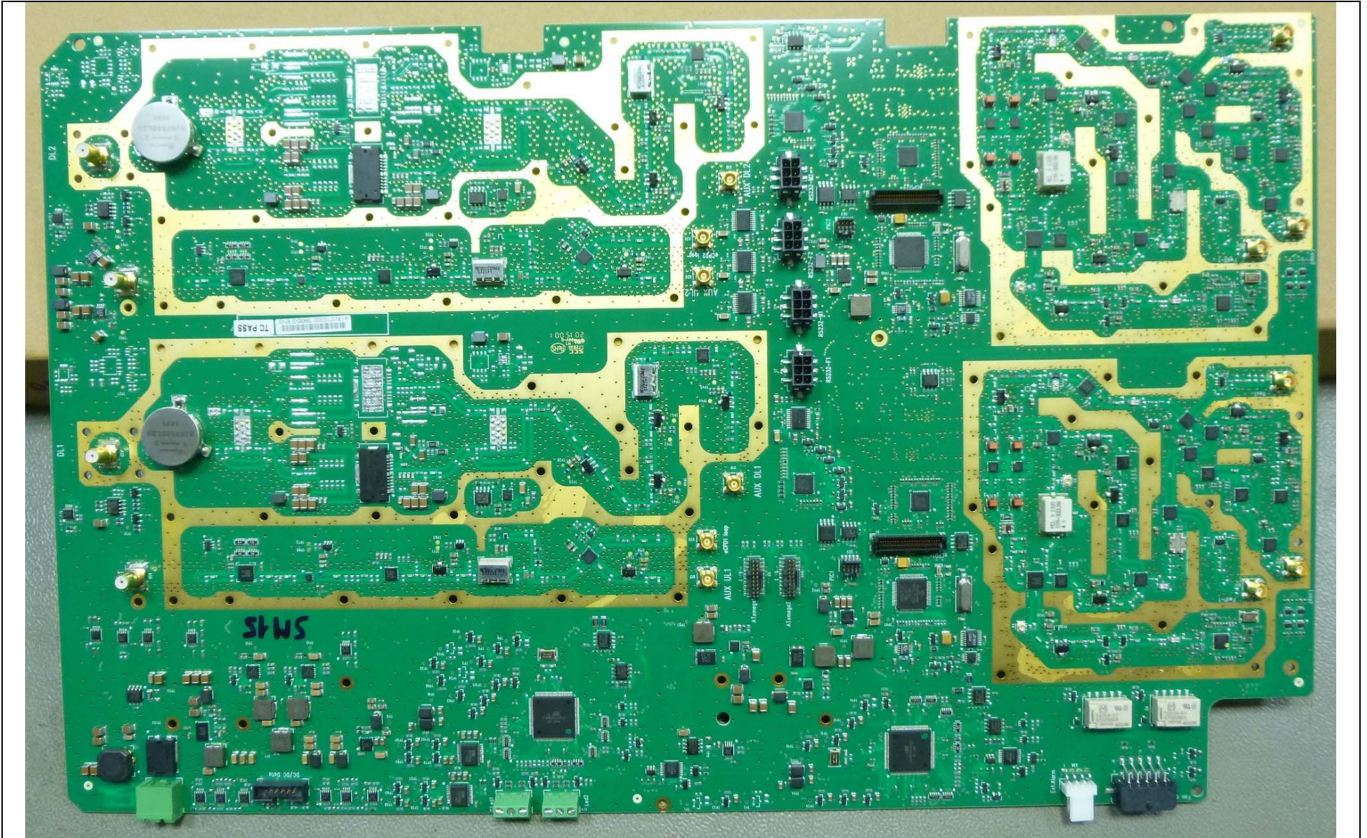
PCB Pop board P3945 ION-U EU L 23/23 (Top) 7699395-00
