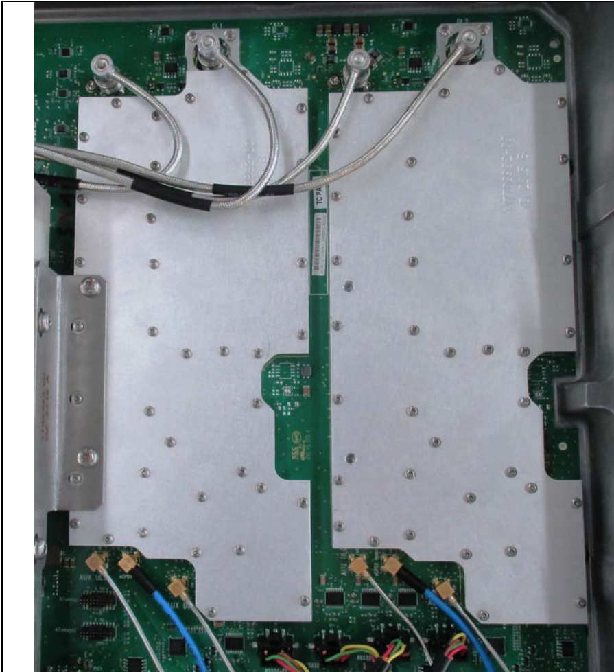
Amplification area
