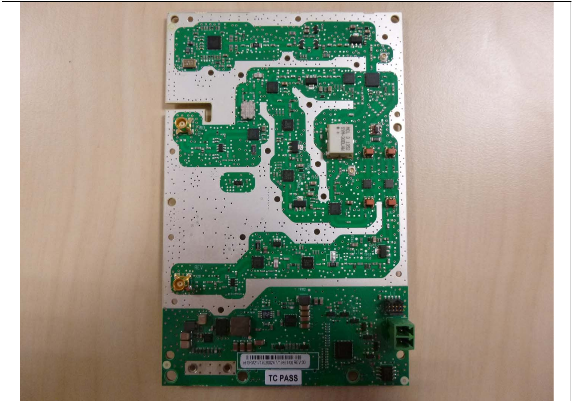
PCB Pop board 4097 eCPD ION-U LP (Top) 7719851-00
