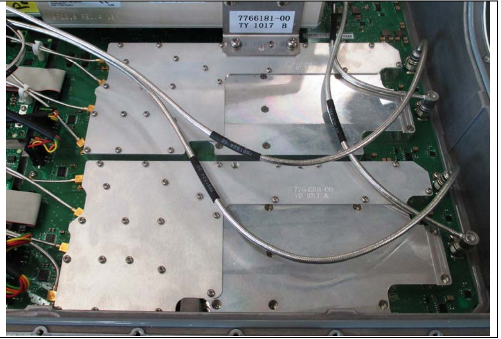
Amplification area
