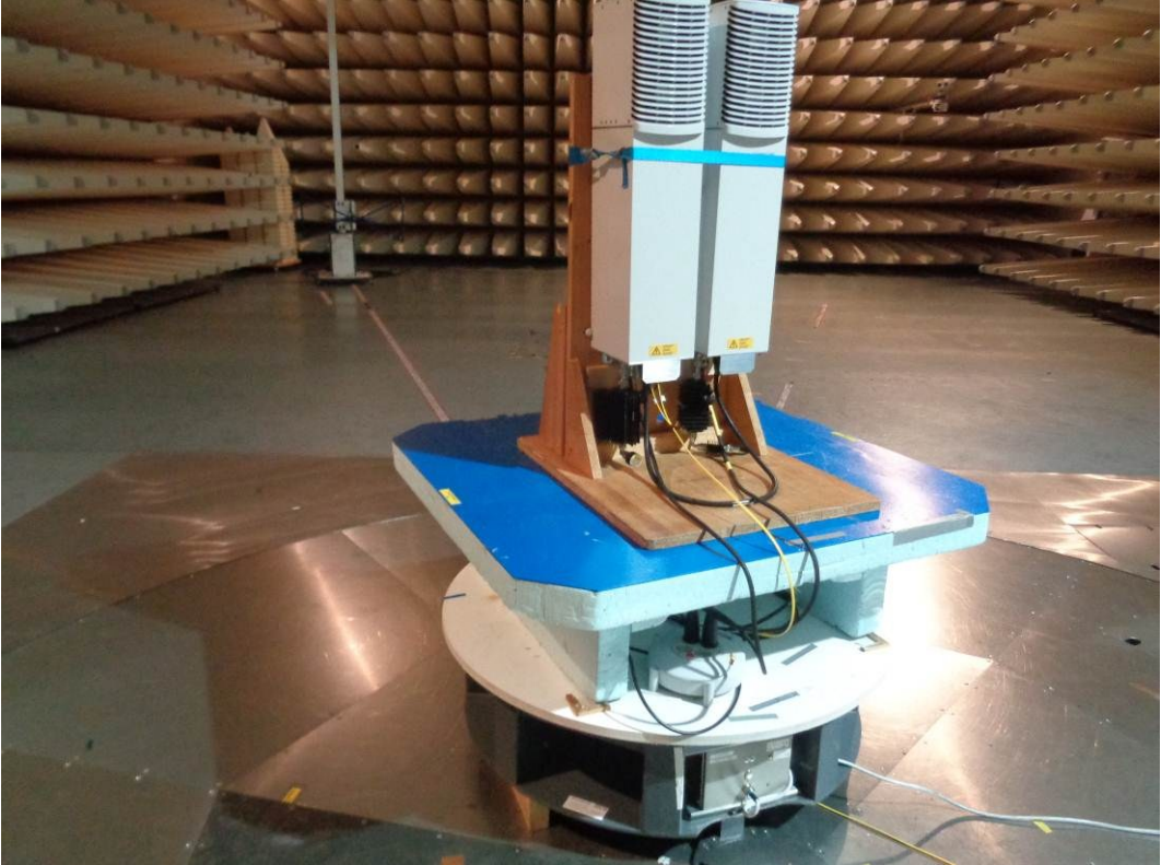
picture 8.3: Test setup: Field Strength Emission 30 MHz - 1 GHz @10m in the SAC
