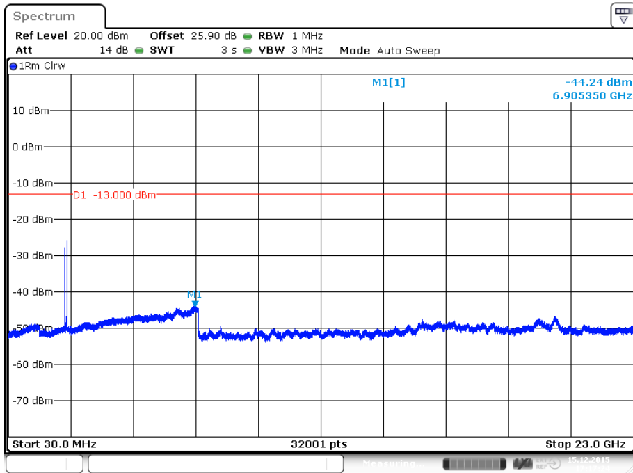
plot 7.3.1.1-#1 Spurious Emissions at Antenna Terminals: §27.53, §2.1051; Test results; Downlink; CDMA > 1MHz to band edge; carrier (2145MHz) notched
