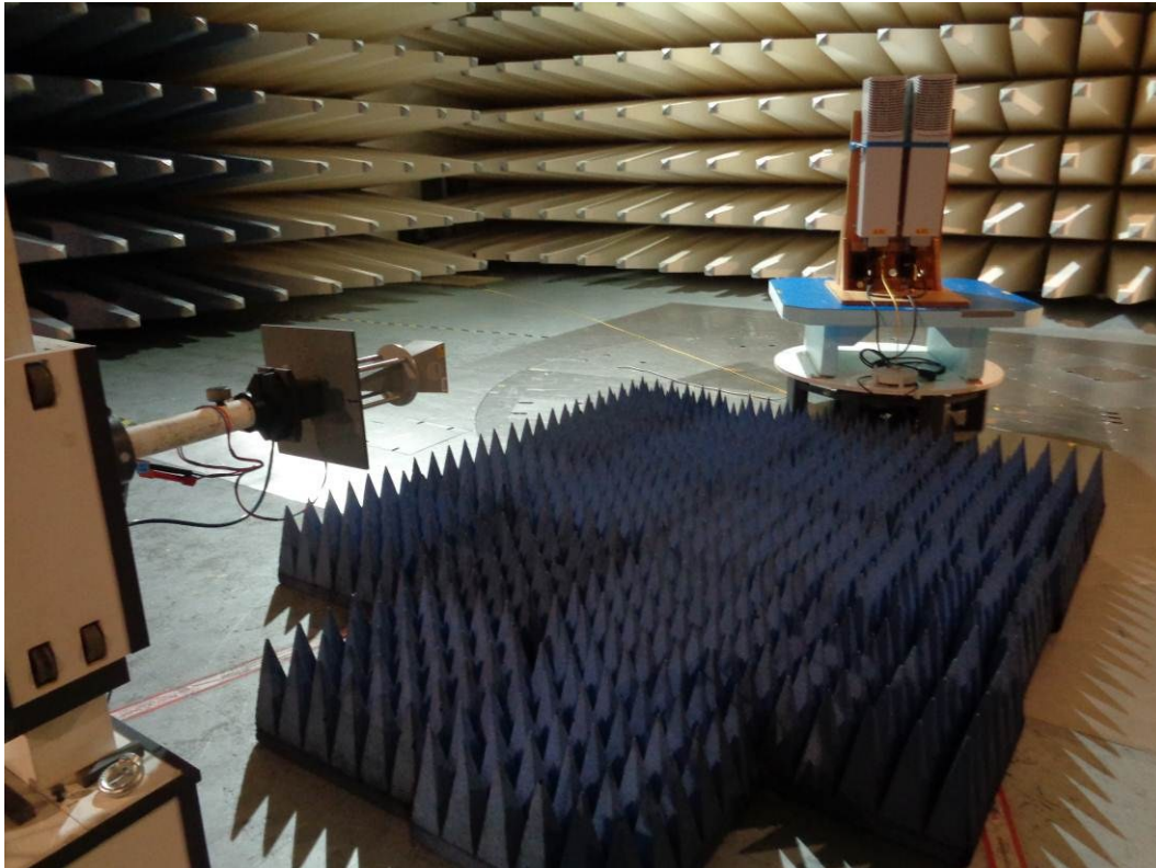
picture 8.5: Test setup: Field Strength Emission 18-26 GHz @3m in the SAC
