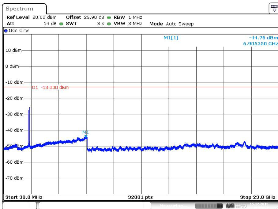
plot 7.3.1.3-#1 Spurious Emissions at Antenna Terminals: §27.53, §2.1051; Test results; Downlink; LTE > 1MHz to band edge; carrier (2145MHz) notched
