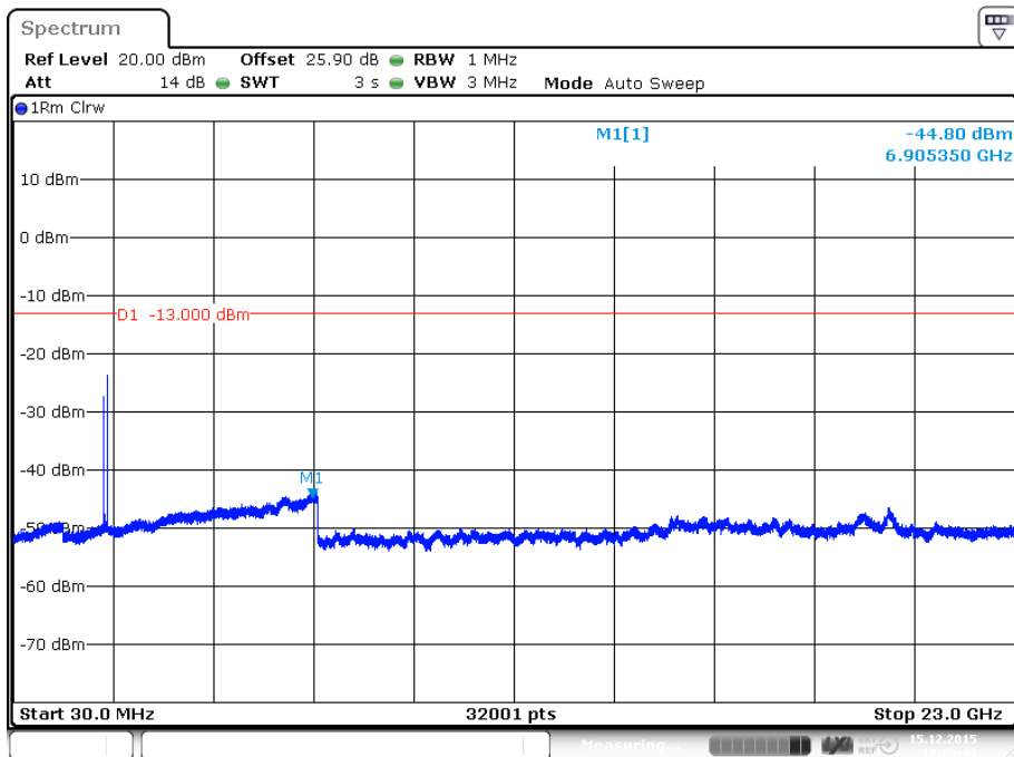
plot 7.3.1.2-#1 Spurious Emissions at Antenna Terminals: §27.53, §2.1051; Test results; Downlink; W-CDMA > 1MHz to band edge; carrier (2145MHz) notched
