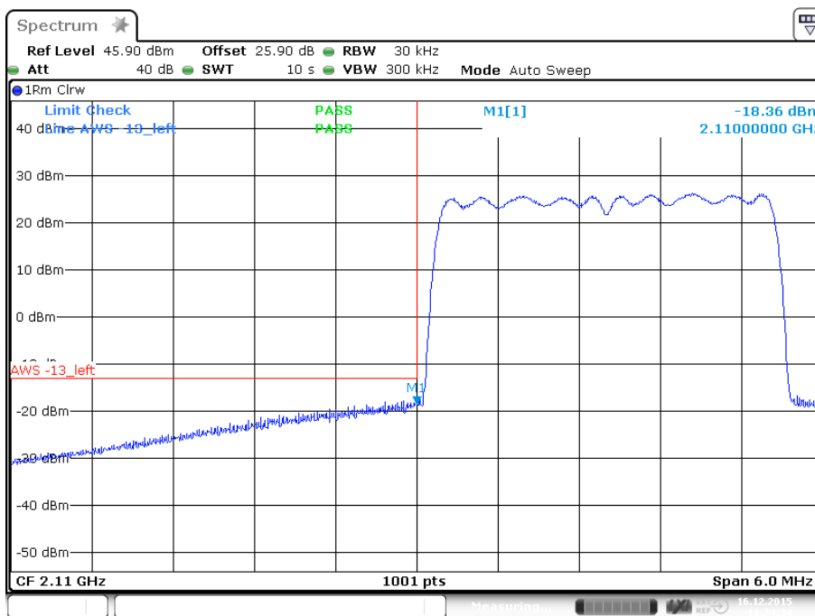
plot 8.3.1.1-#1 Intermodulation: §27.53, §2.1051; Test results; Downlink; CDMA < 1MHz to band edge Lower Band Edge
