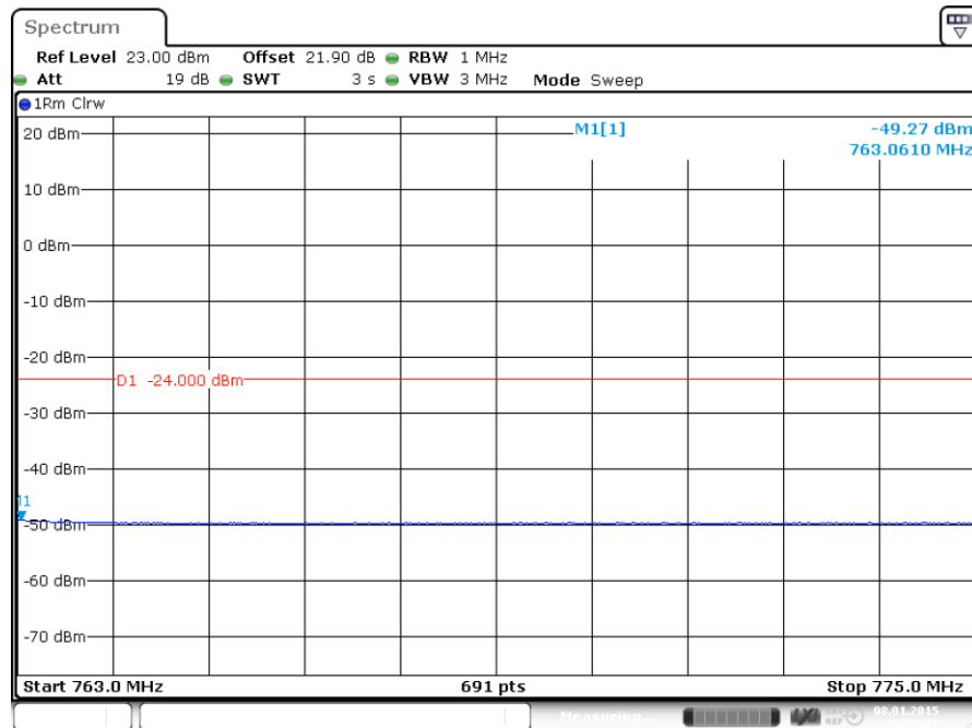
plot 7.3.1.1-#2 Spurious Emissions at Antenna Terminals: §27.53, §2.1051; Test results; Downlink; LTE 728 – 746MHz; 763 MHz – 775 MHz
