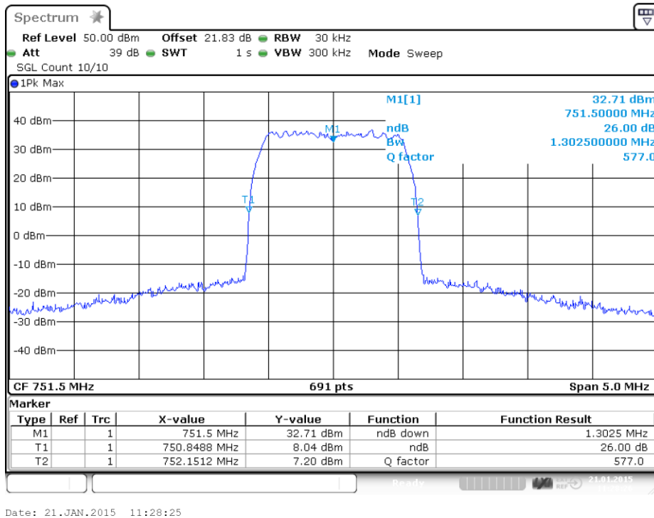
plot 6.3.2.2-#1 Occupied Bandwidth: §2.1049; Test results; 26dB Bandwidth; LTE 746 – 757MHz Output
