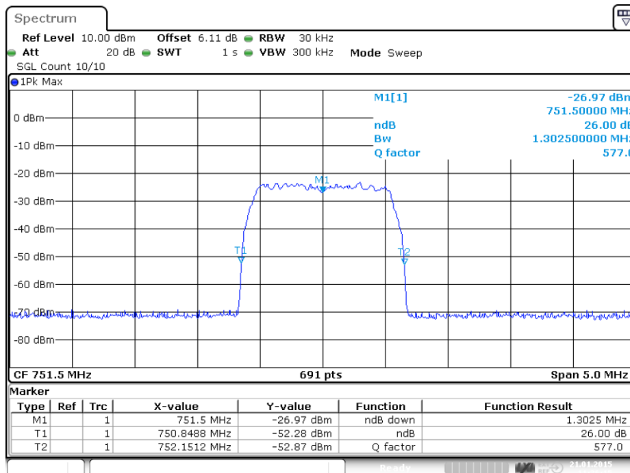
plot 6.3.2.2-#2 Occupied Bandwidth: §2.1049; Test results; 26dB Bandwidth; LTE 746 – 757MHz Input
