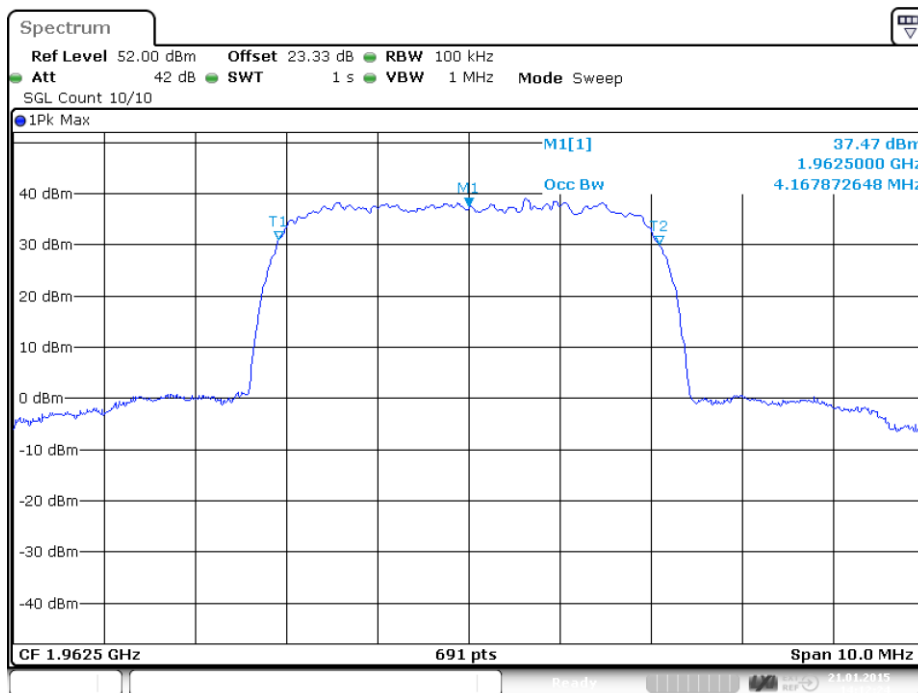
plot 6.2.1.4-#1 Occupied Bandwidth: §2.1049;; Test method; Downlink; WCDMA Output
