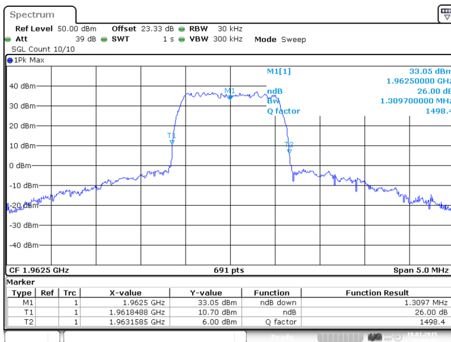
plot 6.2.2.5-#1 Occupied Bandwidth: §2.1049;; Test method; 26dB Bandwidth; LTE Output
