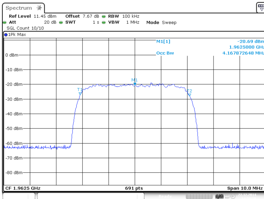
plot 6.2.1.4-#2 Occupied Bandwidth: §2.1049;; Test method; Downlink; WCDMA Input
