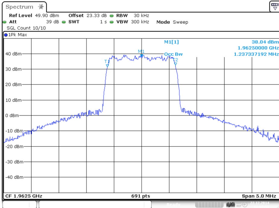
plot 6.2.1.3-#1 Occupied Bandwidth: §2.1049;; Test method; Downlink; CDMA Output
