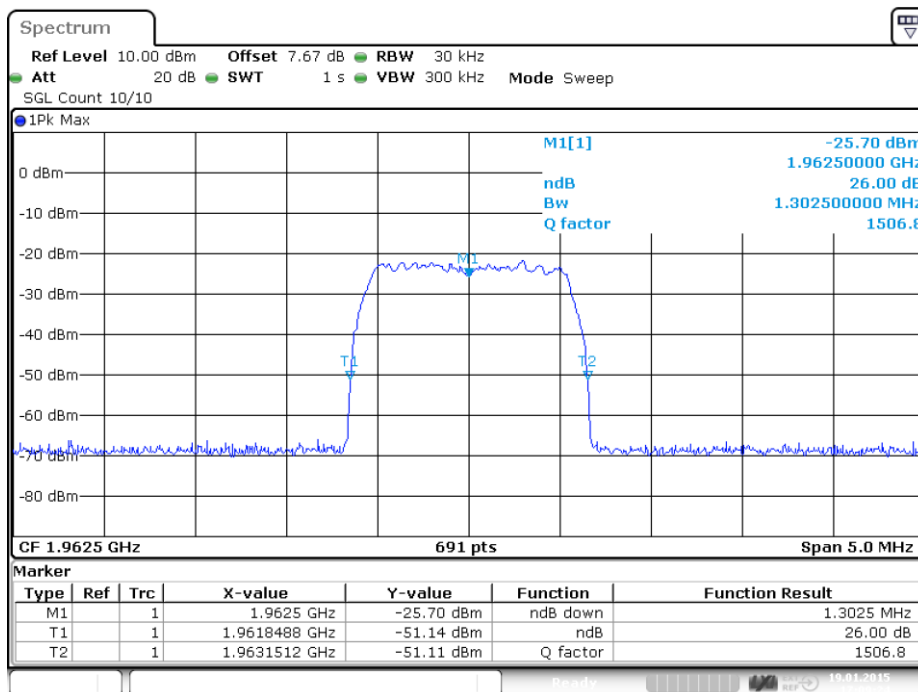
plot 6.2.2.5-#2 Occupied Bandwidth: §2.1049;; Test method; 26dB Bandwidth; LTE Input
