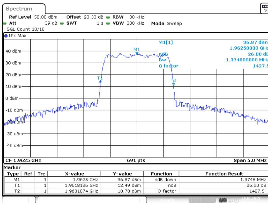
plot 6.2.2.3-#1 Occupied Bandwidth: $2.1049;; Test method; 26dB Bandwidth; CDMA Output
