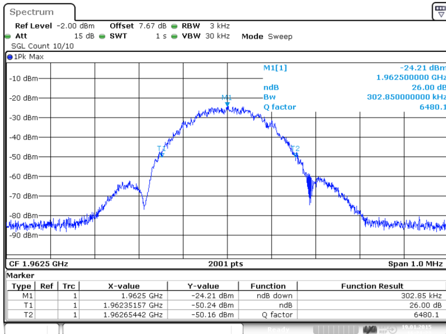
plot 6.2.2.2-#1 Occupied Bandwidth: §2.1049;; Test method; 26dB Bandwidth; EDGE Output
