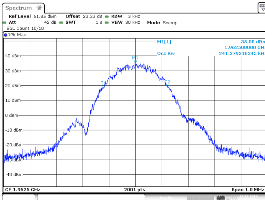
plot 6.2.1.2-#1 Occupied Bandwidth: $2.1049;; Test method; Downlink; EDGE Output
