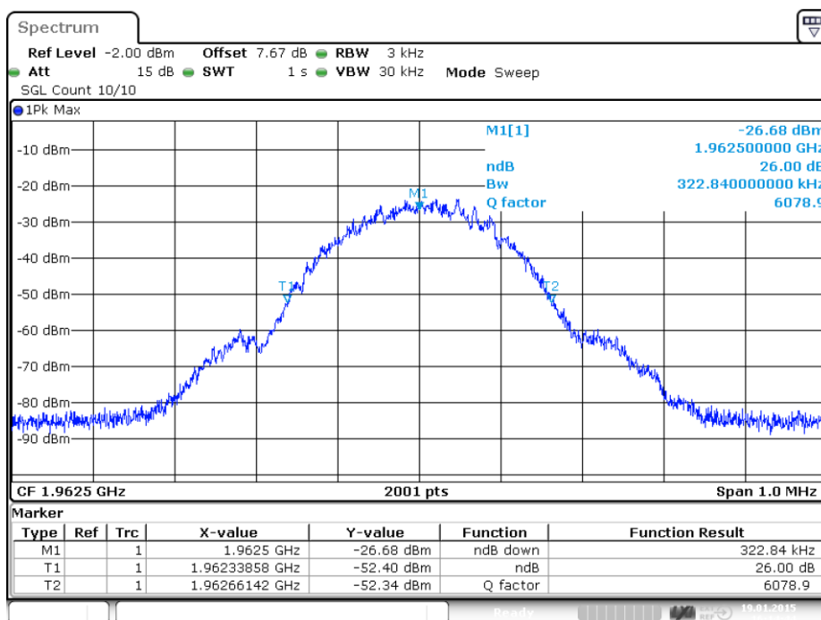
plot 6.2.2.1-#1 Occupied Bandwidth: §2.1049;; Test method; 26dB Bandwidth; GSM Output
