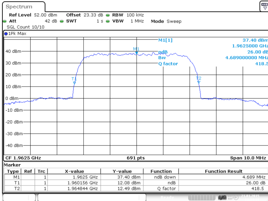
plot 6.2.2.4-#1 Occupied Bandwidth: §2.1049;; Test method; 26dB Bandwidth; WCDMA Output
