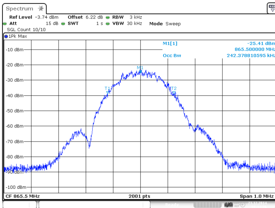
plot 6.3.1.2-#2 Occupied Bandwidth: §90.210, §2.1049; Test results; Downlink; EDGE Input
