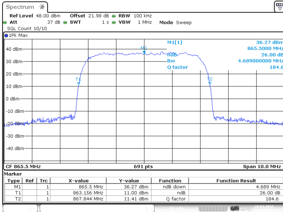
plot 6.3.2.4-#1 Occupied Bandwidth: §90.210, §2.1049; Test results; 26dB BW; WCDMA Output
