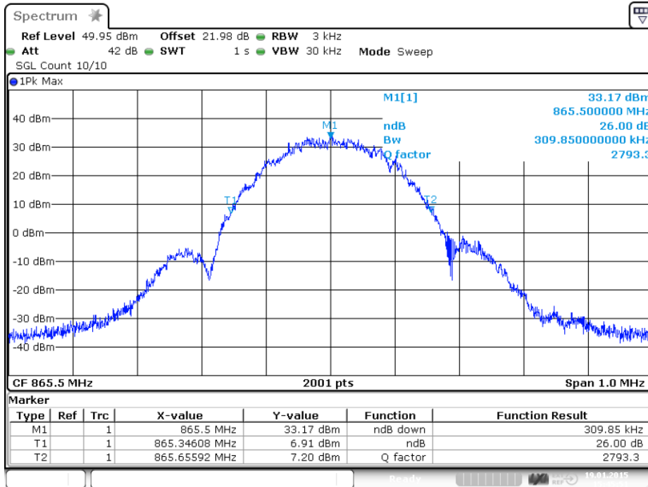
plot 6.3.2.2-#1 Occupied Bandwidth: §90.210, §2.1049; Test results; 26dB BW; EDGE Output
