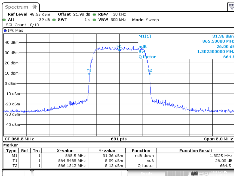
plot 6.3.2.5-#1 Occupied Bandwidth: §90.210, §2.1049; Test results; 26dB BW; LTE Output
