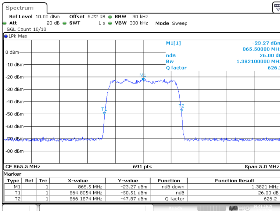
plot 6.3.2.3-#2 Occupied Bandwidth: $90.210, $2.1049; Test results; 26dB BW; CDMA Input
