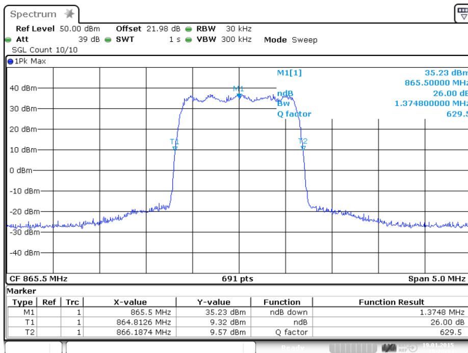
plot 6.3.2.3-#1 Occupied Bandwidth: $90.210, $2.1049; Test results; 26dB BW; CDMA Output
