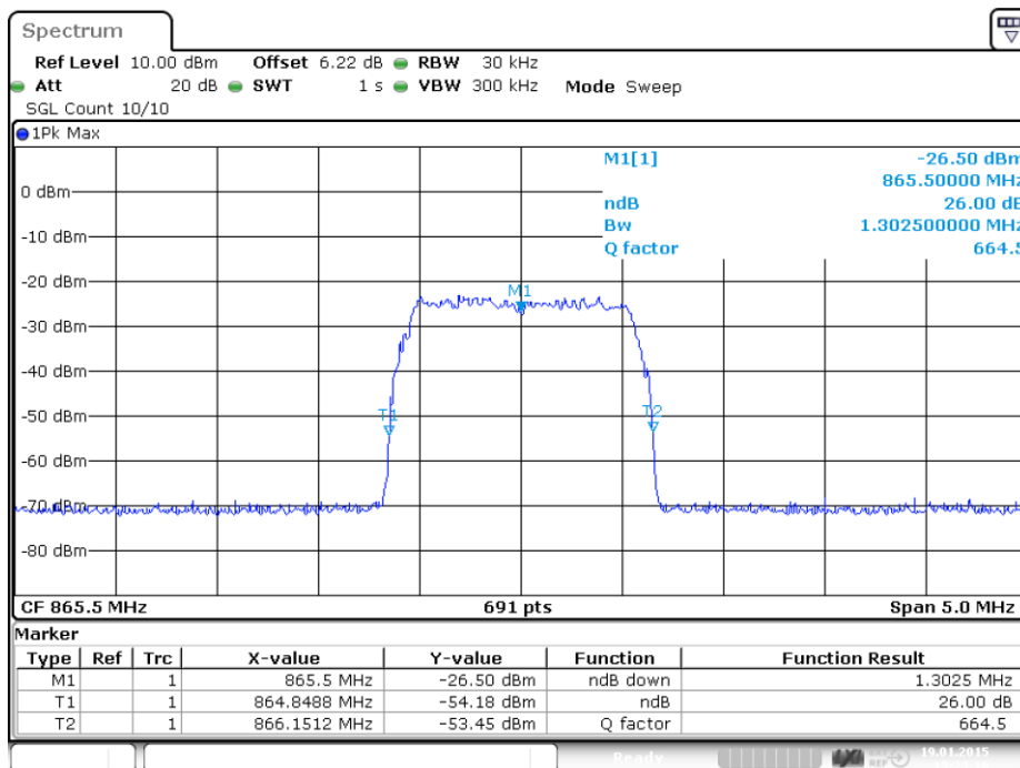
plot 6.3.2.5-#2 Occupied Bandwidth: §90.210, §2.1049; Test results; 26dB BW; LTE Input
