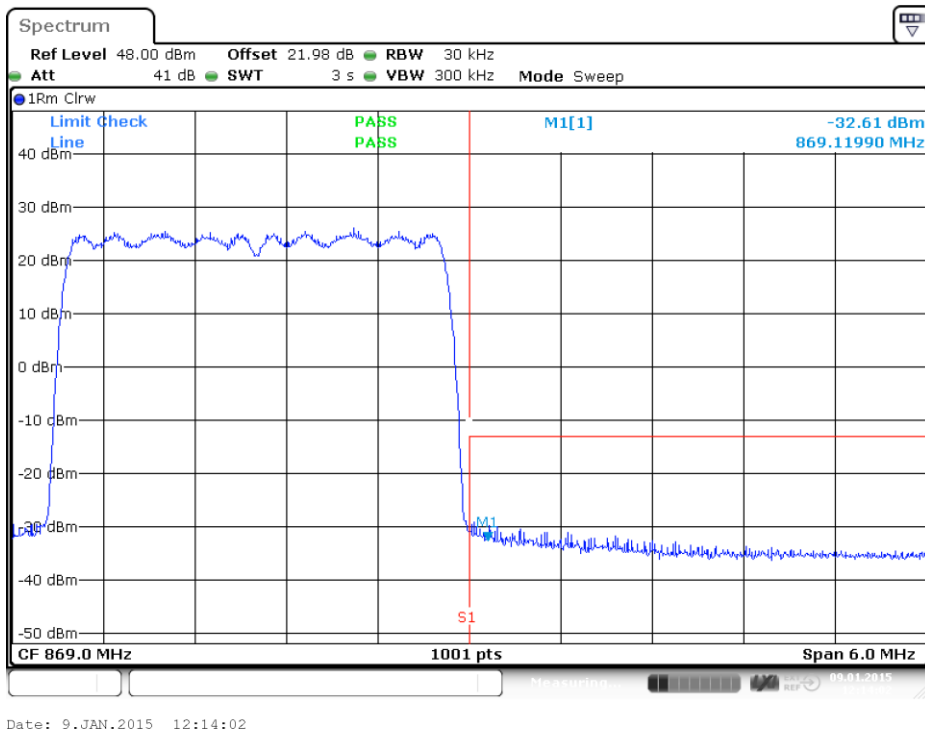
plot 8.3.1.3-#2 Intermodulation: §90.219, §2.1051; Test results; Downlink; CDMA Upper Band Edge
