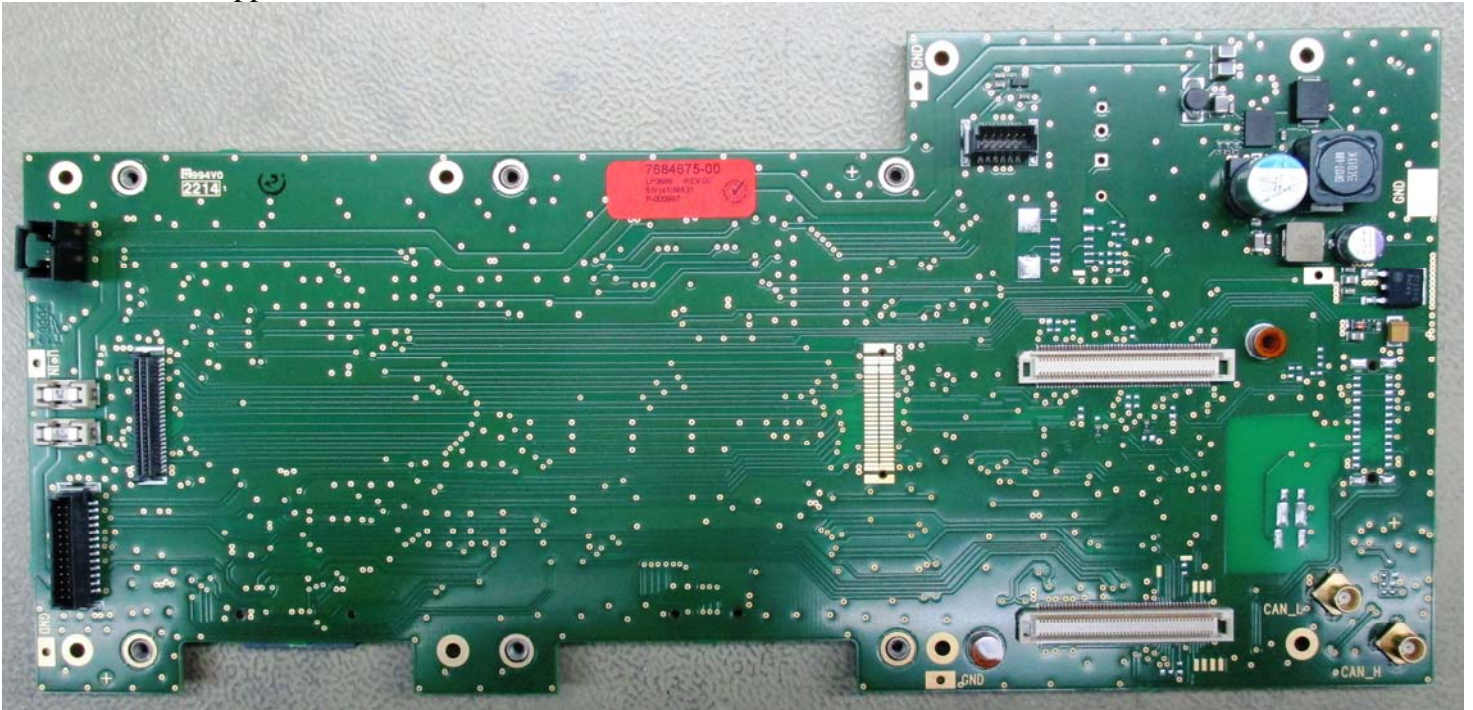
PCB P3686 EU Application board M2 Cab 7684675-00
