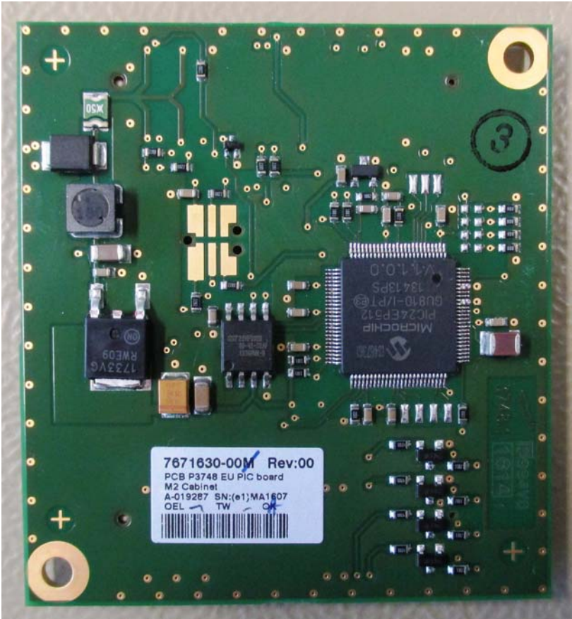
PCB P3748 EU PIC board M2 Cabinet 7671630-00
