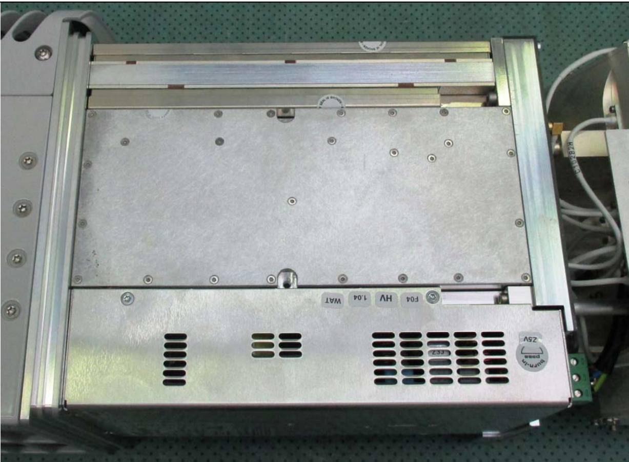
eCPD+ & Controller
