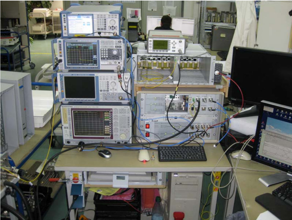
Figure 2. Measurement Equipment
