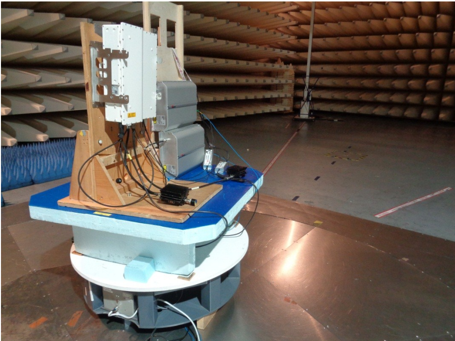
picture 8.4: Test setup: Field Strength Emission
