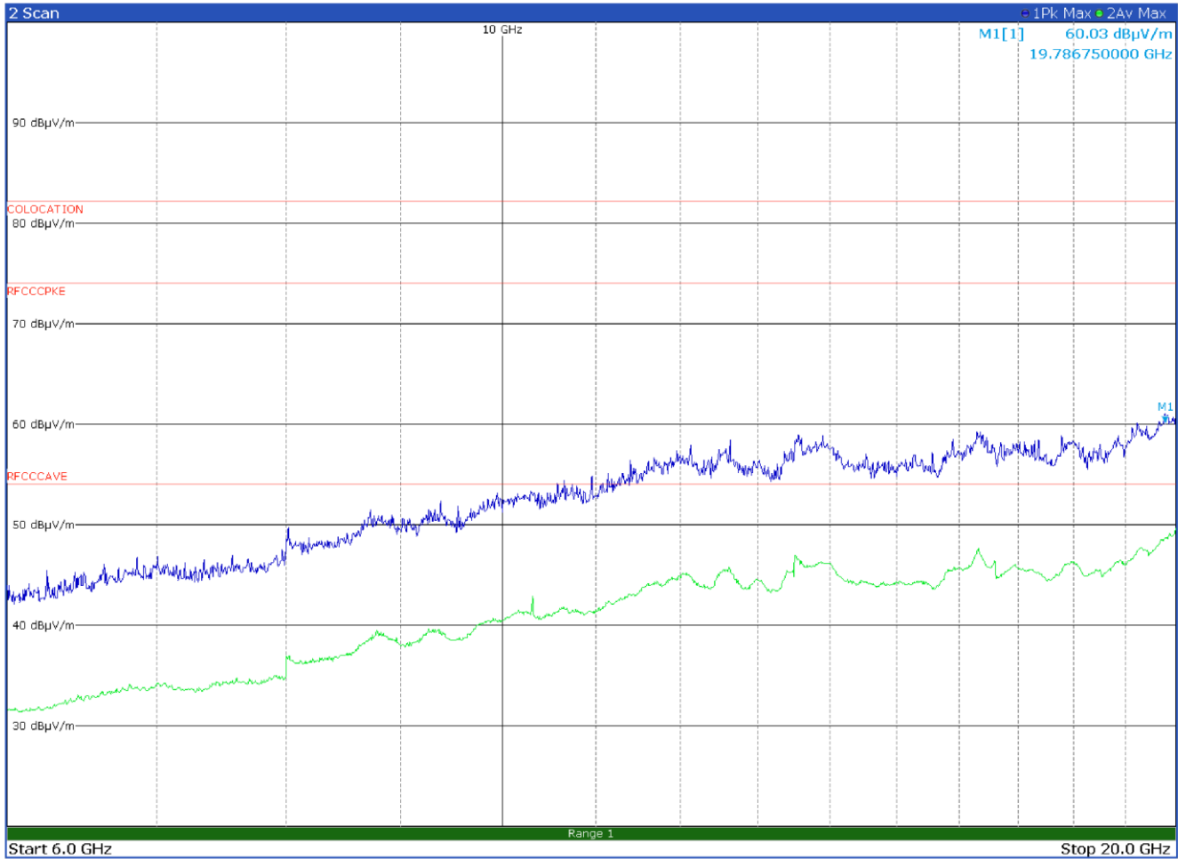
Radiated emission in the frequency range 6 to 20 GHz with antenna in vertical polarization (85-B5 band) No intermodulation products found
