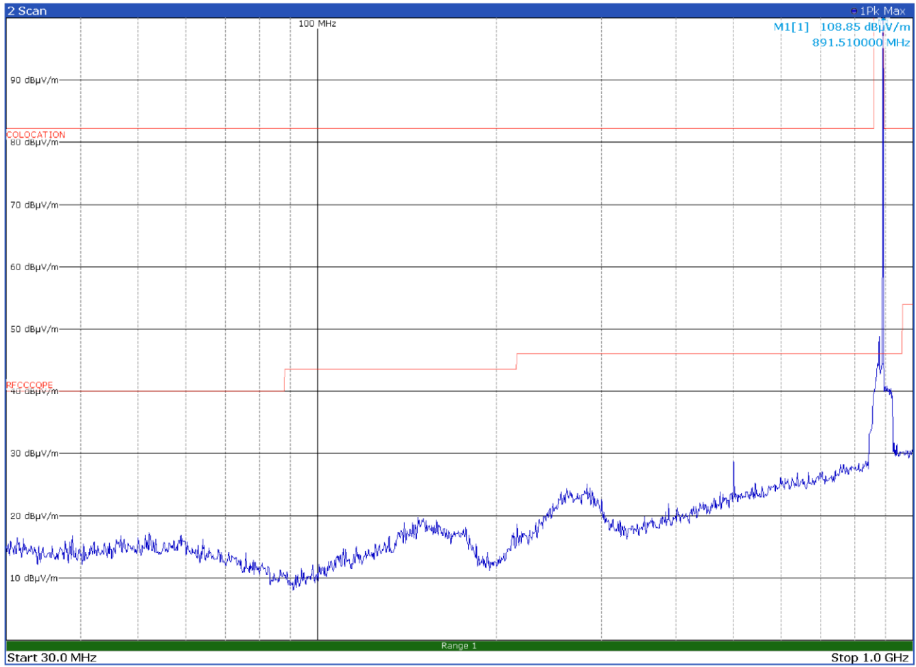
Radiated emission in the frequency range 30 to 1000 MHz with antenna in horizontal polarization (85-B5 band) Limits exceeded by the carriers. No intermodulation products found
