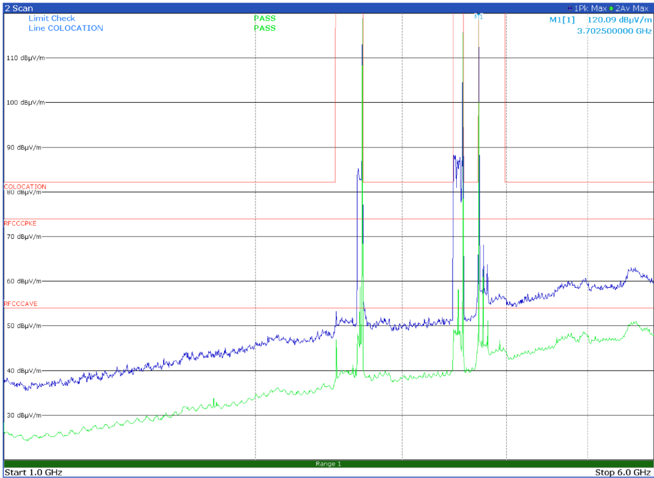
Radiated emission in the frequency range 1 to 6 GHz with antenna in horizontal polarization (85-B5 band) Limits exceeded by the carriers. No intermodulation products found
