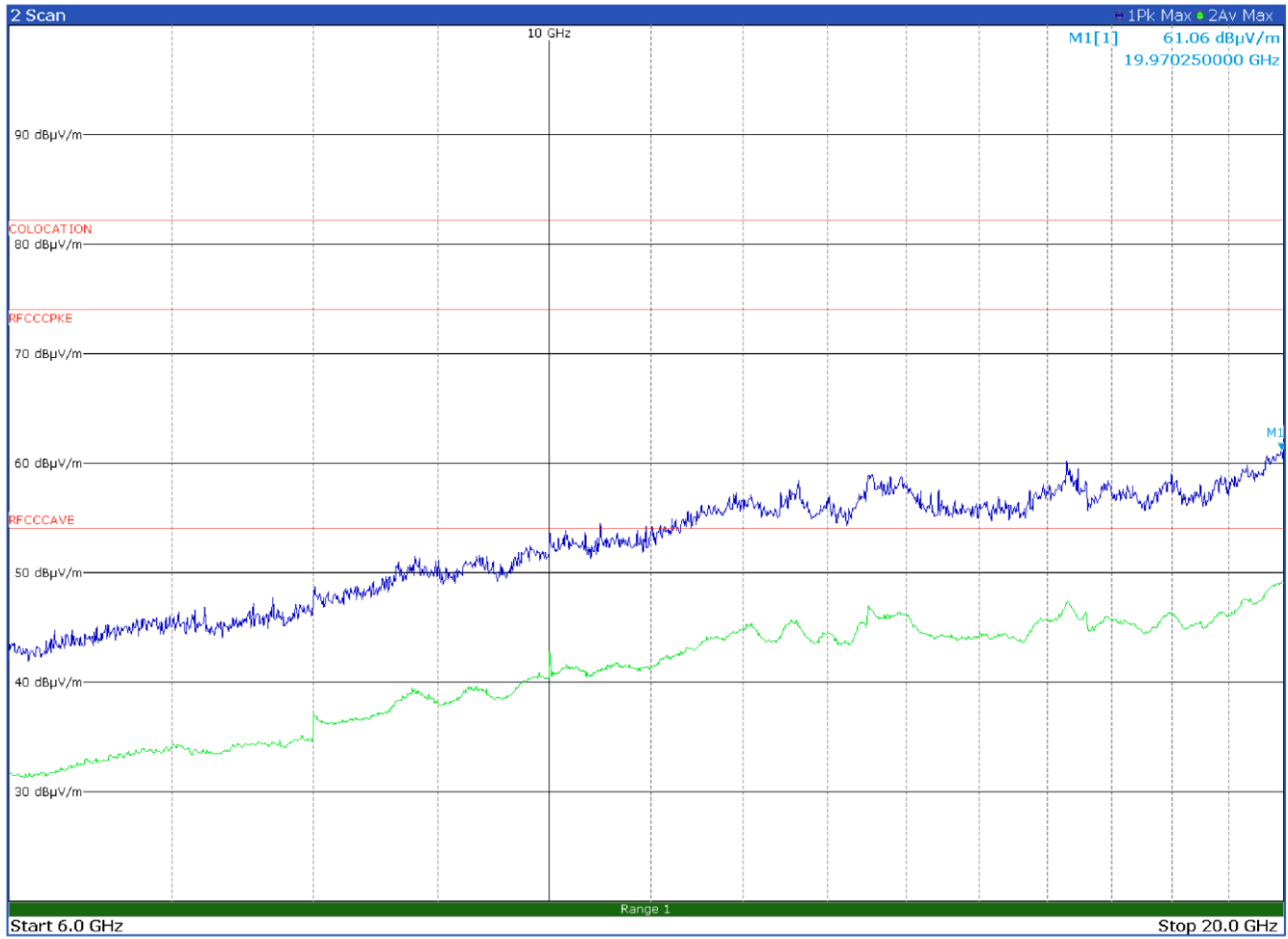
Radiated emission in the frequency range 6 to 20 GHz with antenna in horizontal polarization (80-B27 band) No intermodulation products found
