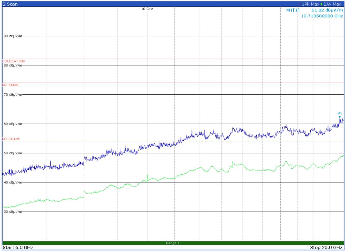
Radiated emission in the frequency range 6 to 20 GHz with antenna in horizontal polarization (85-B5 band) No intermodulation products found
