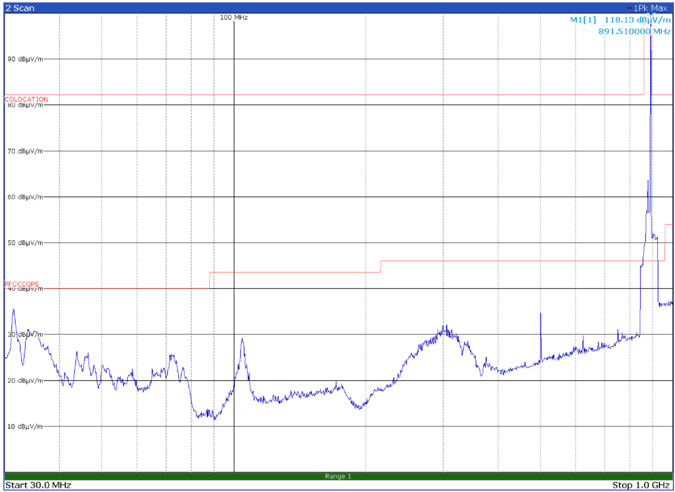
Radiated emission in the frequency range 30 to 1000 MHz with antenna in vertical polarization (85-B5 band) Limits exceeded by the carriers. No intermodulation products found
