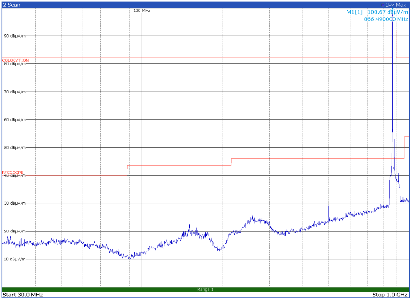
Radiated emission in the frequency range 30 to 1000 MHz with antenna in horizontal polarization (80-B27 band) Limits exceeded by the carriers. No intermodulation products found
