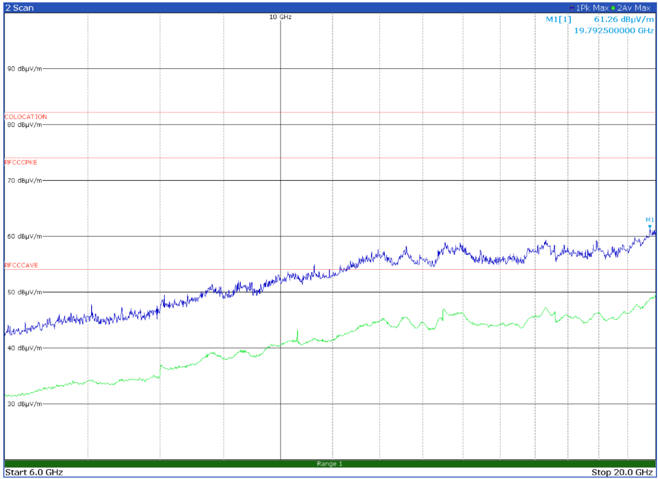
Radiated emission in the frequency range 6 to 20 GHz with antenna in vertical polarization (80-B27 band) No intermodulation products found
