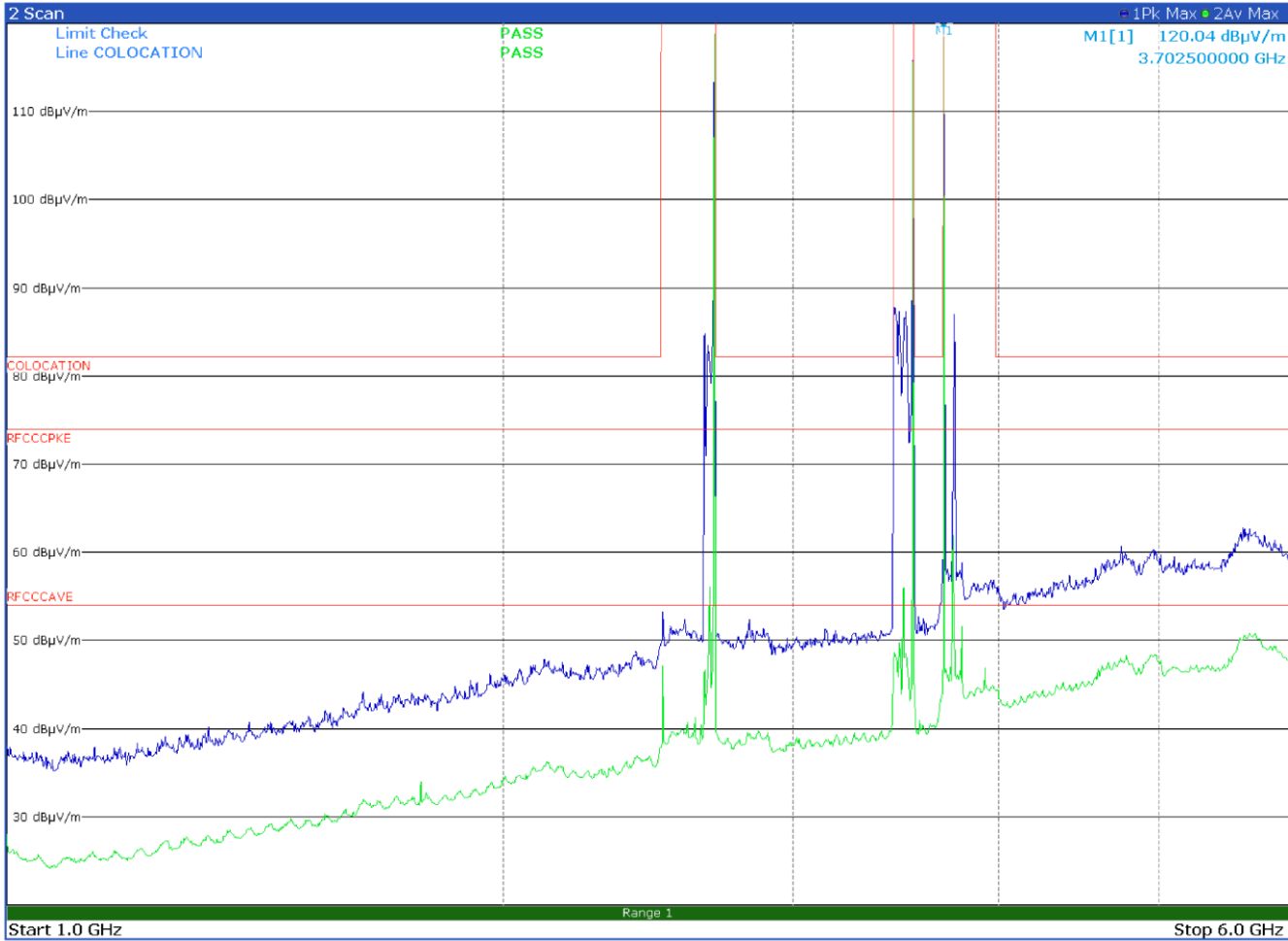
Radiated emission in the frequency range 1 to 6 GHz with antenna in horizontal polarization (80-B27 band) Limits exceeded by the carriers. No intermodulation products found
