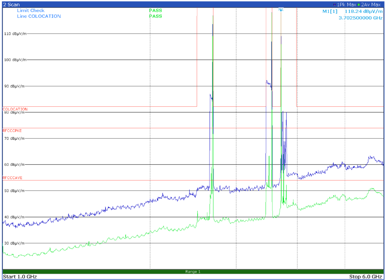
Radiated emission in the frequency range 1 to 6 GHz with antenna in vertical polarization (85-B5 band) Limits exceeded by the carriers. No intermodulation products found
