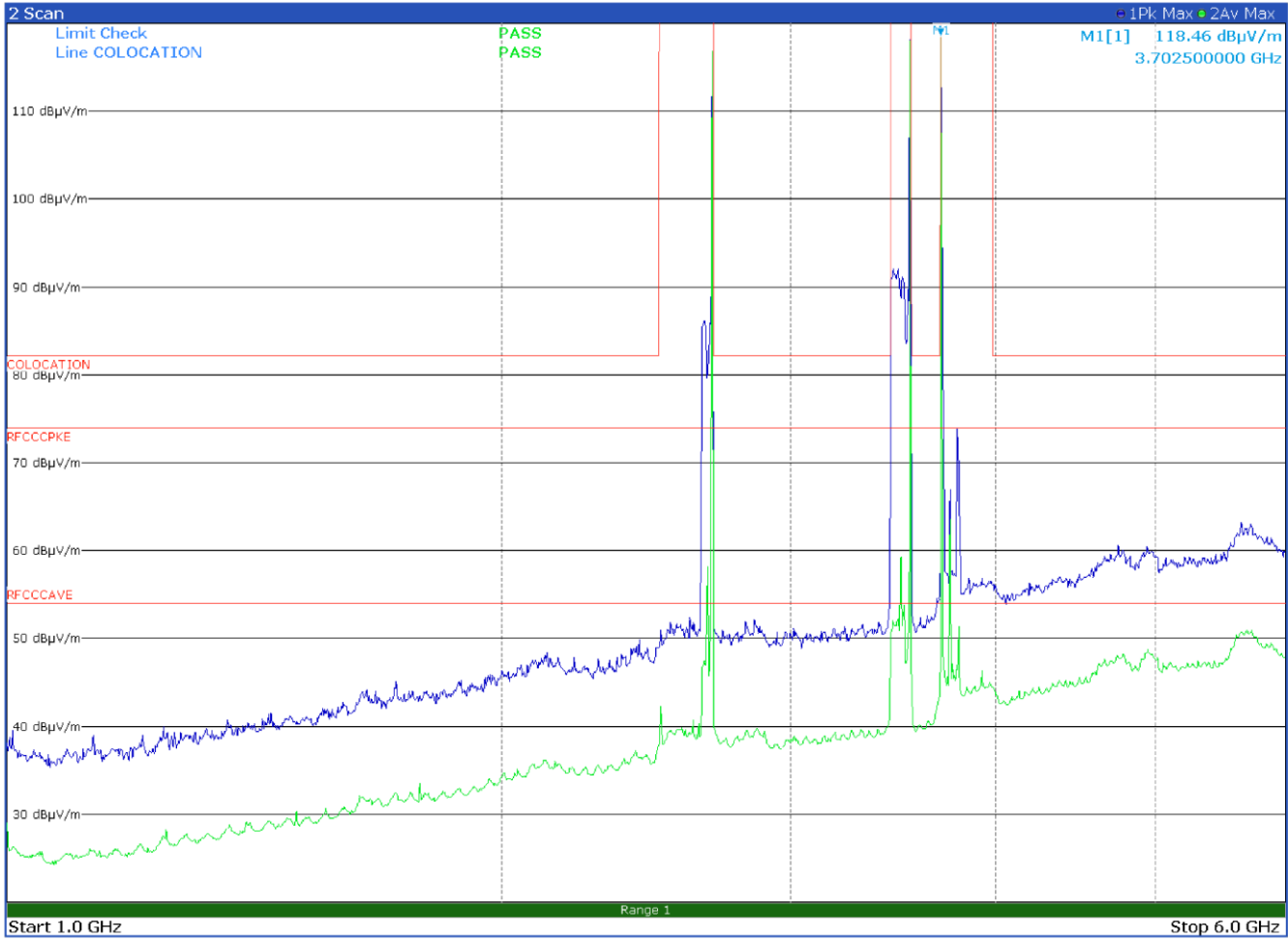
Radiated emission in the frequency range 1 to 6 GHz with antenna in vertical polarization (80-B27 band) Limits exceeded by the carriers. No intermodulation products found
