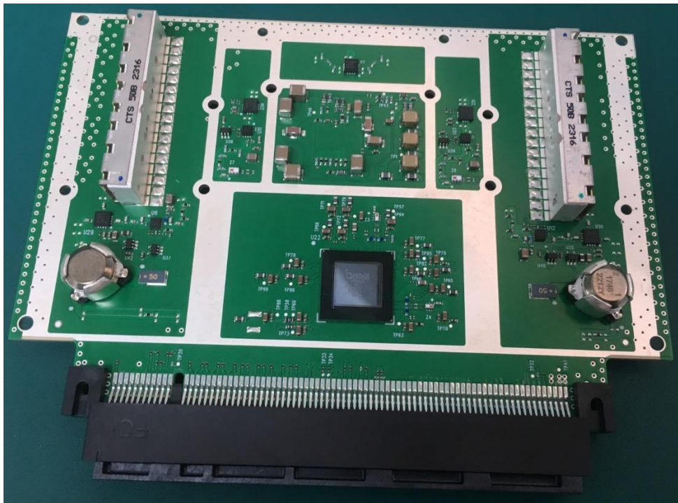
RM 34T – 785726-00 - BOTTOM View
