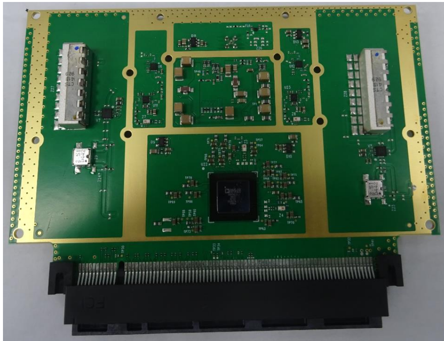
RM 25T – 7843230-03 - BOTTOM View
