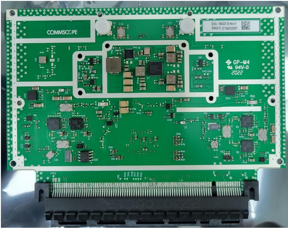
RM 37T – 785527-xx - TOP View
