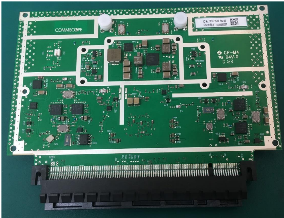
RM 34T – 785726-00 – TOP View
