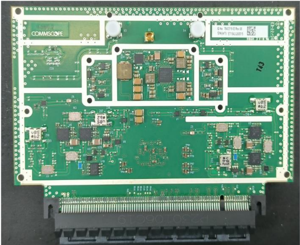
RM 80-85 – 7843219-03 - TOP View
