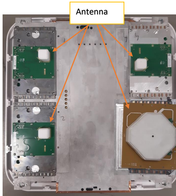
UAP 2 without upper cover
