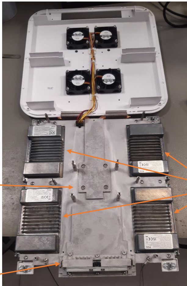
UAP 2 without upper cover and ventilation cover
