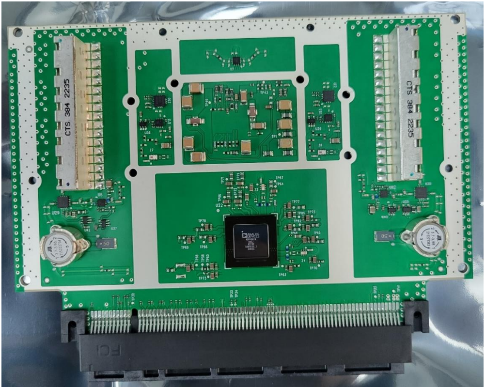
RM 37T – 785527-xx – BOTTOM View
