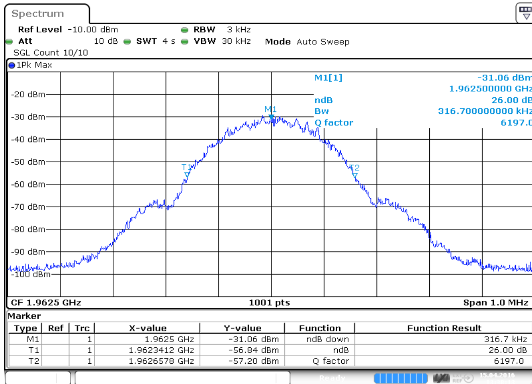
plot 6.3.2.1-#1 Occupied Bandwidth: $2.1049;; Test results; 26dB Bandwidth; GSM Output
