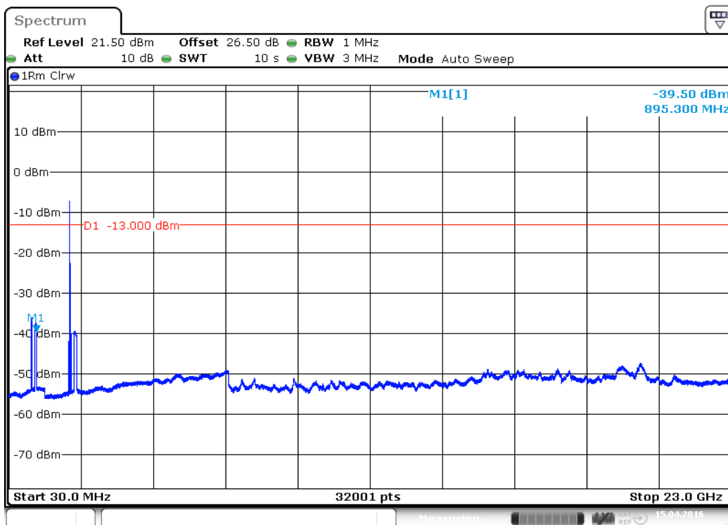
plot 7.3.1.3-#1 Spurious Emissions at Antenna Terminals: §24.238, §2.1051; Test results; Downlink; CDMA; carrier (1962,5MHz) notched
