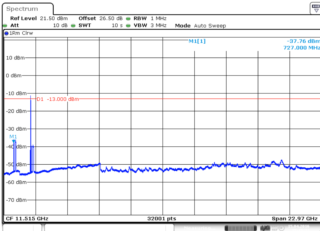
plot 7.3.1.4-#1 Spurious Emissions at Antenna Terminals: §24.238, §2.1051; Test results; Downlink; WCDMA; carrier (1962,5MHz) notched
