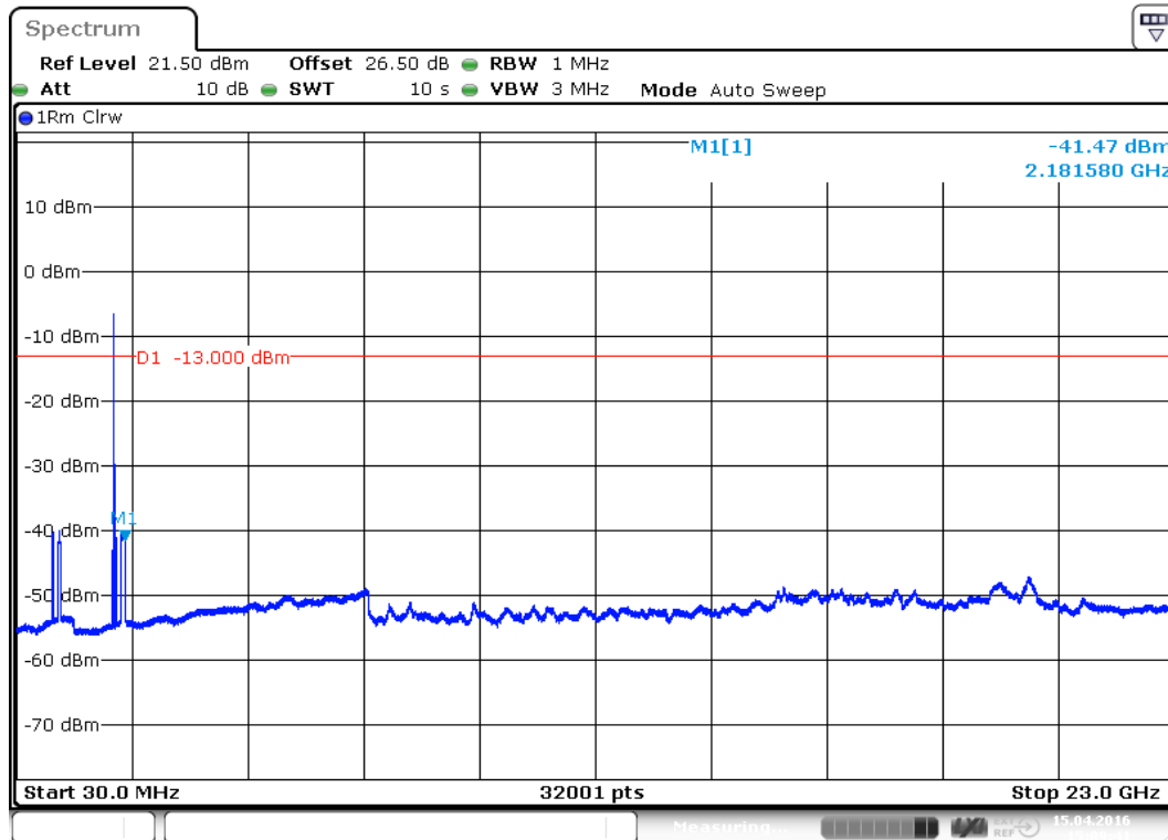
plot 7.3.1.1-#1 Spurious Emissions at Antenna Terminals: §24.238, §2.1051; Test results; Downlink; GSM; carrier (1962,5MHz) notched
