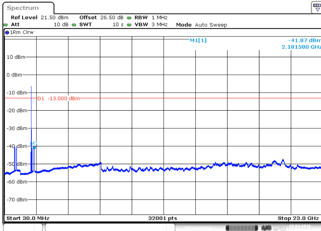
plot 7.3.1.2-#1 Spurious Emissions at Antenna Terminals: §24.238, §2.1051; Test results; Downlink; EDGE; carrier (1962,5MHz) notched
