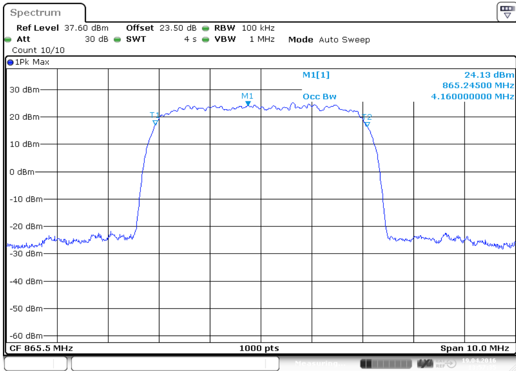
plot 6.3.1.4-#1 Occupied Bandwidth: §90.210, §2.1049; Test results; Downlink; WCDMA Output
