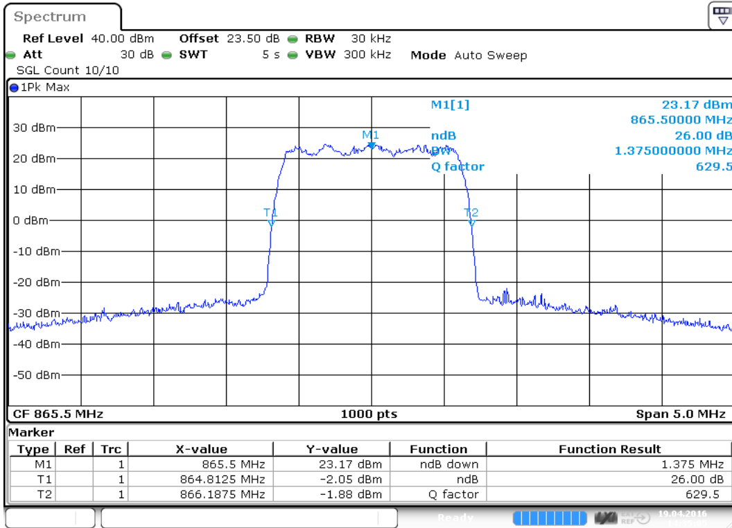
plot 6.3.2.3-#1 Occupied Bandwidth: §90.210, §2.1049; Test results; 26dB Bandwidth; CDMA Output
