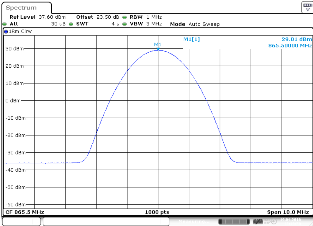
plot 5.3.1.1-#1 RF Power Out: §90.635, §2.1046; Test Results; Downlink; GSM Middle
