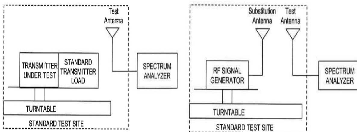
picture 8.3: Substitution method
