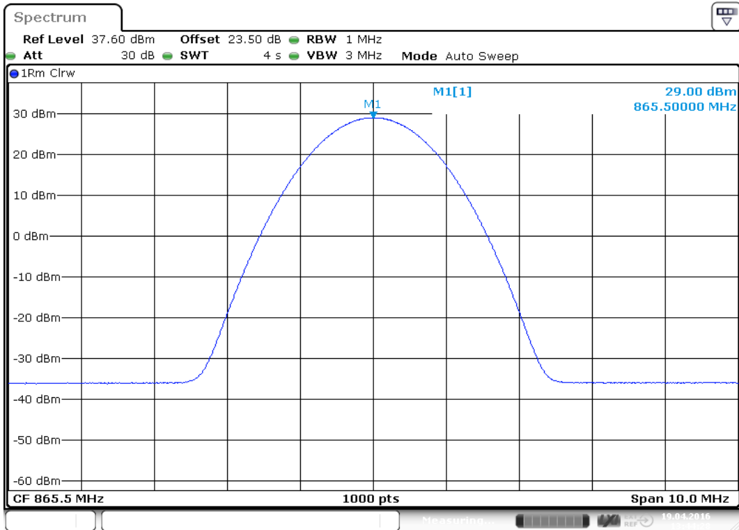
plot 5.3.1.2-#1 RF Power Out: §90.635, §2.1046; Test Results; Downlink; EDGE Middle
