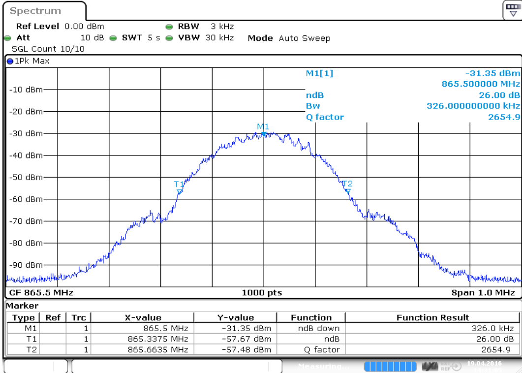
plot 6.3.2.1-#1 Occupied Bandwidth: $90.210, $2.1049; Test results; 26dB Bandwidth; GSM Output
