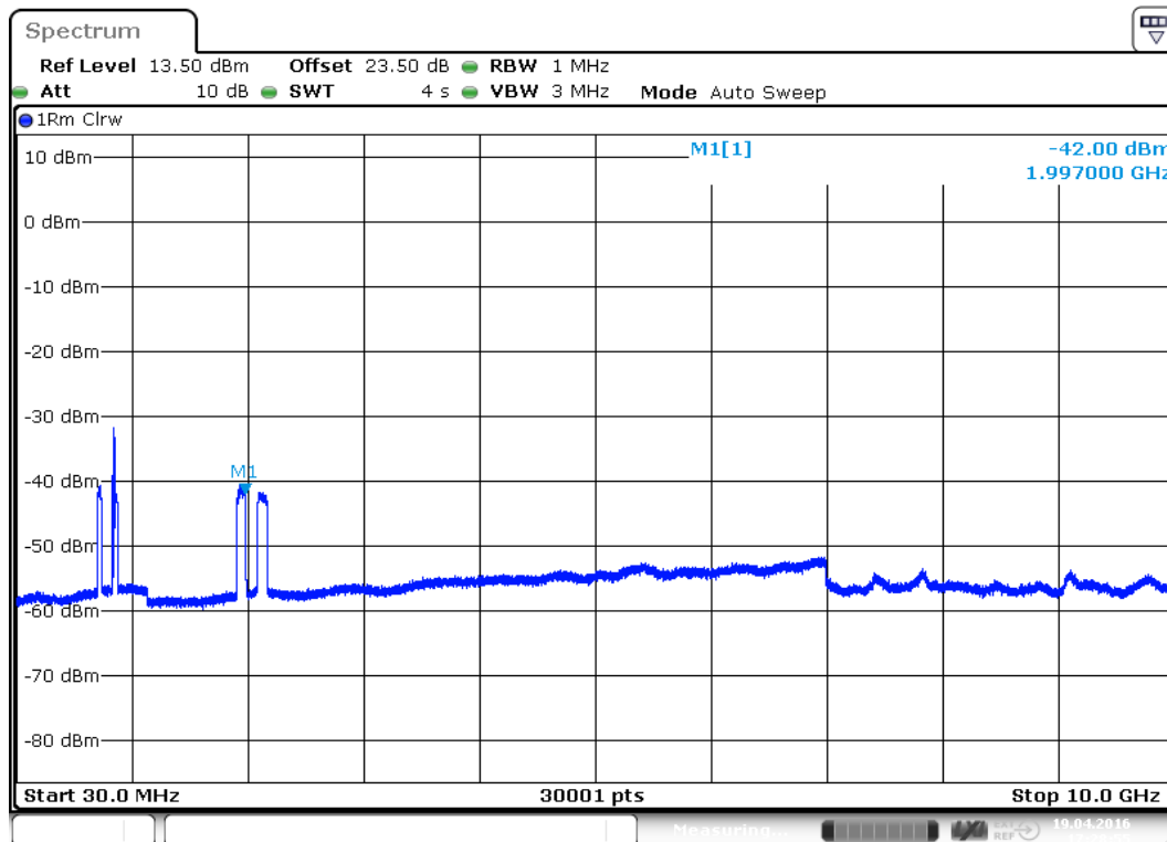
plot 7.3.1.4-#1 Spurious Emissions at Antenna Terminals: §90.210, §2.1051; Test results; Downlink; WCDMA; carrier (865,5MHz) notched
