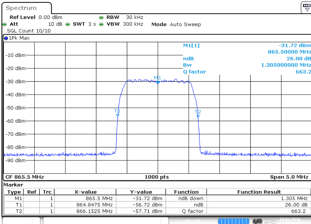
plot 6.3.2.5-#1 Occupied Bandwidth: §90.210, §2.1049; Test results; 26dB Bandwidth; LTE Output
