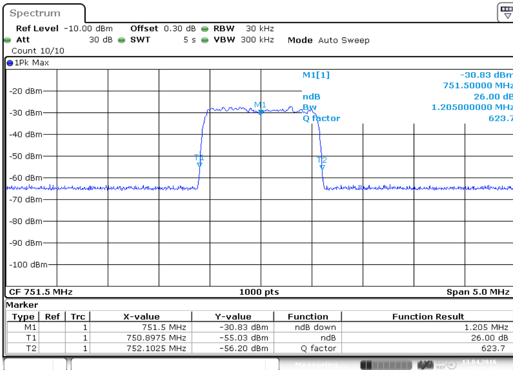
plot 6.3.2.2-#1 Occupied Bandwidth: §2.1049; Test results; 26 dB Bandwidth; LTE 746 – 757MHz Output
