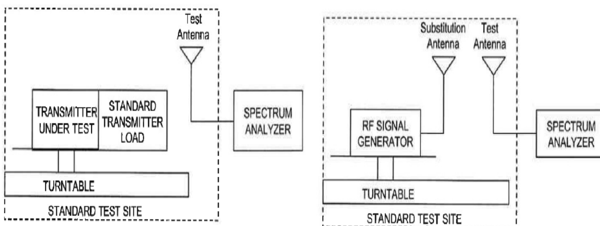
Figure #8.3 Substitution methods TIA/EIA-603-C
