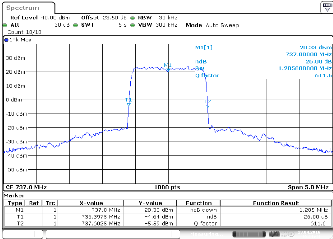
plot 6.3.2.1-#1 Occupied Bandwidth: $2.1049; Test results; 26 dB Bandwidth; LTE 728 – 746 MHz Output
