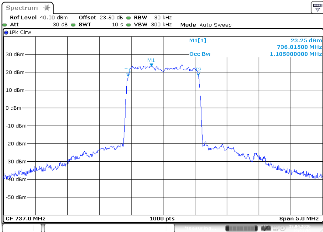
plot 6.3.1.1-#1 Occupied Bandwidth: $2.1049; Test results; Downlink; LTE 728 – 746MHz Output
