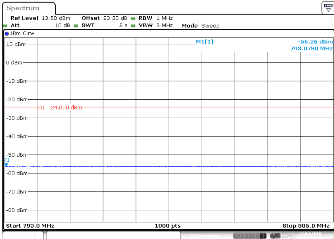
plot 7.3.1.2-#2 Spurious Emissions at Antenna Terminals: §27.53, §2.1051; Test results; Downlink; LTE 746 – 757MHz; 763 MHz – 775 MHz
