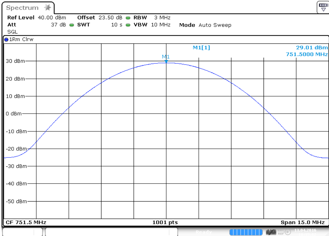
plot 5.3.1.2-#1 RF Power Out: §27.50, §2.1046; Downlink; LTE 746 – 757MHz Middle
