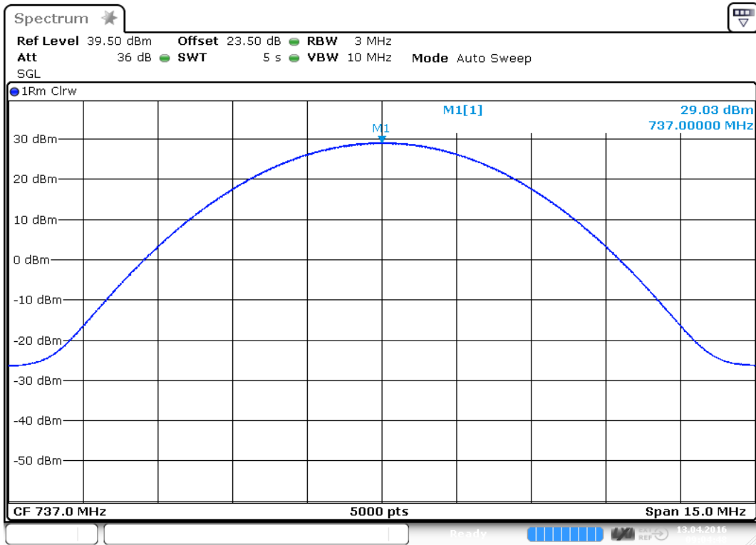
plot 5.3.1.1-#1 RF Power Out: §27.50, §2.1046; Downlink; LTE 728 – 746MHz Middle
