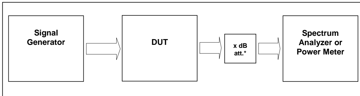
External Attenuator DL x dB = 20 dB figure 4.4-#1 Test setup: Occupied Bandwidth: §2.1049
