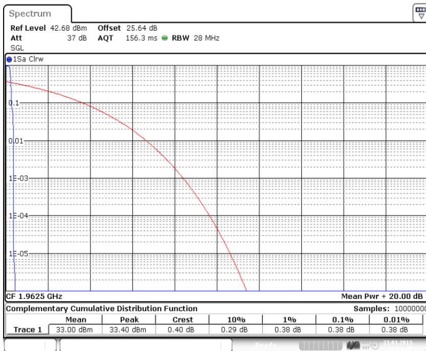
plot 7.3.1.2-#1 Transmitter Output Power: IC RSS-133, RSS-GEN; Test results; Downlink; GSM Middle Peak – to - average
