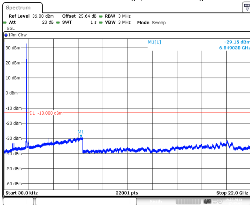
plot 6.3.1.12-#1 Spurious Emissions at Antenna Terminals: §24.238, §2.1051; Test results; Downlink; LTE > 1MHz to band edge; Lower Band Edge
