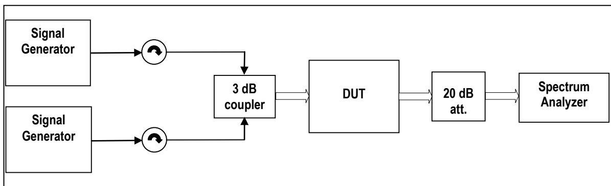
figure 8-#1 Test setup: Transmitter Unwanted Emissions: IC RSS-133
