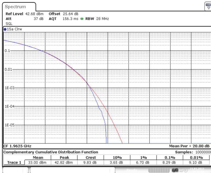
plot 7.3.1.6-#1 Transmitter Output Power: IC RSS-133, RSS-GEN; Test results; Downlink; LTE Middle Peak – to - average
