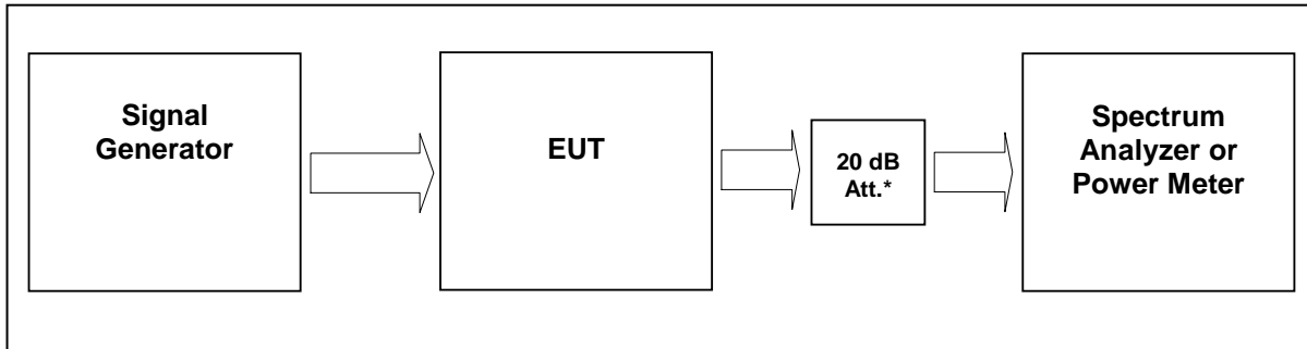
figure 6.4-#1 Test setup: Transmitter Output Power: IC RSS-133, RSS-GEN
