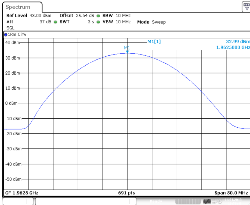
plot 4.3.1.5-#1 RF Power Out: §24.232, §2.1046; Test results; Downlink; W-CDMA Middle
