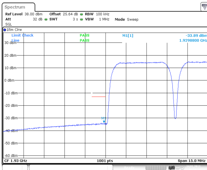
plot 6.3.1.5-#1 Spurious Emissions at Antenna Terminals: §24.238, §2.1051; Test results; Downlink; W-CDMA < 1MHz to band edge Lower Band Edge
