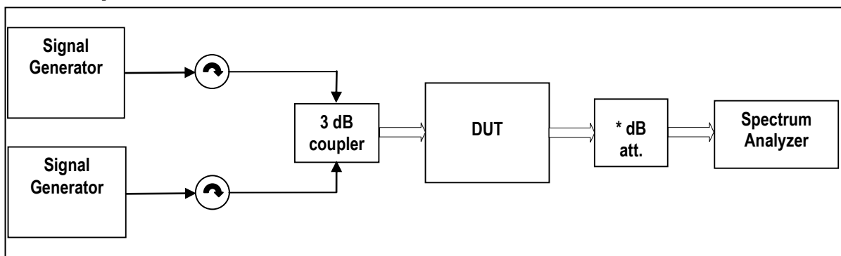
Multisignal-Generator used, External Attenuator DL x dB = 20 dB figure 6-#1 Test setup: Spurious Emissions at Antenna Terminals: §24.238, §2.1051
