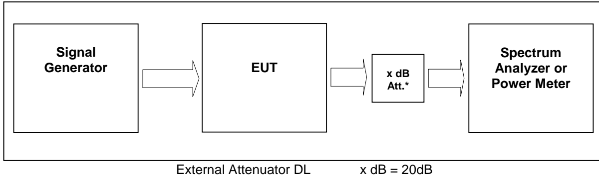
figure 2.4-#1 Test setup: RF Power Out: §24.232, §2.1046
