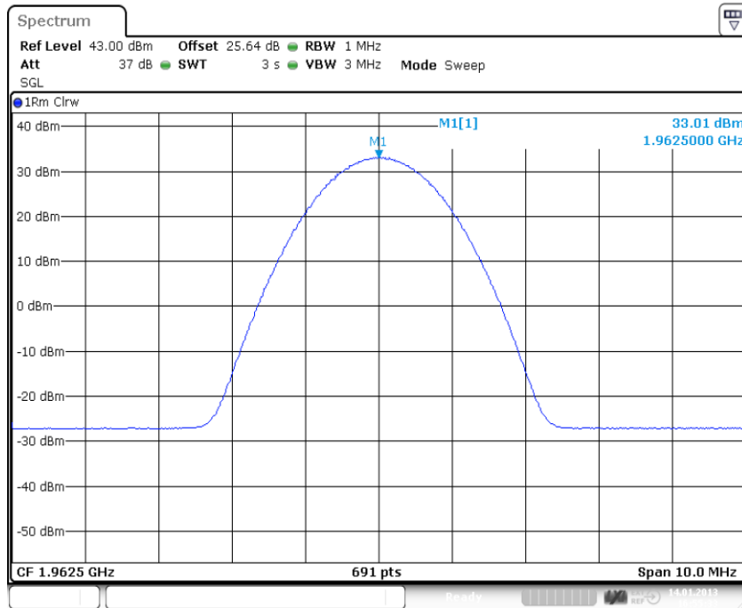
plot 4.3.1.3-#1 RF Power Out: §24.232, §2.1046; Test results; Downlink; EDGE Middle
