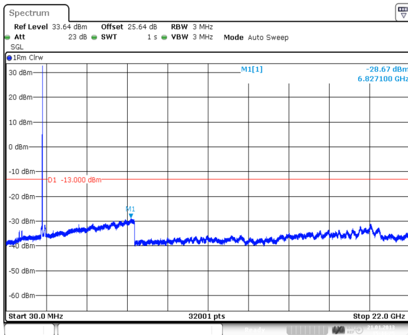
plot 6.3.1.7-#2 Spurious Emissions at Antenna Terminals: §24.238, §2.1051; Test results; Downlink; Analog > 1MHz to band edge; Upper Band Edge
