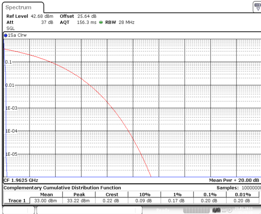
plot 7.3.1.1-#1 Transmitter Output Power: IC RSS-133, RSS-GEN; Test results; Downlink; Analog Middle Peak – to - average
