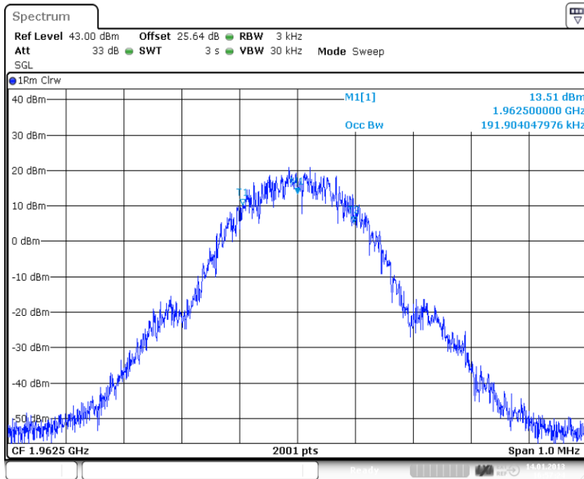
plot 5.3.1.2-#1 Occupied Bandwidth: $2.1049; Test results; Downlink; GSM Output
