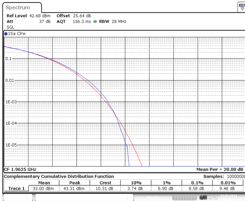
plot 7.3.1.5-#1 Transmitter Output Power: IC RSS-133, RSS-GEN; Test results; Downlink; W-CDMA Middle Peak – to – average
