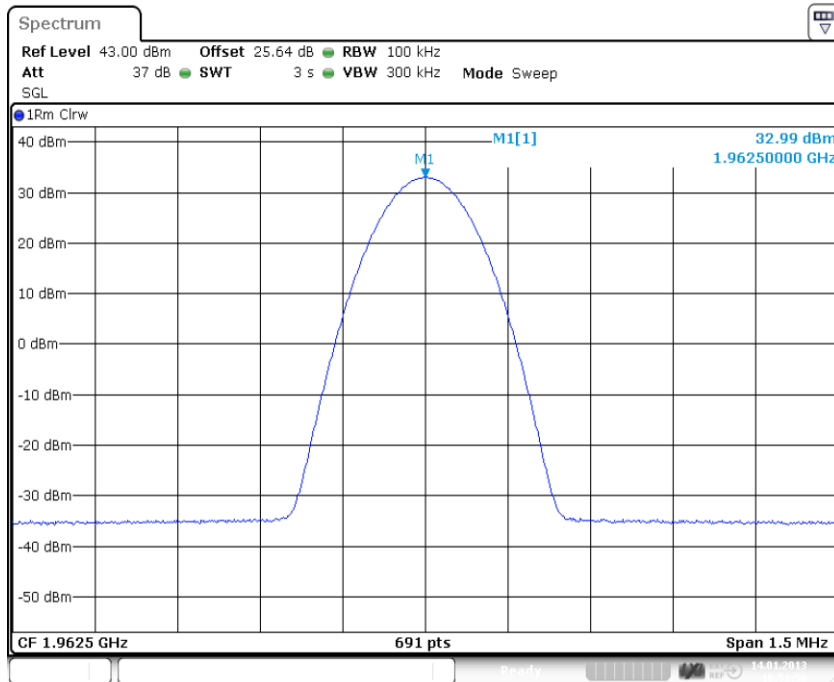
plot 4.3.1.1-#1 RF Power Out: §24.232, §2.1046; Test results; Downlink; Analog Middle
