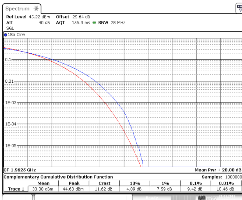
plot 7.3.1.4-#1 Transmitter Output Power: IC RSS-133, RSS-GEN; Test results; Downlink; CDMA Middle Peak – to - average
