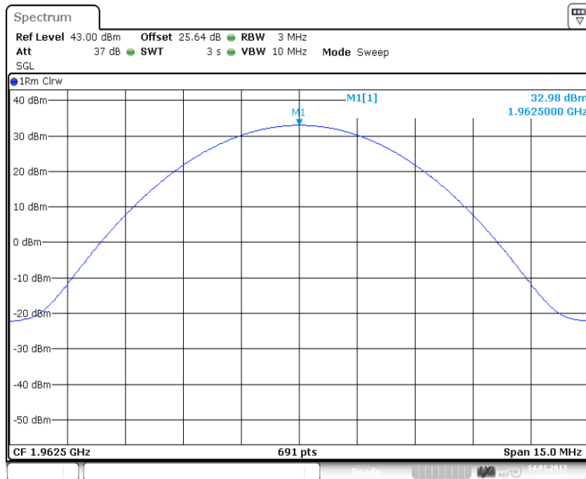
plot 4.3.1.4-#1 RF Power Out: §24.232, §2.1046; Test results; Downlink; CDMA Middle
