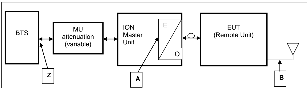
figure 1.1.4-#1 Block diagram of measurement reference points
