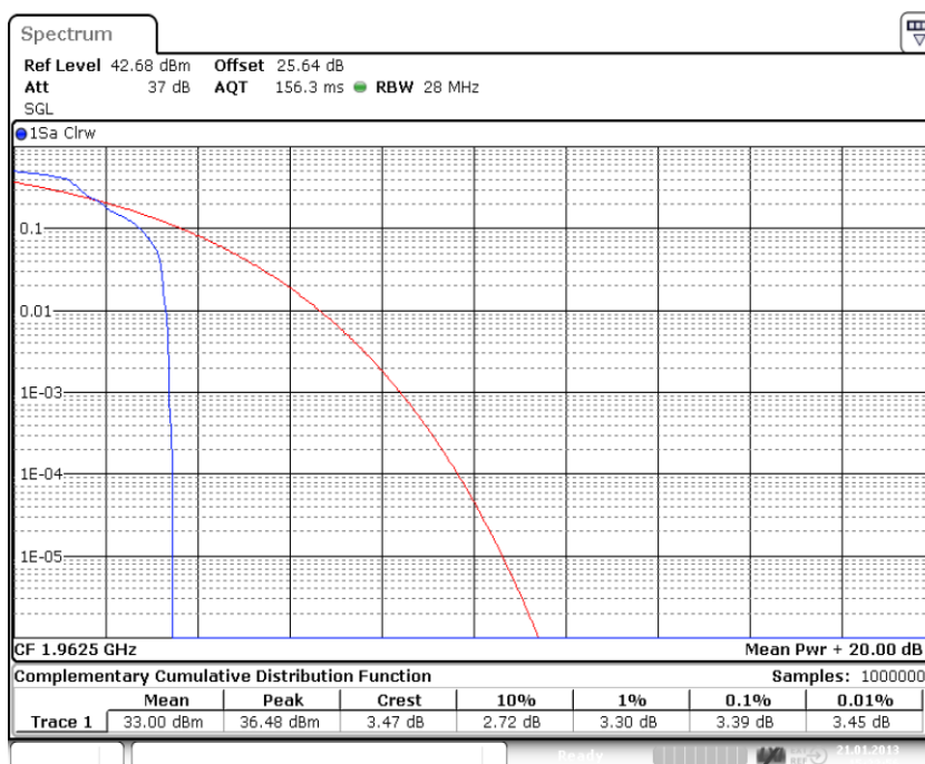
plot 7.3.1.3-#1 Transmitter Output Power: IC RSS-133, RSS-GEN; Test results; Downlink; EDGE Middle Peak – to - average
