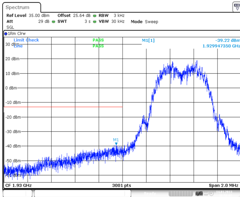
plot 6.3.1.2-#1 Spurious Emissions at Antenna Terminals: §24.238, §2.1051; Test results; Downlink; GSM < 1MHz to band edge Lower Band Edge
