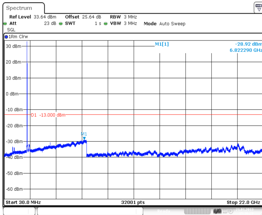
plot 6.3.1.8-#1 Spurious Emissions at Antenna Terminals: §24.238, §2.1051; Test results; Downlink; GSM > 1MHz to band edge; Lower Band Edge
