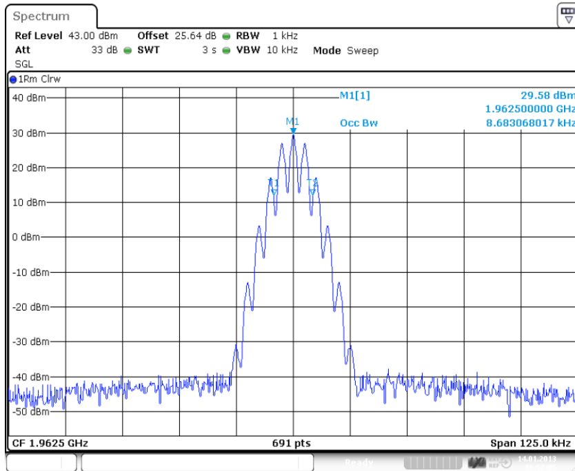
plot 5.3.1.1-#1 Occupied Bandwidth: §2.1049; Test results; Downlink; Analog Output
