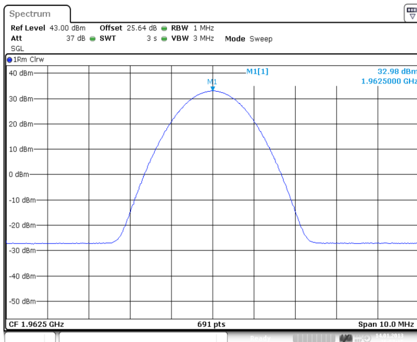
plot 4.3.1.2-#1 RF Power Out: §24.232, §2.1046; Test results; Downlink; GSM Middle
