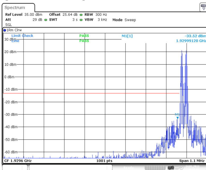
plot 6.3.1.1-#1 Spurious Emissions at Antenna Terminals: §24.238, §2.1051; Test results; Downlink; Analog < 1MHz to band edge Lower Band Edge
