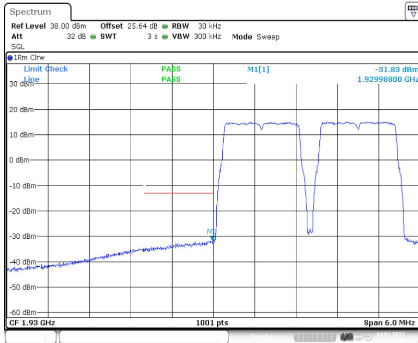
plot 6.3.1.6-#1 Spurious Emissions at Antenna Terminals: §24.238, §2.1051; Test results; Downlink; LTE < 1MHz to band edge Lower Band Edge
