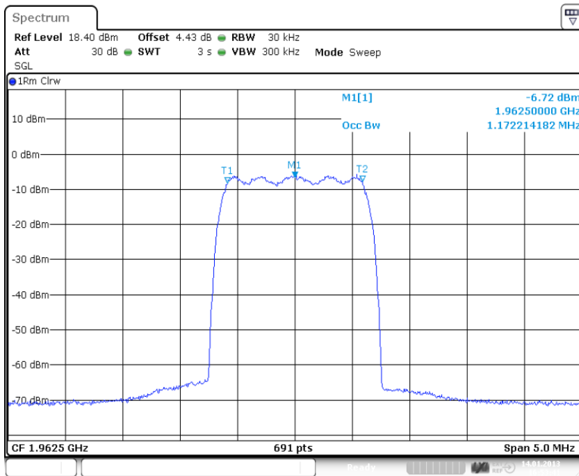
plot 5.3.1.4-#1 Occupied Bandwidth: $2.1049; Test results; Downlink; CDMA Output
