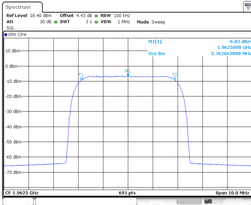
plot 5.3.1.5-#2 Occupied Bandwidth: §2.1049; Test results; Downlink; W-CDMA Input
