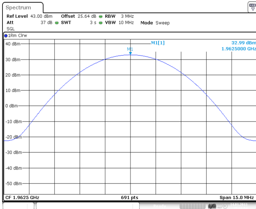
plot 4.3.1.6-#1 RF Power Out: §24.232, §2.1046; Test results; Downlink; LTE Middle
