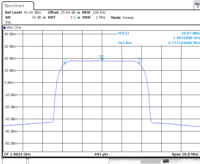
plot 5.3.1.5-#1 Occupied Bandwidth: §2.1049; Test results; Downlink; W-CDMA Output
