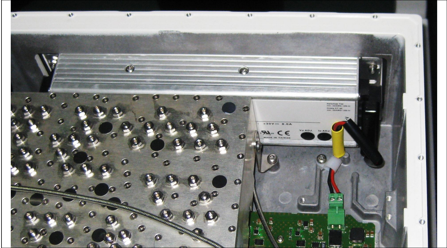
Power Supply
