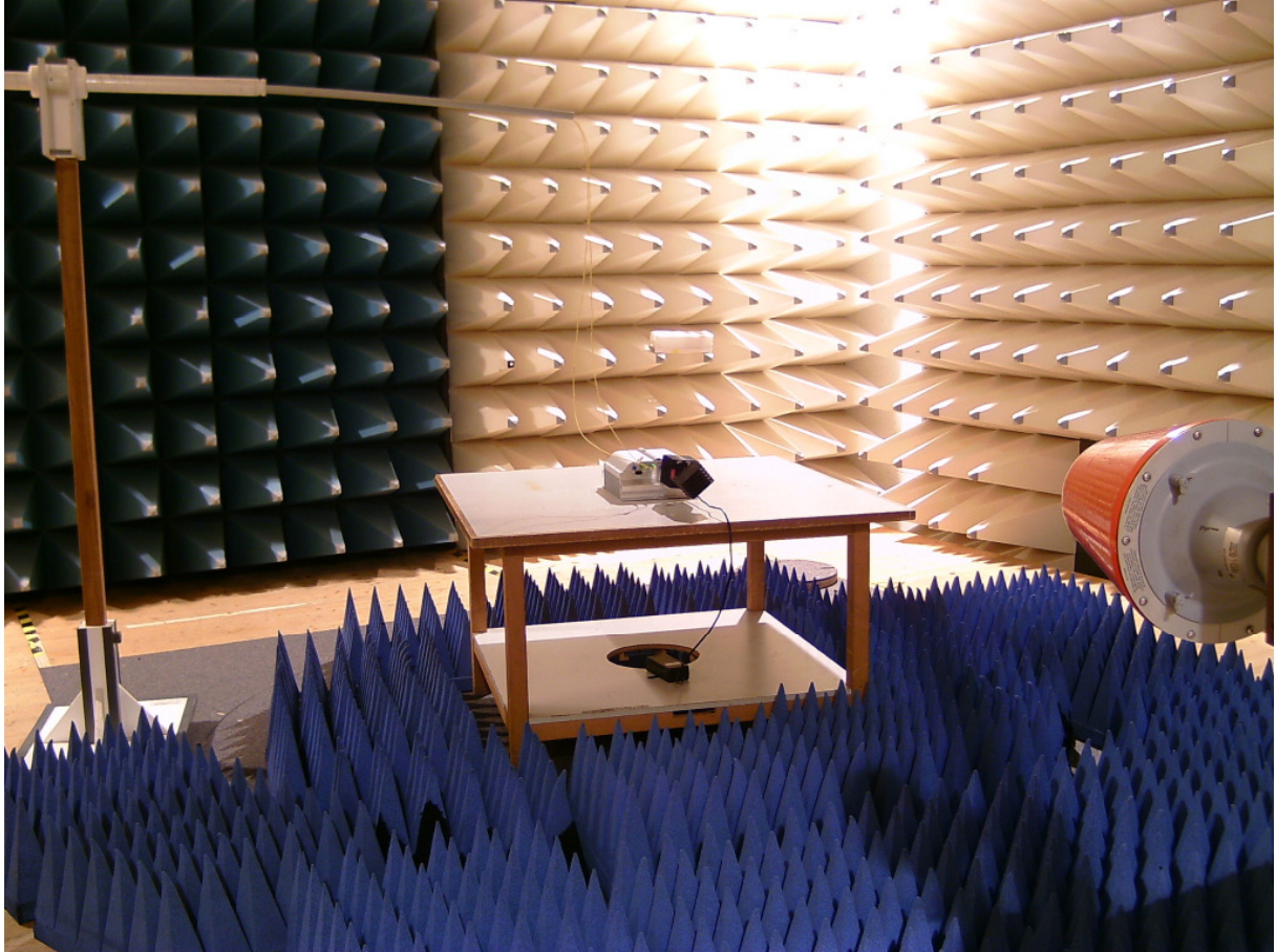
Radiated spurious emission 1GHz to 9GHz @3m in the Fully anechoic chamber .
