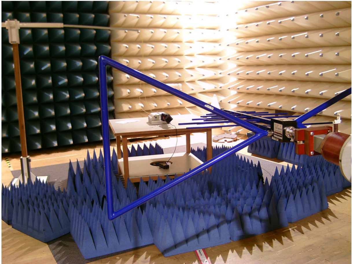
Radiated spurious emission 30MHz to 1GHz @3m in the Fully anechoic chamber
