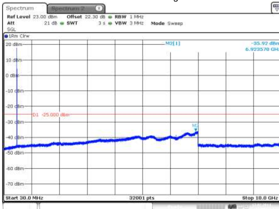
plot 7.3.1.4-#1 Spurious Emissions at Antenna Terminals: §90.210, §2.1051; Test results; Downlink; Band # 4; APCO Phase1 C4FM > 1MHz to band edge;
