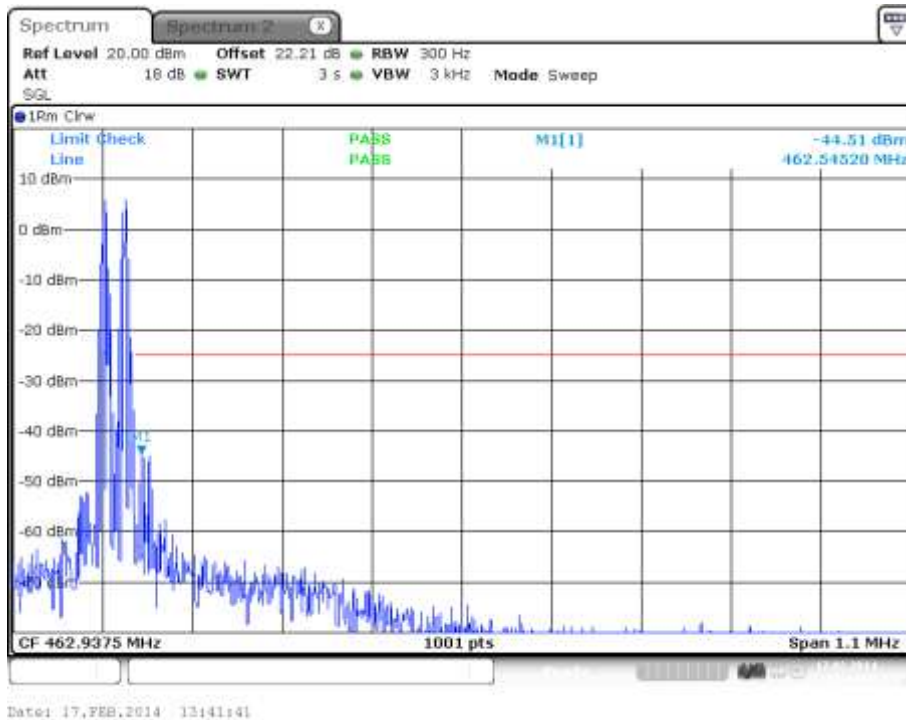
plot 8.3.1.2-#2 Intermodulation: §90.210, §2.1051; Test results; Downlink; Band # 2; Analog < 1MHz to band edge; Upper Band Edge
