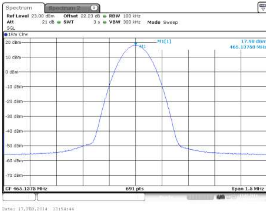
plot 5.3.1.3-#1 RF Power Out: §90.219, §2.1046; Test Results; Downlink; Band # 3; APCO Phase2 H-DQPSK
