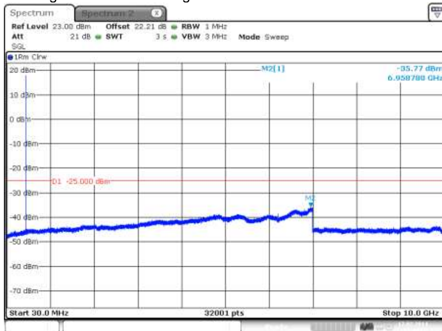
plot 7.3.1.2-#1 Spurious Emissions at Antenna Terminals: §90.210, §2.1051; Test results; Downlink; Band # 2; Analog > 1MHz to band edge;
