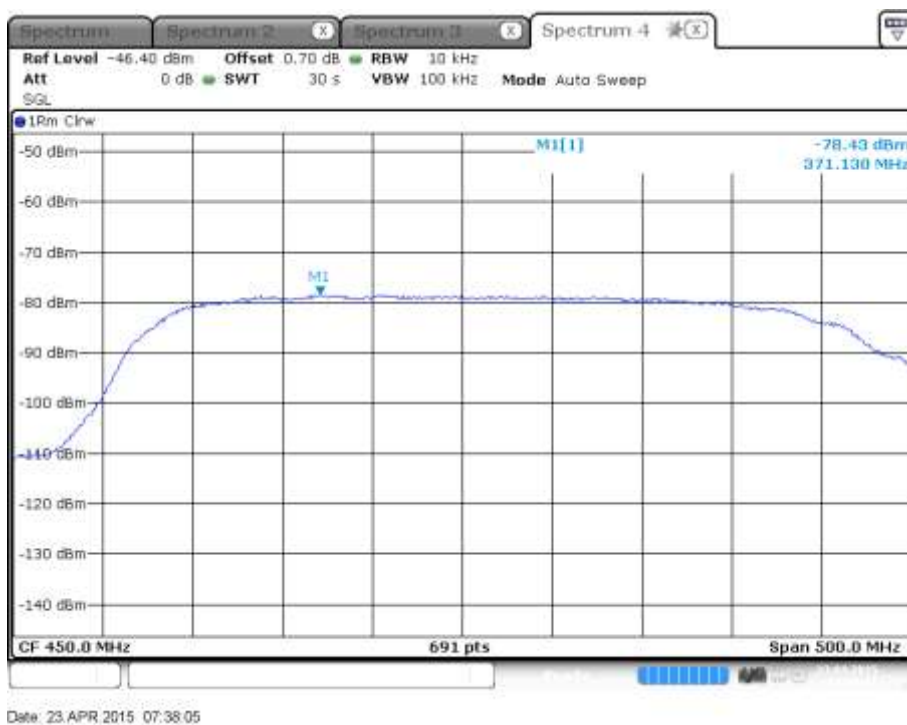
plot 9-#1 Noise
