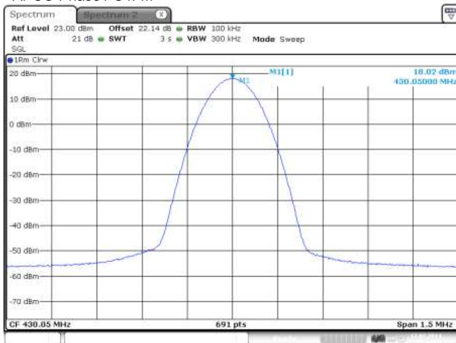
plot 5.3.1.1-#1 RF Power Out: §90.219, §2.1046; Test Results; Downlink; Band # 1; APCO Phase1 C4FM
