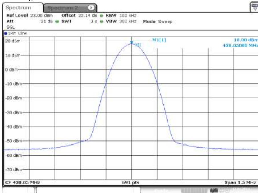
plot 5.3.1.1-#1 RF Power Out: §90.219, §2.1046; Test Results; Downlink; Band # 1; Analog
