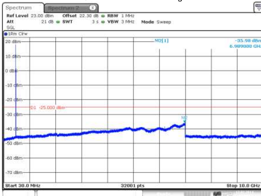
plot 7.3.1.4-#1 Spurious Emissions at Antenna Terminals: §90.210, §2.1051; Test results; Downlink; Band # 4; APCO Phase2 H-DQPSK > 1MHz to band edge;
