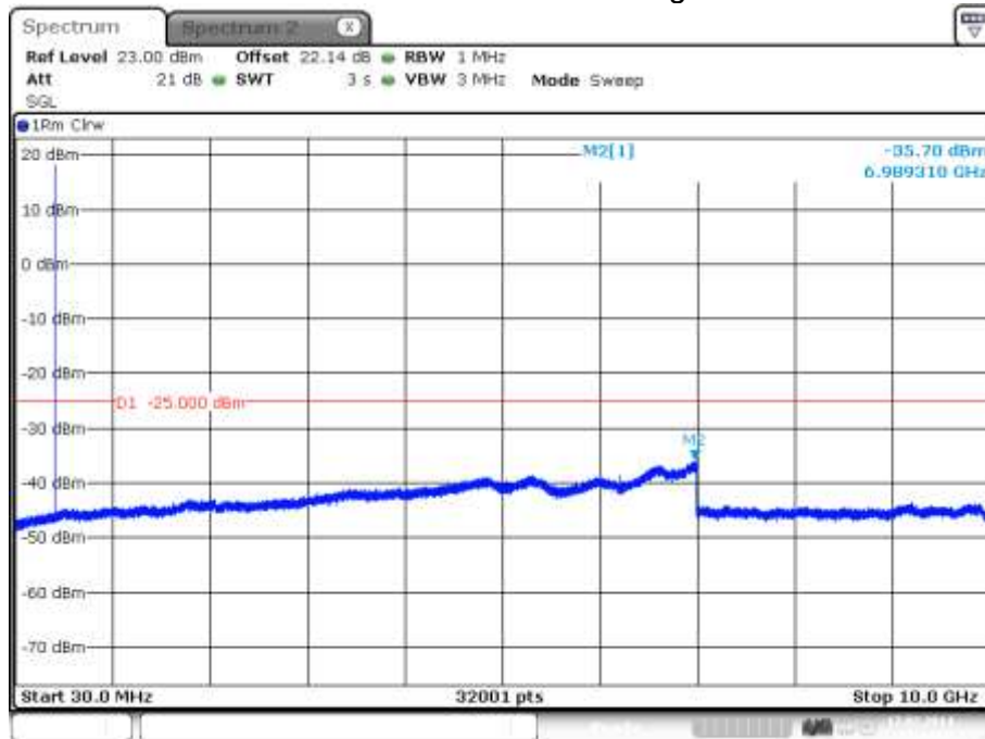
plot 7.3.1.1-#1 Spurious Emissions at Antenna Terminals: §90.210, §2.1051; Test results; Downlink; Band # 1; APCO Phase2 H-DQPSK > 1MHz to band edge;
