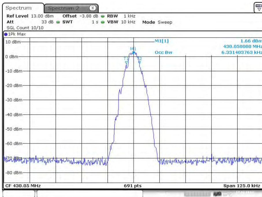
plot 6.3.1.1-#2 Occupied Bandwidth: §90.210, §2.1049; Test results; Downlink; Band # 1; APCO Phase1 C4FM; Input
