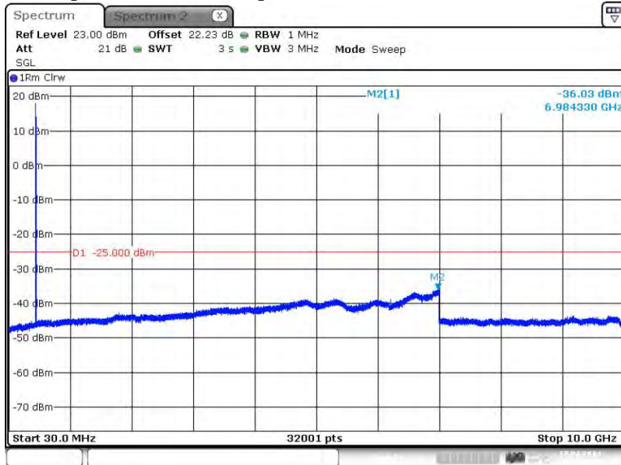
plot 7.3.1.7-#1 Spurious Emissions at Antenna Terminals: §90.210, §2.1051; Test results; Downlink; Band # 3; Analog > 1MHz to band edge;
