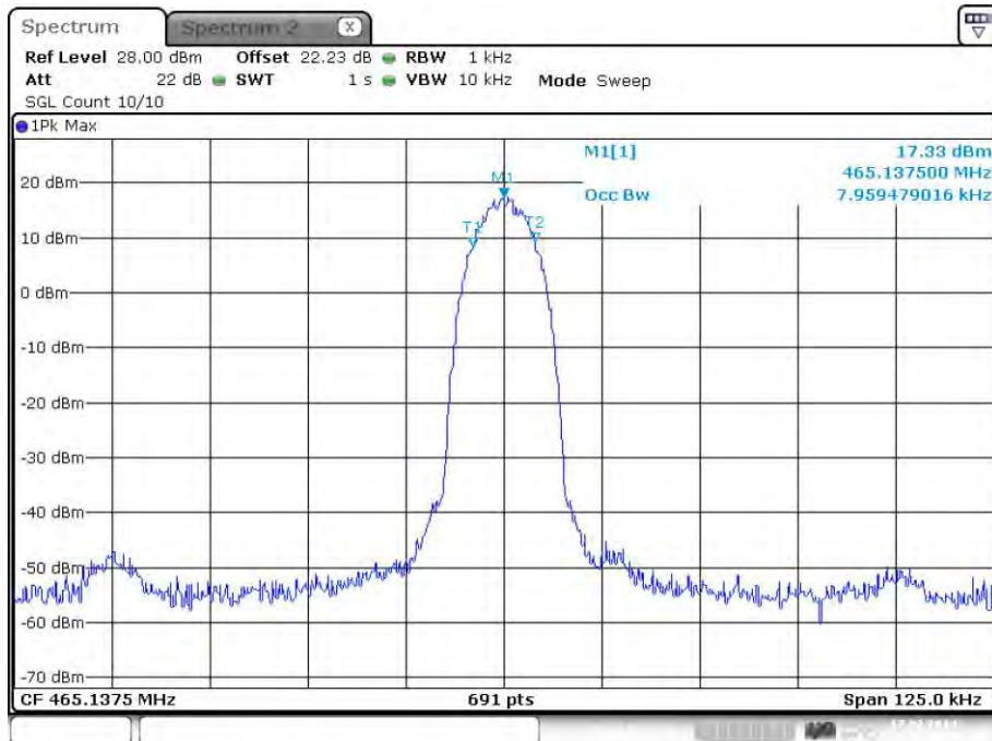
plot 6.3.1.3-#1 Occupied Bandwidth: §90.210, §2.1049; Test results; Downlink; Band # 3; APCO Phase2 H-DQPSK; Output
