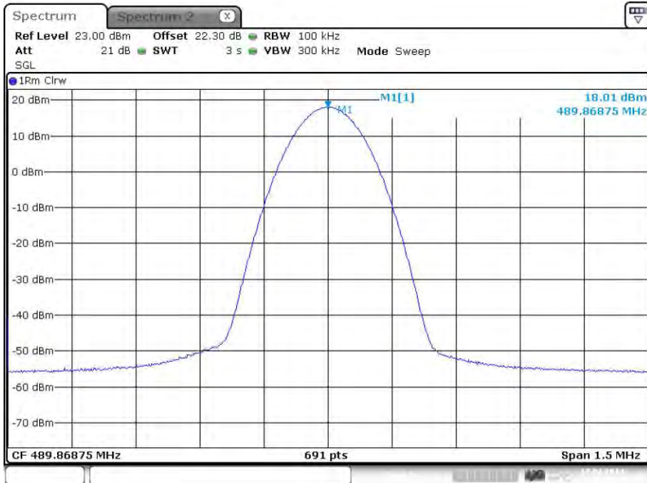
plot 5.3.1.4-#1 RF Power Out: §90.635, §2.1046; Test Results; Downlink; Band # 4; APCO Phase2 H-DQPSK
