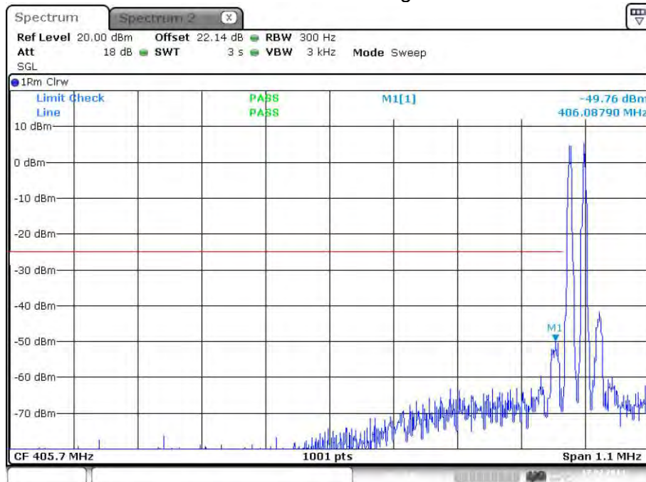
plot 7.3.1.1-#1 Spurious Emissions at Antenna Terminals: §90.210, §2.1051; Test results; Downlink; Band # 1; APCO Phase1 C4FM < 1MHz to band edge; Lower Band Edge
