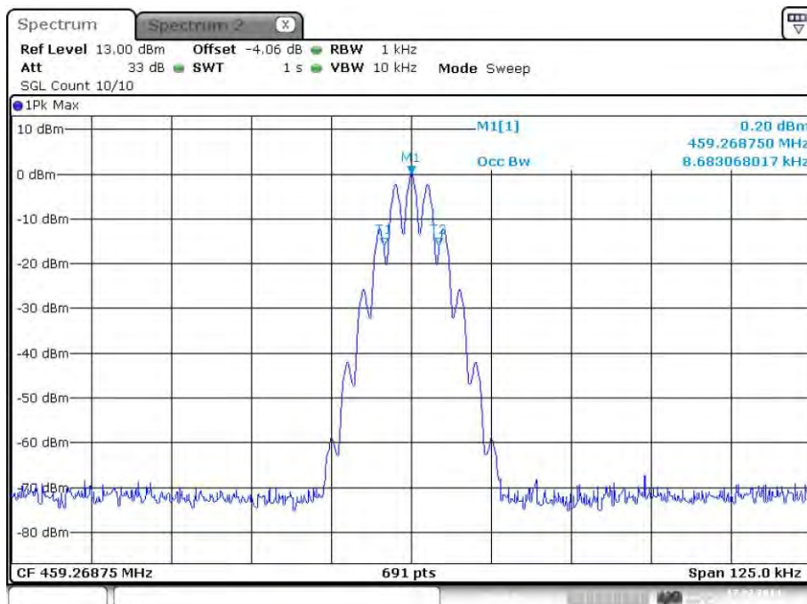
plot 6.3.1.2-#1 Occupied Bandwidth: §90.210, §2.1049; Test results; Downlink; Band # 2; Analog; Output
