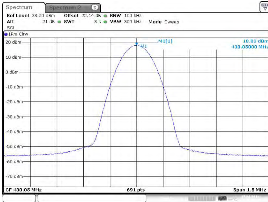
plot 5.3.1.1-#1 RF Power Out: §90.635, §2.1046; Test Results; Downlink; Band # 1; APCO Phase2 H-DQPSK
