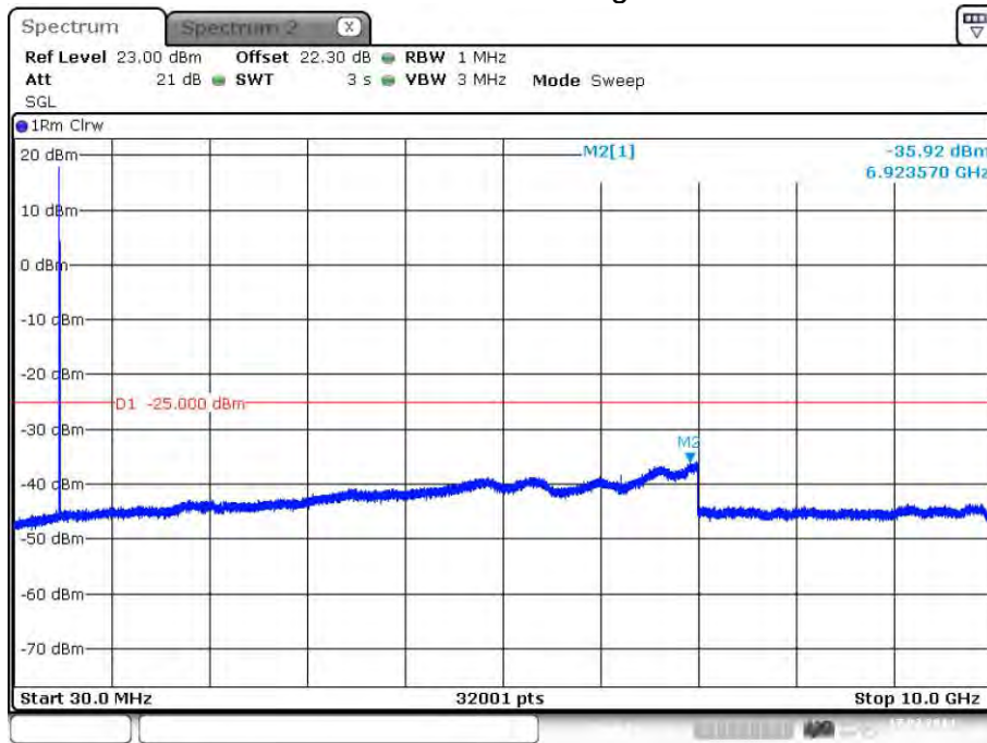
plot 7.3.1.8-#1 Spurious Emissions at Antenna Terminals: §90.210, §2.1051; Test results; Downlink; Band # 4; APCO Phase1 C4FM > 1MHz to band edge;
