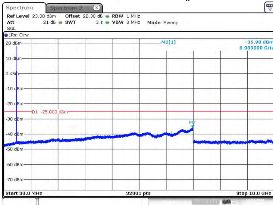
plot 7.3.1.8-#1 Spurious Emissions at Antenna Terminals: §90.210, §2.1051; Test results; Downlink; Band # 4; APCO Phase2 H-DQPSK > 1MHz to band edge;
