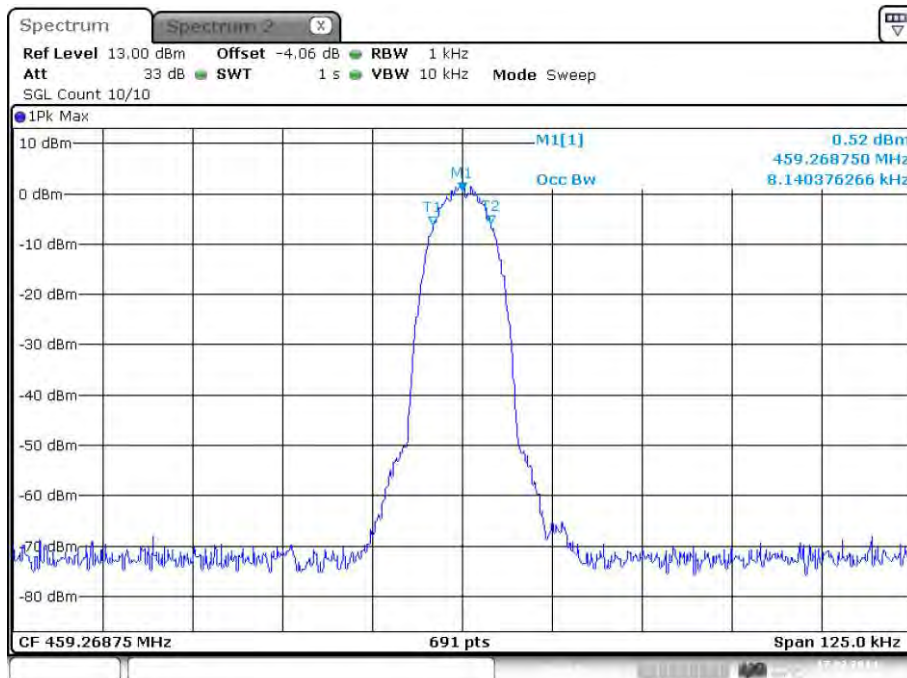
plot 6.3.1.2-#1 Occupied Bandwidth: §90.210, §2.1049; Test results; Downlink; Band # 2; APCO Phase2 H-DQPSK; Output
