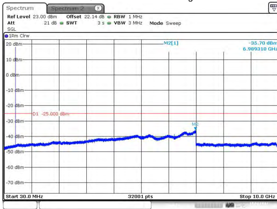
plot 7.3.1.5-#1 Spurious Emissions at Antenna Terminals: §90.210, §2.1051; Test results; Downlink; Band # 1; APCO Phase2 H-DQPSK > 1MHz to band edge;
