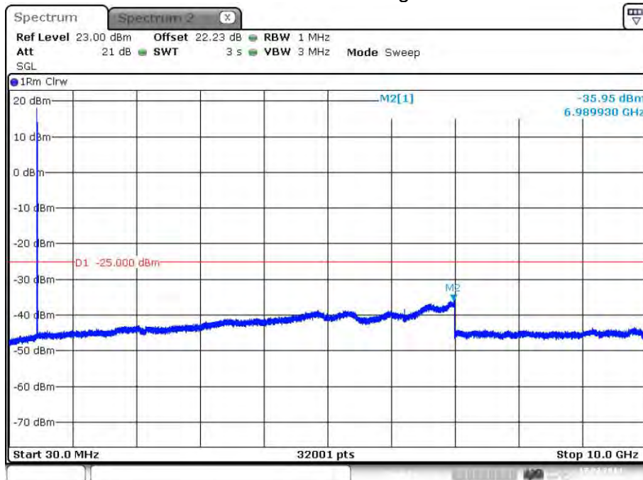
plot 7.3.1.7-#1 Spurious Emissions at Antenna Terminals: §90.210, §2.1051; Test results; Downlink; Band # 3; APCO Phase1 C4FM > 1MHz to band edge;
