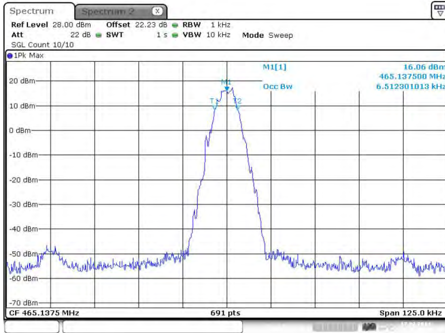
plot 6.3.1.3-#1 Occupied Bandwidth: §90.210, §2.1049; Test results; Downlink; Band # 3; APCO Phase1 C4FM; Output
