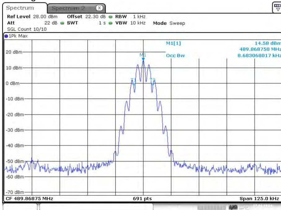
plot 6.3.1.4-#1 Occupied Bandwidth: §90.210, §2.1049; Test results; Downlink; Band # 4; Analog; Output
