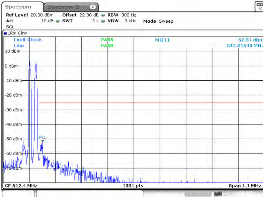
plot 7.3.1.4-#2 Spurious Emissions at Antenna Terminals: §90.210, §2.1051; Test results; Downlink; Band # 4; APCO Phase2 H-DQPSK < 1MHz to band edge; Upper Band Edge
