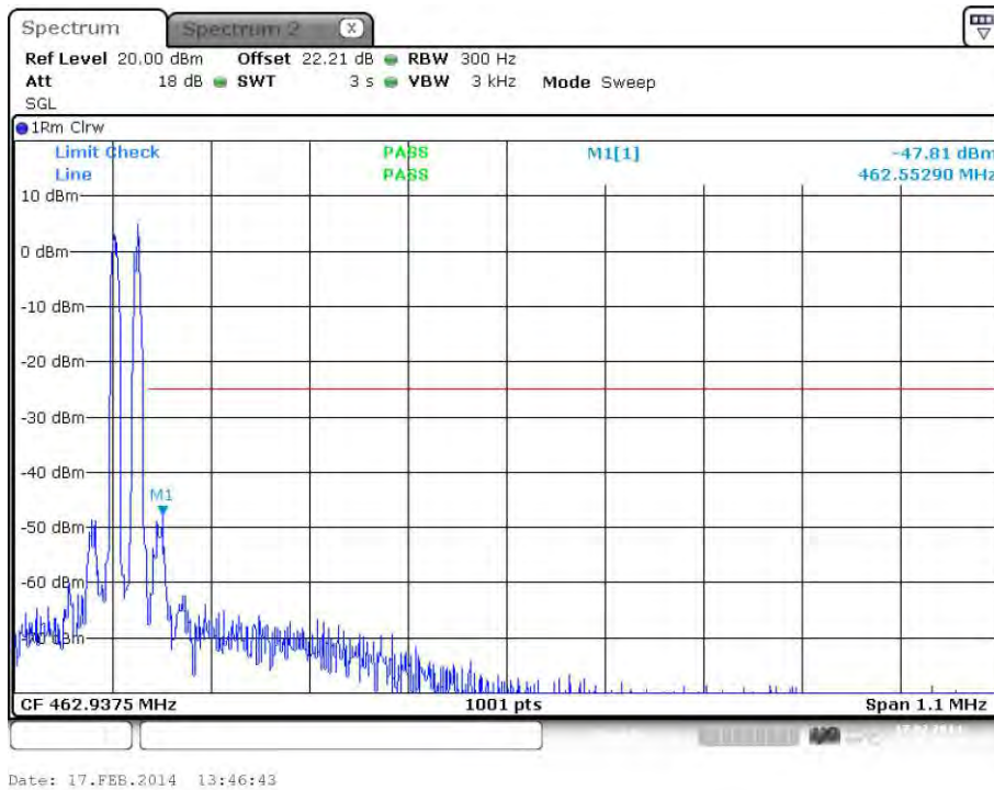
plot 7.3.1.2-#2 Spurious Emissions at Antenna Terminals: §90.210, §2.1051; Test results; Downlink; Band # 2; APCO Phase2 H-DQPSK < 1MHz to band edge; Upper Band Edge
