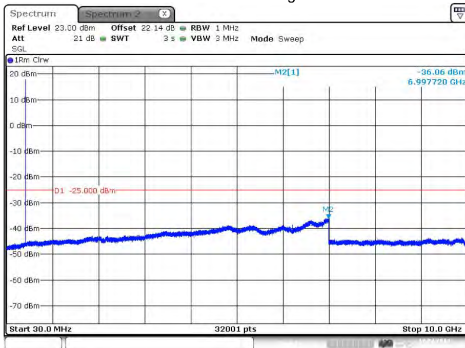
plot 7.3.1.5-#1 Spurious Emissions at Antenna Terminals: §90.210, §2.1051; Test results; Downlink; Band # 1; APCO Phase1 C4FM > 1MHz to band edge;
