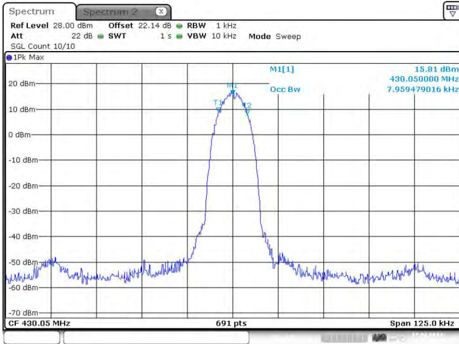
plot 6.3.1.1-#1 Occupied Bandwidth: §90.210, §2.1049; Test results; Downlink; Band # 1; APCO Phase2 H-DQPSK; Output
