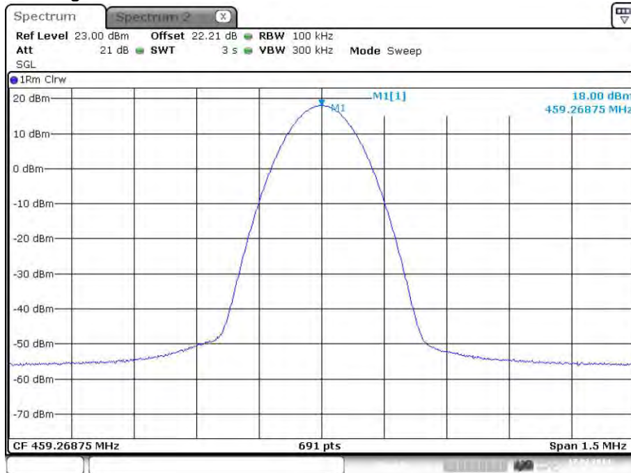
plot 5.3.1.2-#1 RF Power Out: §90.635, §2.1046; Test Results; Downlink; Band # 2; Analog
