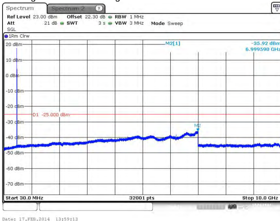
plot 7.3.1.8-#1 Spurious Emissions at Antenna Terminals: §90.210, §2.1051; Test results; Downlink; Band # 4; Analog > 1MHz to band edge;
