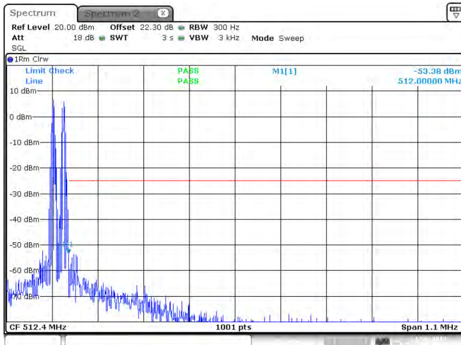
plot 7.3.1.4-#1 Spurious Emissions at Antenna Terminals: §90.210, §2.1051; Test results; Downlink; Band # 4; Analog < 1MHz to band edge; Lower Band Edge
