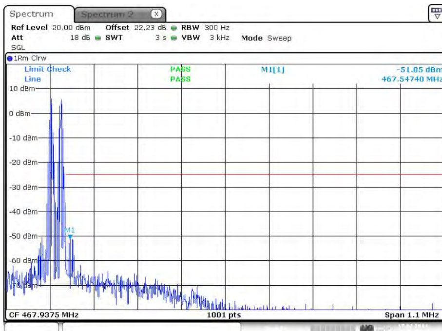
plot 7.3.1.3-#1 Spurious Emissions at Antenna Terminals: §90.210, §2.1051; Test results; Downlink; Band # 3; Analog < 1MHz to band edge; Lower Band Edge
