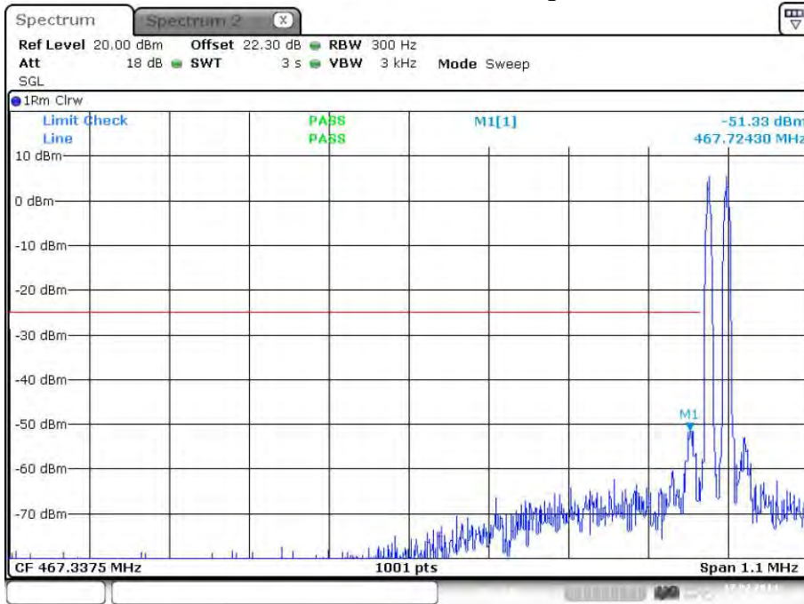
plot 7.3.1.4-#1 Spurious Emissions at Antenna Terminals: §90.210, §2.1051; Test results; Downlink; Band # 4; APCO Phase2 H-DQPSK < 1MHz to band edge; Lower Band Edge
