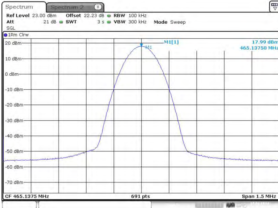
plot 5.3.1.3-#1 RF Power Out: §90.635, §2.1046; Test Results; Downlink; Band # 3; APCO Phase1 C4FM
