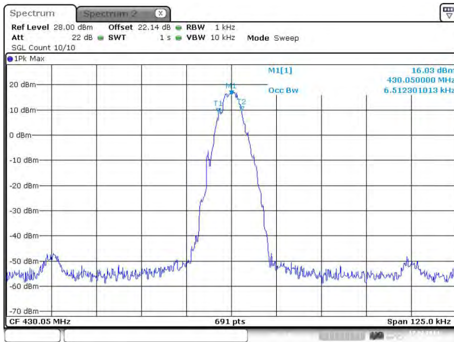
plot 6.3.1.1-#1 Occupied Bandwidth: §90.210, §2.1049; Test results; Downlink; Band # 1; APCO Phase1 C4FM; Output
