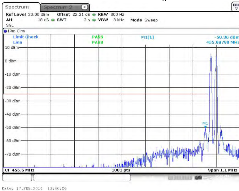
plot 7.3.1.2-#1 Spurious Emissions at Antenna Terminals: §90.210, §2.1051; Test results; Downlink; Band # 2; APCO Phase2 H-DQPSK < 1MHz to band edge; Lower Band Edge
