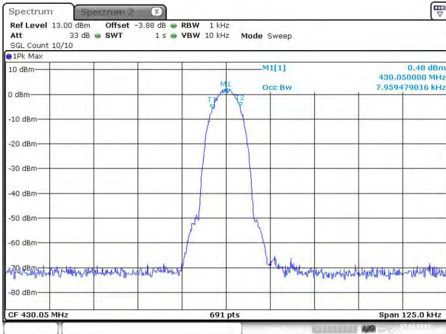
plot 6.3.1.1-#2 Occupied Bandwidth: §90.210, §2.1049; Test results; Downlink; Band # 1; APCO Phase2 H-DQPSK; Input
