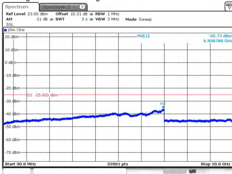
plot 7.3.1.6-#1 Spurious Emissions at Antenna Terminals: §90.210, §2.1051; Test results; Downlink; Band # 2; Analog > 1MHz to band edge;
