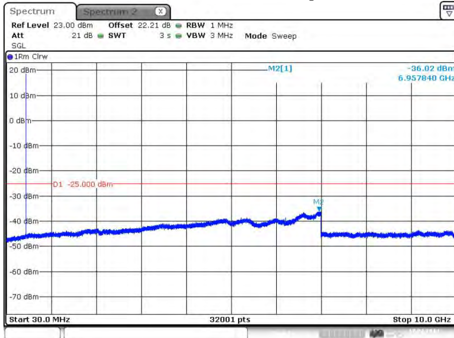
plot 7.3.1.6-#1 Spurious Emissions at Antenna Terminals: §90.210, §2.1051; Test results; Downlink; Band # 2; APCO Phase2 H-DQPSK > 1MHz to band edge;
