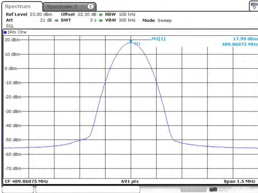
plot 5.3.1.4-#1 RF Power Out: §90.635, §2.1046; Test Results; Downlink; Band # 4; APCO Phase1 C4FM
