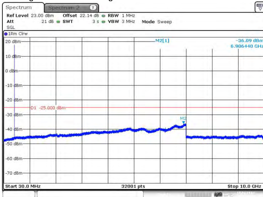
plot 7.3.1.5-#1 Spurious Emissions at Antenna Terminals: §90.210, §2.1051; Test results; Downlink; Band # 1; Analog > 1MHz to band edge;
