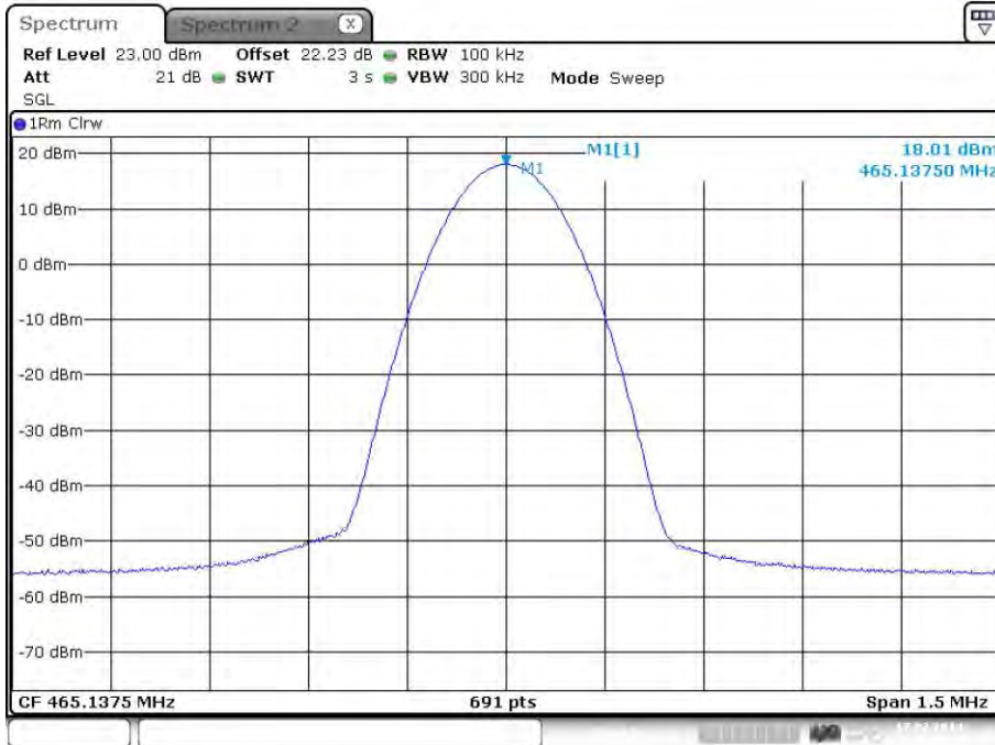
plot 5.3.1.3-#1 RF Power Out: §90.635, §2.1046; Test Results; Downlink; Band # 3; Analog
