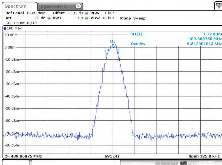
plot 6.3.1.4-#1 Occupied Bandwidth: §90.210, §2.1049; Test results; Downlink; Band # 4; APCO Phase1 C4FM; Output
