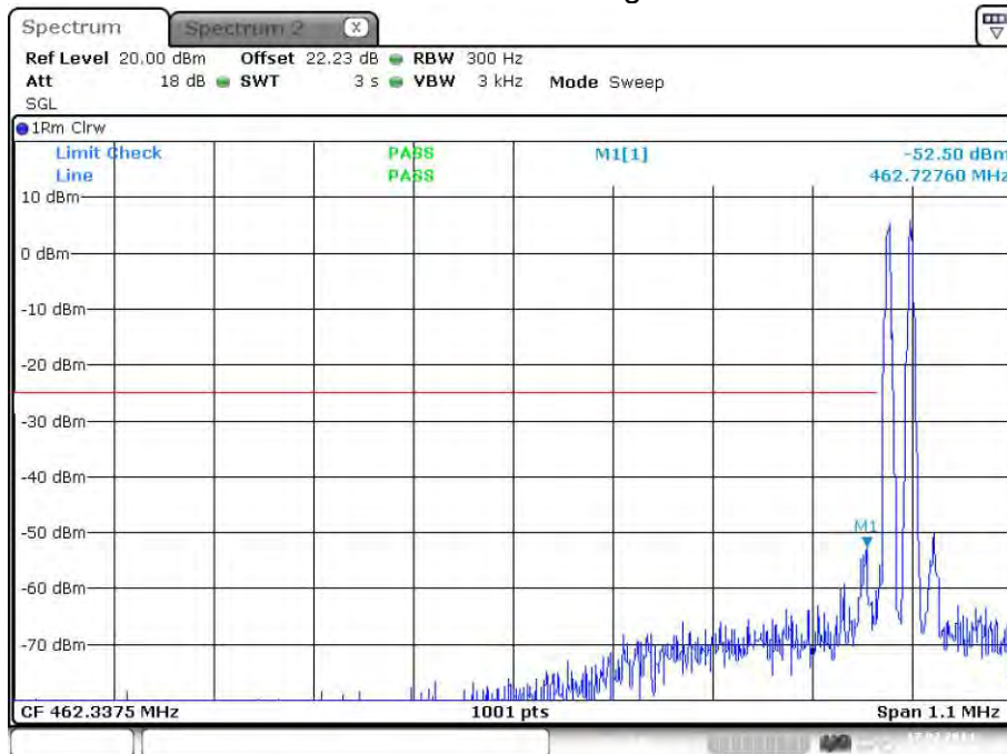
plot 7.3.1.3-#1 Spurious Emissions at Antenna Terminals: §90.210, §2.1051; Test results; Downlink; Band # 3; APCO Phase1 C4FM < 1MHz to band edge; Lower Band Edge
