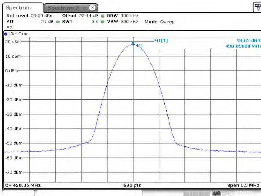
plot 5.3.1.1-#1 RF Power Out: §90.635, §2.1046; Test Results; Downlink; Band # 1; APCO Phase1 C4FM
