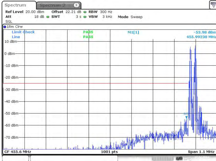
plot 7.3.1.2-#1 Spurious Emissions at Antenna Terminals: §90.210, §2.1051; Test results; Downlink; Band # 2; Analog < 1MHz to band edge; Lower Band Edge
