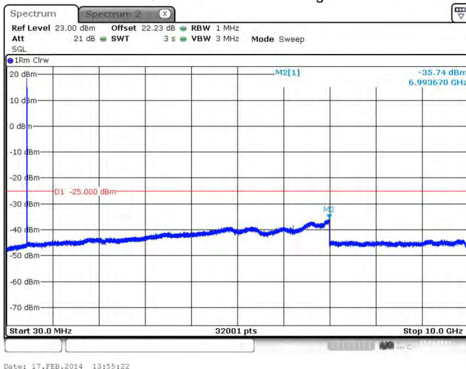
plot 7.3.1.7-#1 Spurious Emissions at Antenna Terminals: §90.210, §2.1051; Test results; Downlink; Band # 3; APCO Phase2 H-DQPSK > 1MHz to band edge;
