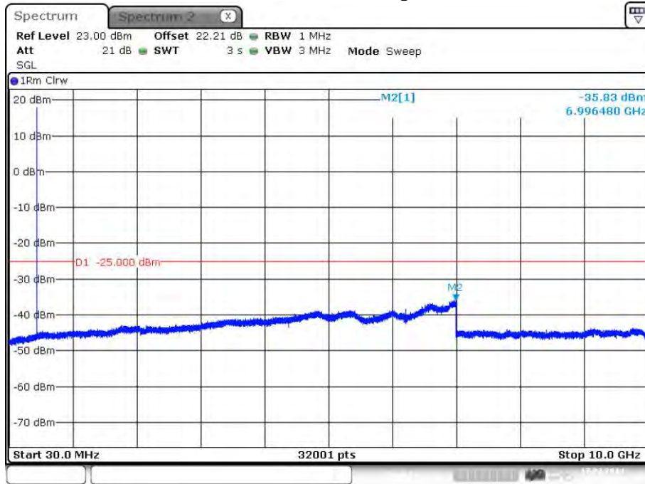
plot 7.3.1.6-#1 Spurious Emissions at Antenna Terminals: §90.210, §2.1051; Test results; Downlink; Band # 2; APCO Phase1 C4FM > 1MHz to band edge;
