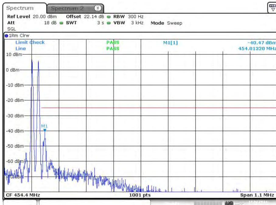
plot 7.3.1.1-#2 Spurious Emissions at Antenna Terminals: §90.210, §2.1051; Test results; Downlink; Band # 1; APCO Phase1 C4FM < 1MHz to band edge; Upper Band Edge
