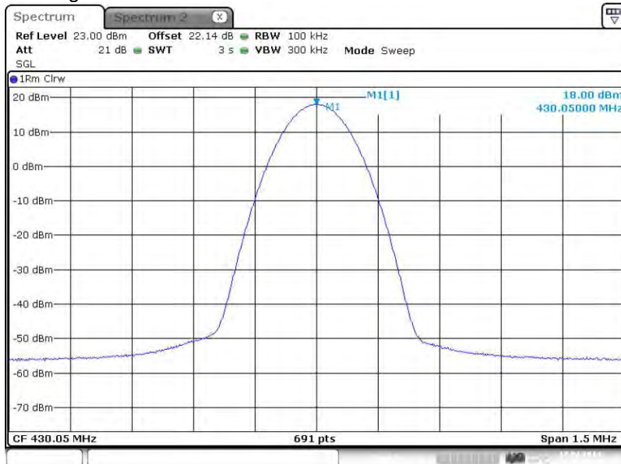
plot 5.3.1.1-#1 RF Power Out: §90.635, §2.1046; Test Results; Downlink; Band # 1; Analog
