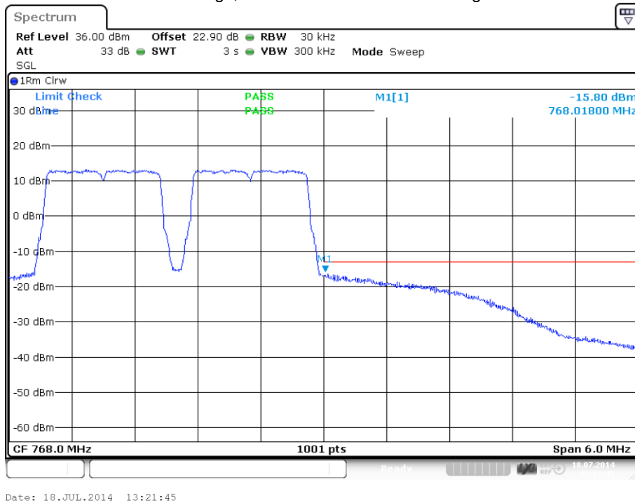
plot 7.3.1.1-#2 Spurious Emissions at Antenna Terminals: §90.543, §2.1051; Test results; Downlink; LTE < 1MHz to band edge; 758 – 768MHz Upper Band Edge
